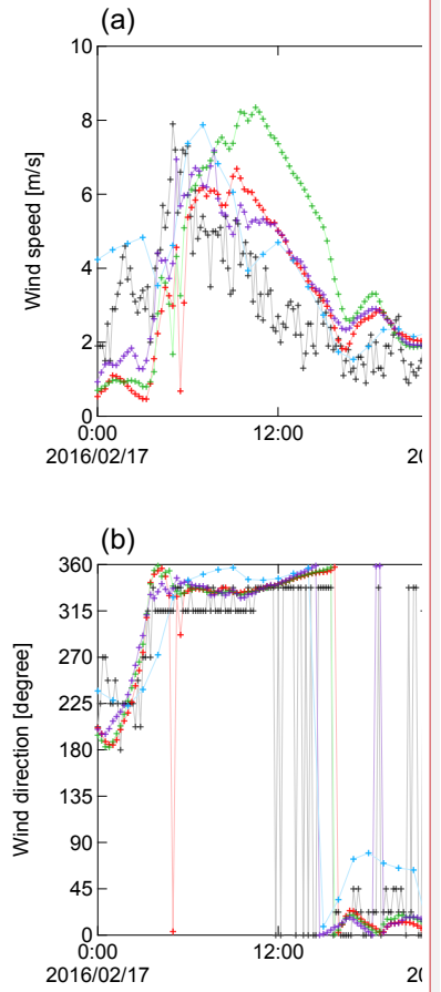
Figure 4. (a) Wind speed and (b) wind direction at the Tokyo AMeDAS station. The model data from the WRF simulations using different PBL schemes and the ERA5 reanalysis are also shown.
