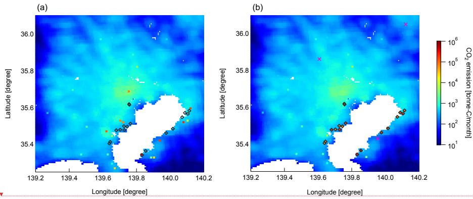
Figure 3. Anthropogenic CO 2 emissions from the TMA in March 2016 in (a) the original ODIAC 2020b data and (b) the same data except that the locations and emission magnitudes of large point sources, such as power plants and manufacturing plants, were corrected based on the national emission inventory. Open diamonds denote the locations of large point sources, and the crosses in (b) denote the observation sites.
