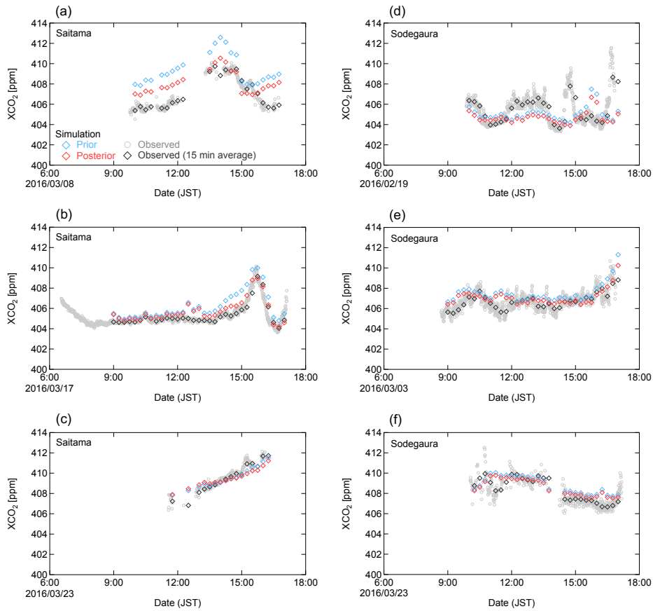
525 Figure 8. Comparison of the XCO 2 observations with the WRF–STILT prior (blue) and posterior (red) simulation results for three representative days at (a–c) Saitama and (d–f) Sodegaura. The observations are presented as individual values (open circles) and as the 15-min averaged values used for the inversion (open diamonds).
