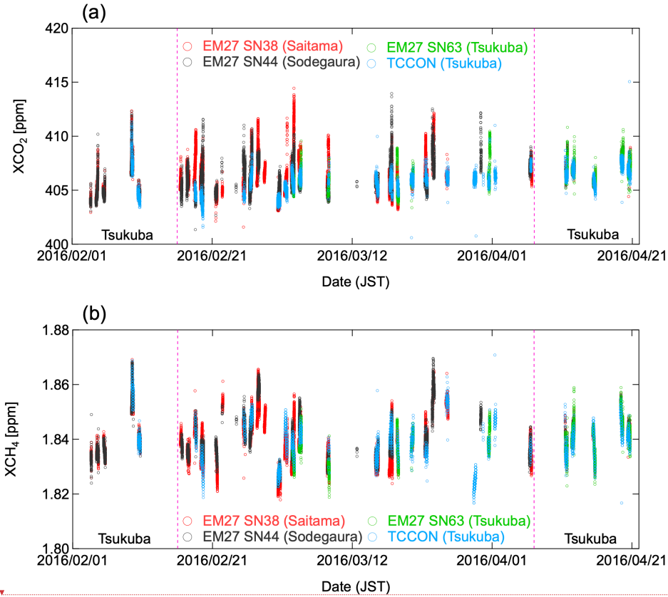
470 Figure 2. Time series of XCO 2 and XCH 4 during the observation campaign, including side-by-side measurements conducted at Tsukuba. The dashed vertical lines show the dates when the field observations began and ended at the three sites.
