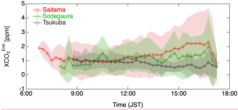
Figure 6. Average diurnal variations in XCO_2 differences ( XCO_2^{Enh} ) from daily background values. These background values were assumed to be common to the three sites and be the 5th percentile value of the Tsukuba TCCON measurements throughout each day. The average XCO_2^{Enh} values (open diamonds) and their standard deviations (shading) were calculated for 15-min bins using all data acquired during the campaign period.
