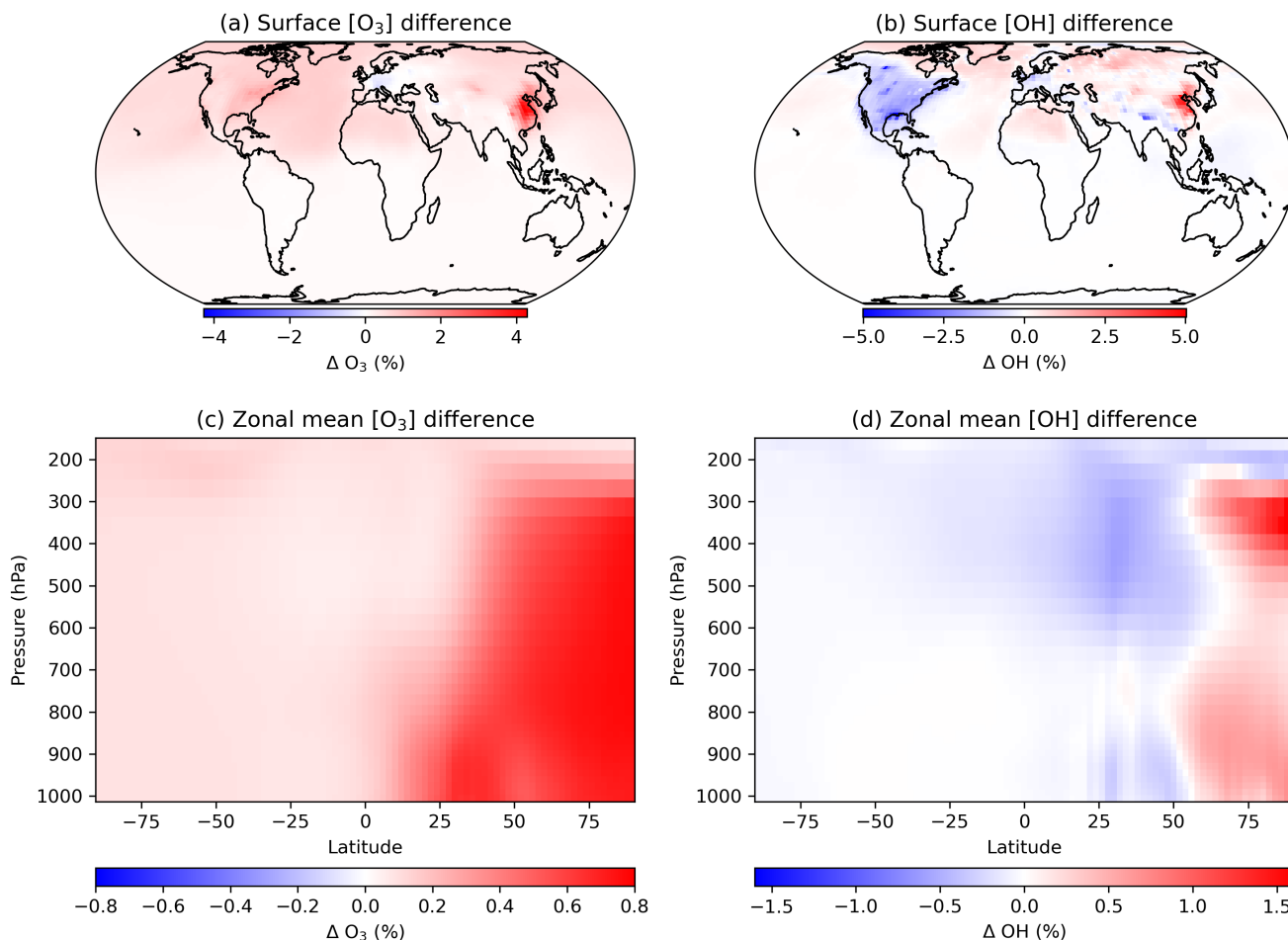
Figure 19. Top panels show the simulated percentage change in annual mean surface concentrations of \text{O}_3 (a) and \text{OH} (b). Lower panels show the annual mean percentage change through the troposphere for the same species.
