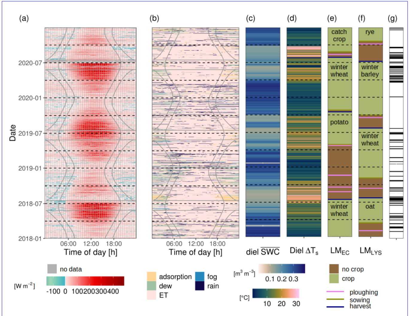
Figure 4. Diel and seasonal dynamics of (a) quality filtered latent heat fluxes from eddy covariance (EC) technique (b) classified dominant lysimeter (LYS) fluxes (exemplarily shown for Se_Y_{032} ) at the Selhausen agricultural field site. Solid vertical lines mark the end of the night, sunrise, sunset, and beginning of the night, respectively (determined by the geographic coordinates of the field site). Mean volumetric soil water content at 0.1 m depth \overline{SWC} and maximum diel difference in surface temperature ( \Delta T_s ) are displayed as diel measurements in panels (c) and (d). Land management (LM) is illustrated separately below the EC (e) and on the LYS (f). In panel (g) the dates selected for this comparison based on the absence of rain, fog, and dew are marked as horizontal black lines (see section 3.4).
