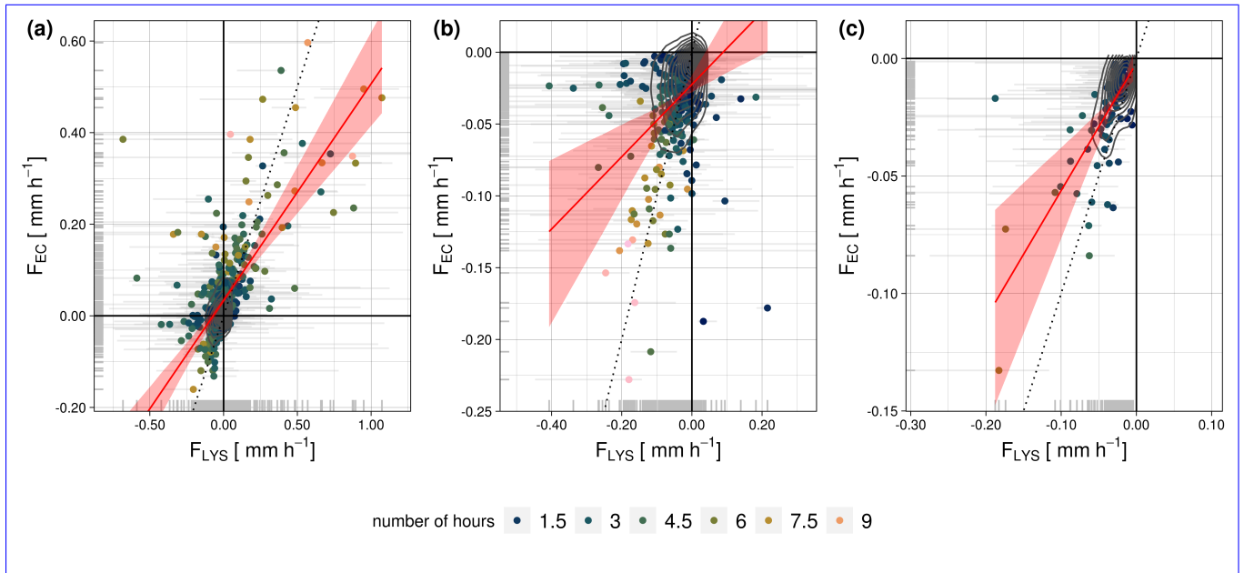
Figure 6. Comparison between night-time sums of lysimeter measured water fluxes ( F_{LYS} ) against eddy-covariance measured fluxes ( F_{EC} ) in Majadas de Tiétar (ES-LMa*, toprow) for different subsets of the data: (a) all good quality nighttime fluxes, (b) negative EC nighttime fluxes, and (c) negative nighttime fluxes and all lysimeter fluxes classified as soil adsorption of atmospheric water vapor. The red line illustrates a major axis regression model and the red shading the confidence interval of the model. The black dotted line illustrates identity. Horizontal grey lines illustrate the minimum and maximum sum observed from single lysimeter columns. The colorcode illustrates the number of hours over which this sum was formed. It depends on how many observations were measured for the respective conditions on each night.
