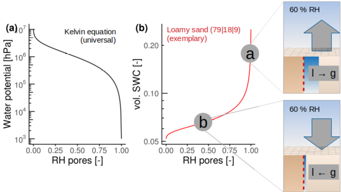
Figure 1. Relationship between (a) soil water potential and relative humidity (rH) of the soil pores at 20 degC defined with the Kelvin equation. (b) Illustration of the conversion of water potential from (a) to the respective volumetric soil water content (SWC, \text{m}^3 \text{m}^{-3} ) for a loamy sand consisting of 79 % sand, 18 % silt and 9 % clay , based on the van Genuchten Model [ van Genuchten , 1980]. The representations (a and b) illustrate that at constant atmospheric rH of 60 % at a temperature of 20 °C, the vapor flux direction and phase change ( l and g for liquid and gas ) within the soil are opposite for different soil water potentials.
