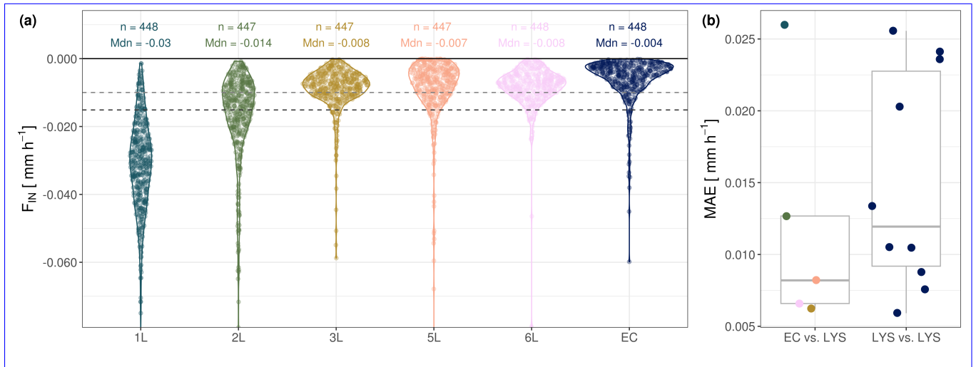
Figure 7. a) Distributions of half hourly readings shown individually for each lysimeter and the EC in Majadas de Tiétar. Only periods during which adsorption and negative latent heat flux were measured uniformly were selected. The horizontal dashed lines show the mean (black) and median (grey). b) Mean average error (MAE, mm) between individual lysimeter columns and EC (between techniques) and MAE between lysimeter columns (same technique).
