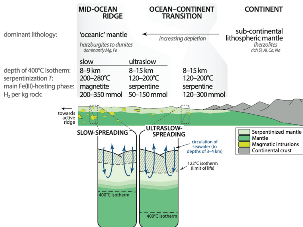
Figure 13. Sketch of natural H 2 generation related to serpentinisation at (magma-poor) rifted margins, as well as ultraslow- and slow-spreading mid-oceanic ridges. Differences in H 2 generation potential are due to petrological variations in the serpentinising rocks, as well as due to changes in the thermal regime, which itself strongly depends on the divergence velocity.
