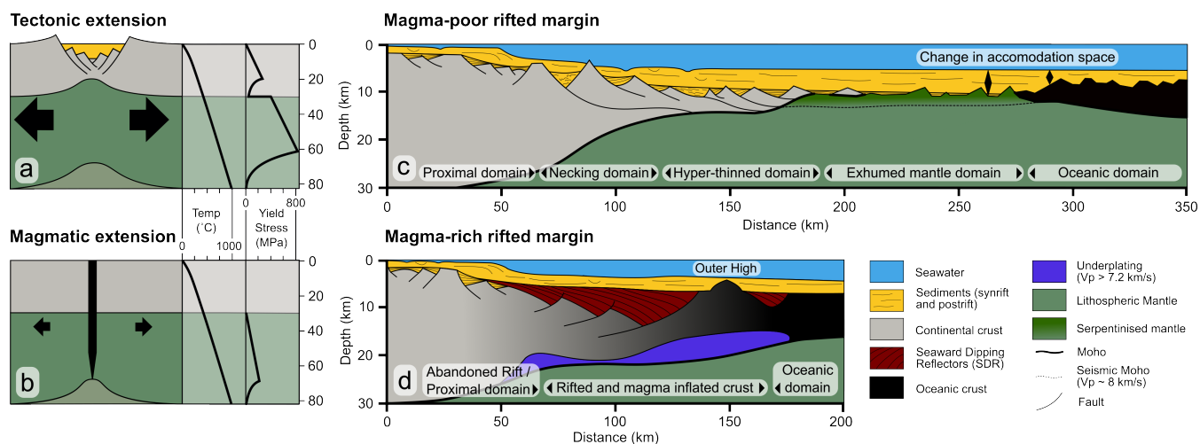
Figure 5. Schematics of rifting without (a) and with (b) contemporaneous magmatic intrusions, redrawn from Buck (2006). The yield stress required for extension to progress is significantly lower where magmatic injections weaken the lithosphere. The related characteristics of magma-poor and magma-rich rifted margins, which form during rifting without and with contemporaneous magmatism, are shown in panels (c) and (d), respectively.
