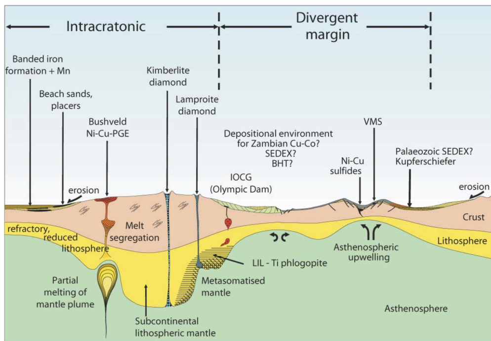
Figure 11. Schematic diagram of major mineral deposit types formed in continental crust, and along passive continental margins and oceanic spreading ridges. Adopted from Groves and Bierlein (2007).
