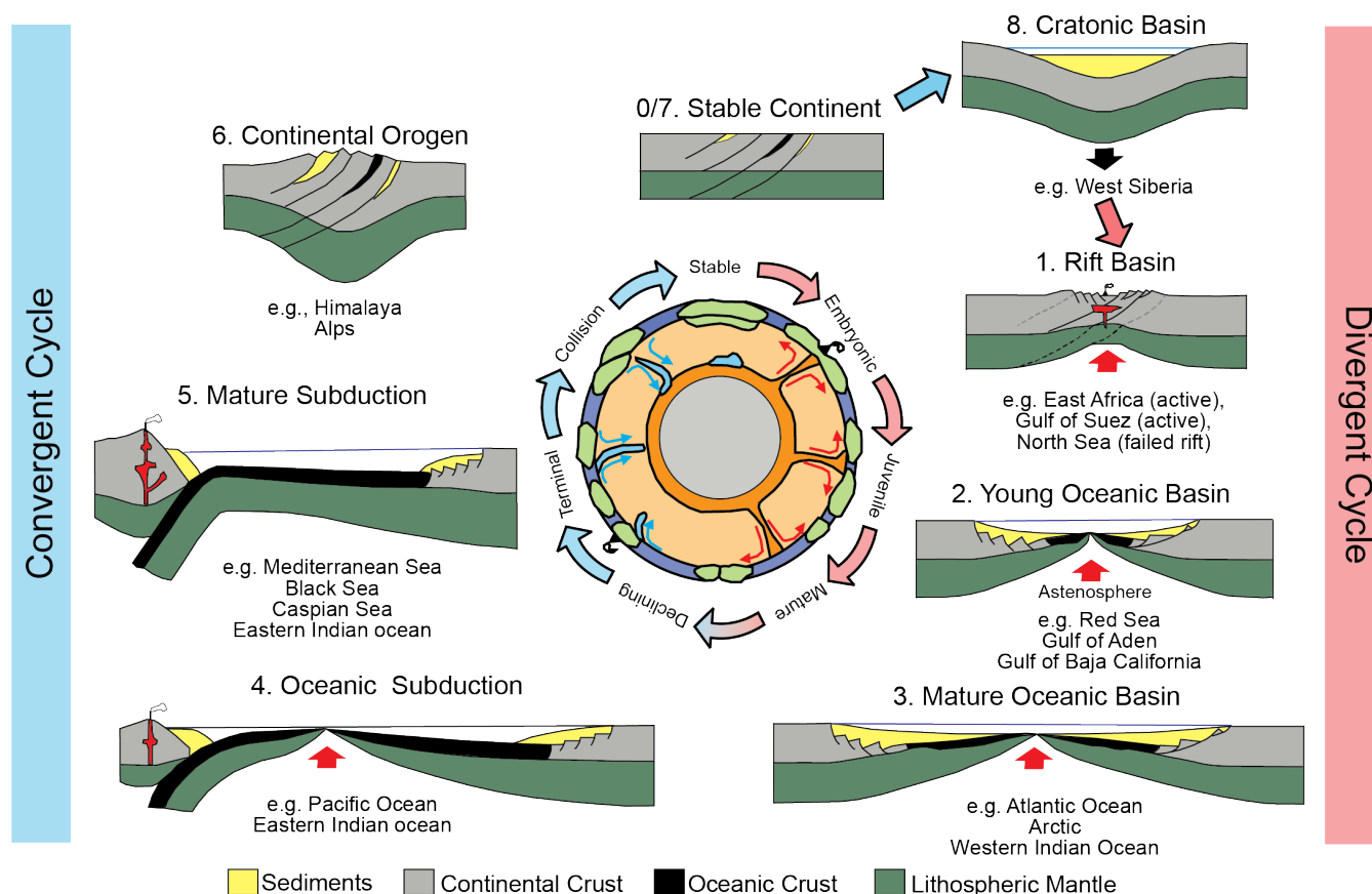
Figure 1. Schematic representation of the Wilson cycle, as originally proposed by Wilson (1968). Image modified after Wilson et al. (2019).
