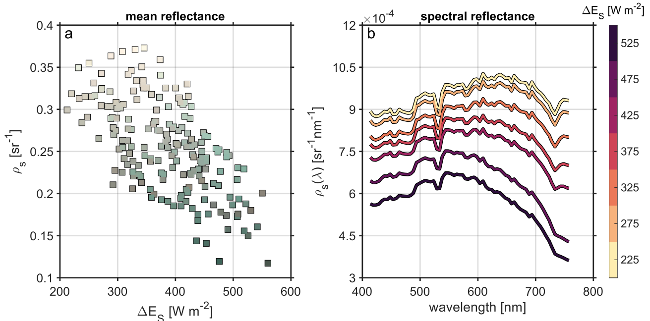
Figure 7. a Variation of spatially-averaged surface reflectance \rho_s [sr -1 ] Reviewer #2: —averaged over 400-800 nm wavelength and partitioned into 30-second discrete segments of flight—with net solar irradiance. Marker color corresponds to the surface color determined by the red, green, and blue channels of \rho_s . b Spatially-averaged spectral surface reflectance \rho_s(\lambda) [sr -1 nm -1 ], with color indicating the bin-averaged net solar irradiance.
