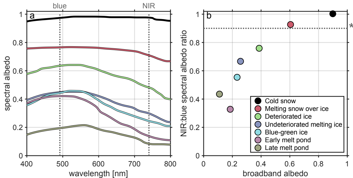
Figure 5. Spectral albedo a and the ratio between the spectral albedo in the near-infrared (NIR) and blue, or NIR:B b for a variety of classifications of first-year sea ice, organized by broadband albedo. Data shown in a were taken from Perovich (2017) and used to compute quantity shown in b . Asterisk in panel b indicates a NIR:blue ratio of 0.9.
