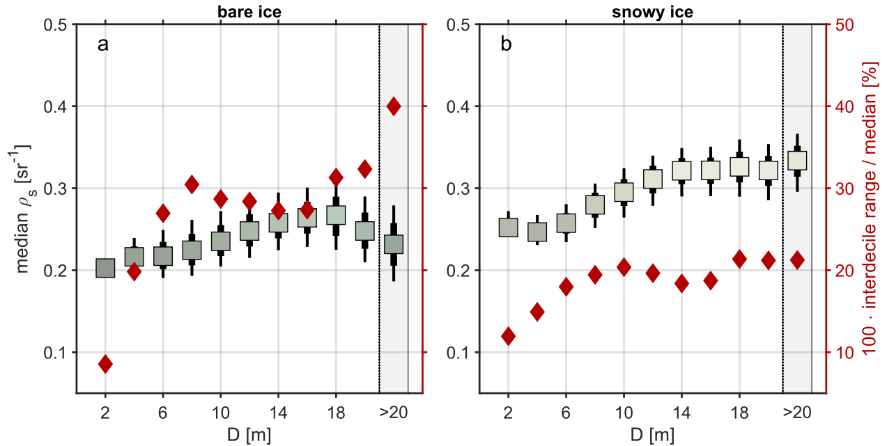
Figure 11. Variation of bare and snowy (a & b, respectively) ice feature surface reflectance \rho_s with feature size. Marker color indicates the mean feature color; thick and thin vertical lines mark the interquartile and interdecile ranges of \rho_s for each bin. Rust-colored diamonds indicate the ratio between the interdecile range and median value of \rho_s , represented as a percentage. The markers in the gray shaded region represent values computed for all features with D > 20 m.
