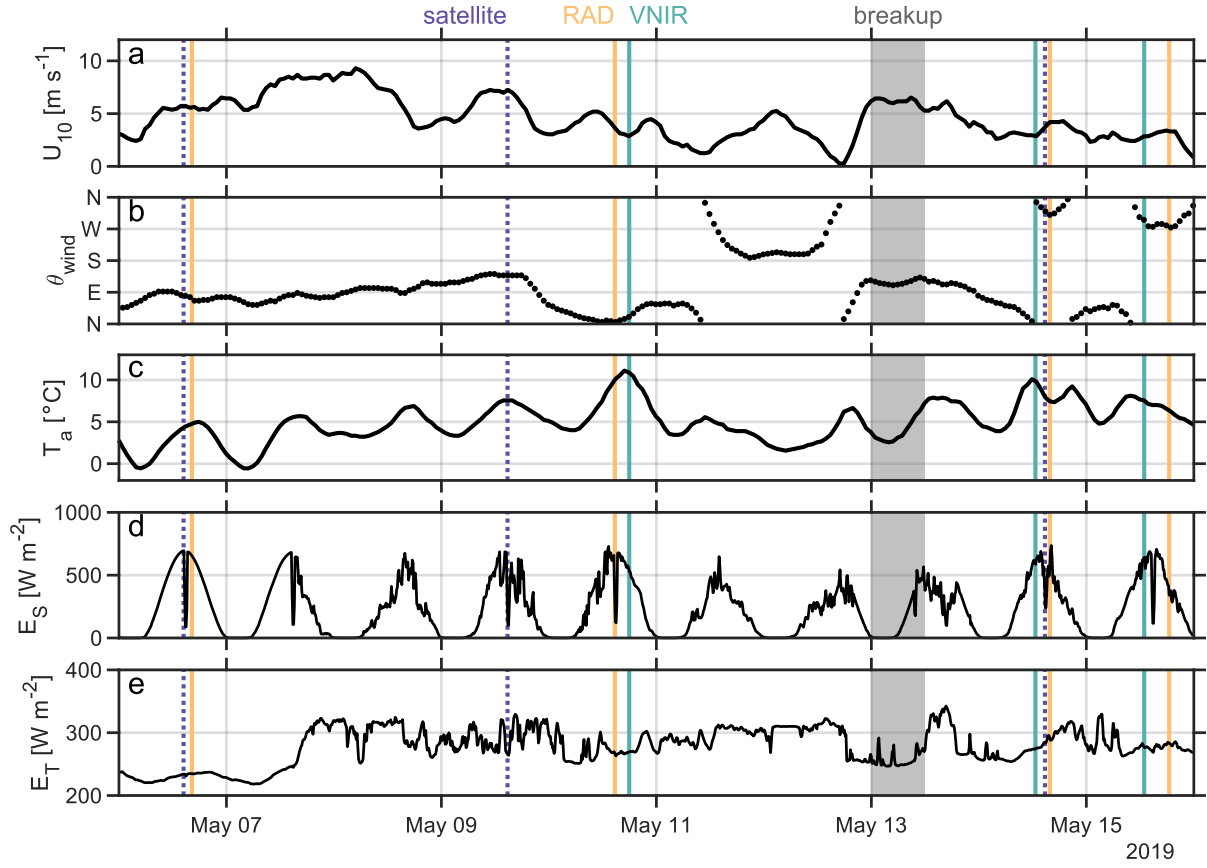
Figure 2. Environmental conditions during field campaign: a wind speed, b wind direction (coming-from convention), c air temperature, d downwelling solar irradiance, and e downwelling thermal irradiance. Wind/air measurements were made at Kotzebue Ralph Wien Airport, while radiative measurements were made at the U.S. Fish & Wildlife Service bunkhouse. Vertical lines indicate times of satellite overpasses (dotted violet), UAV flights with "RAD" payload (solid orange), UAV flights with "VNIR" payload (solid teal); gray shaded region denotes approximate time of major sea ice breakup.
