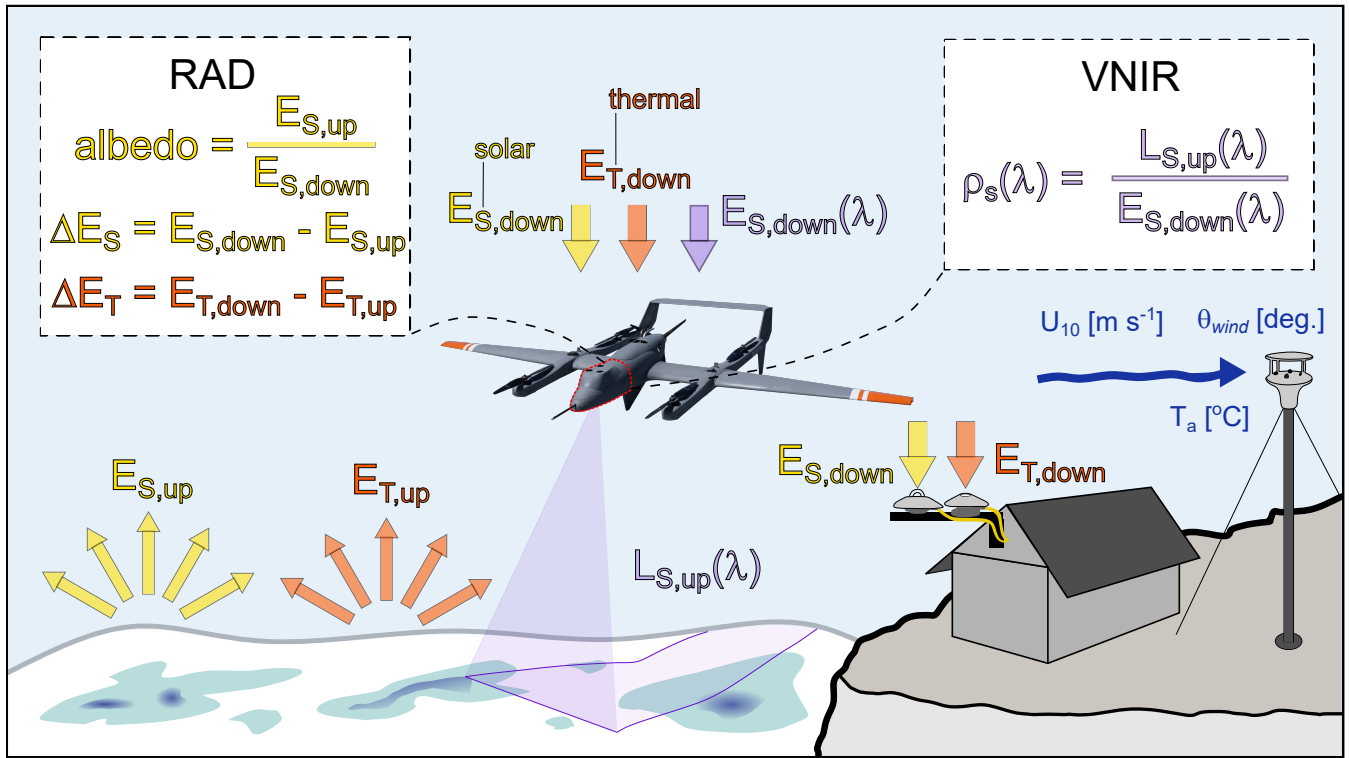
Figure 3. Depiction of fixed and aerial observational platforms, with arrows indicating radiative fluxes. Red dashed region on UAV indicates modular nosecone, with two red dashed boxes showing the measurement capabilities of two payloads: "RAD" payload, with upward/downward-looking pyranometers and pyrgeometers for characterizing upwelling and downwelling thermal and solar radiative fluxes; "VNIR" payload, with a downward-looking hyperspectral pushbroom imager and upward/downward-looking spectrometers for characterizing the spectral surface reflectance. Downwelling thermal and solar radiative fluxes were also measured from a rooftop station at the U.S. Fish and Wildlife Service bunkhouse. Wind speed, direction, and air temperature were measured from a meteorological station at Kotzebue Ralph Wien Airport.
