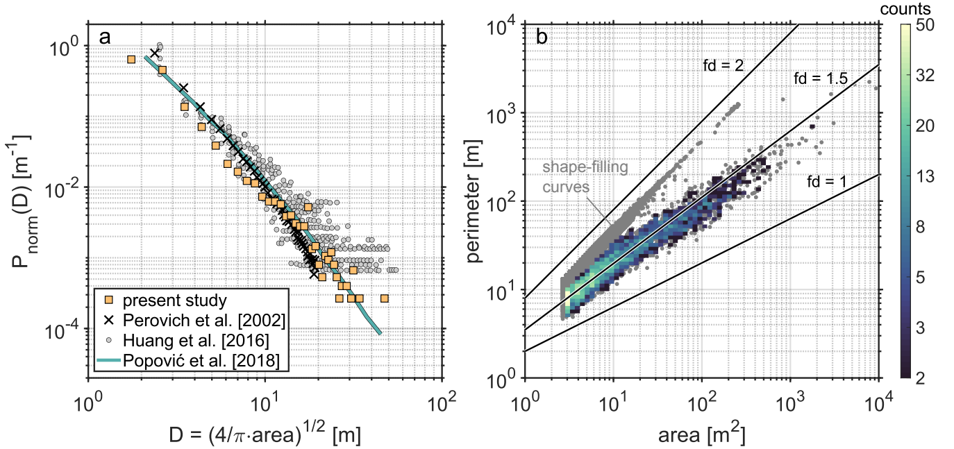
Figure 8. a melt pond size probability density functions, represented in terms of the pond effective diameter D . The observational data of Perovich et al. (2002) and Huang et al. (2016) are shown alongside the physical model of Popović et al. (2018) and observational data from the present study. b melt pond area-perimeter plot, with individual measurements represented by gray dots and the overlying color indicating the value of the corresponding bivariate histogram. Three lines overlaid on the figure correspond to fractal dimensions of 1, 2, and 1.5, the "pond distribution dimension" defined by Horvat et al. (2020).
