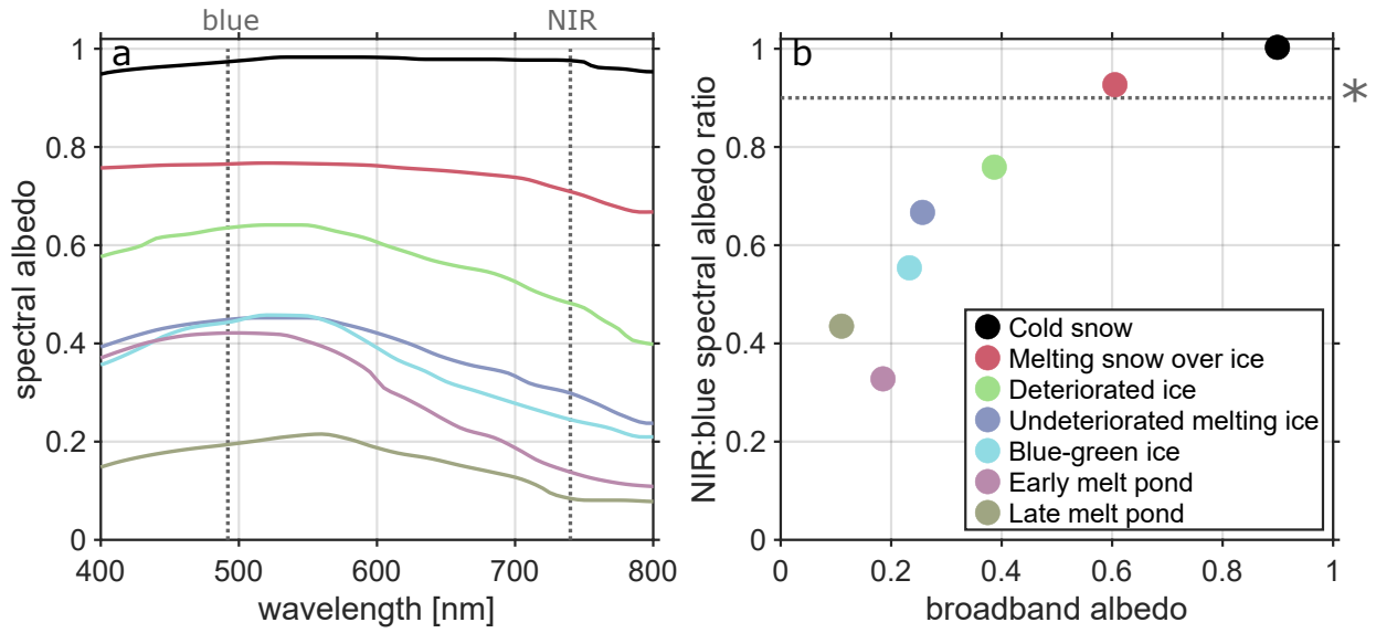
Figure 5. Spectral albedo a and the ratio between the spectral albedo in the near-infrared (NIR) and blue, or NIR:B b for a variety of classifications of first-year sea ice, organized by broadband albedo. Data shown in a were taken from Perovich (2017) and used to compute quantity shown in b . Asterisk in panel b indicates a NIR:blue ratio of 0.9.
