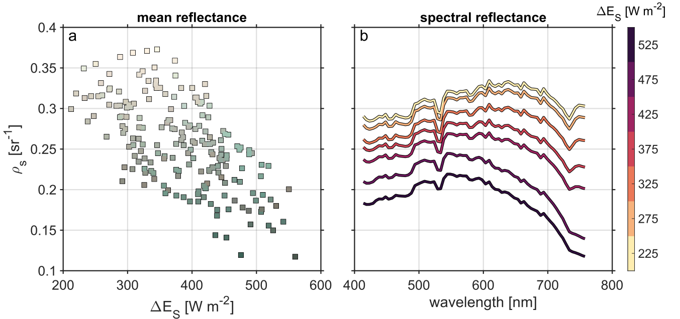
Figure 7. a Spatially-averaged surface reflectance \rho_s [sr -1 ] as a function of net solar irradiance. Marker color corresponds to the surface color determined by the red, green, and blue channels of \rho_s . b Spatially-averaged spectral surface reflectance \rho_s(\lambda) [sr -1 nm -1 ], with color indicating the bin-averaged net solar irradiance.
