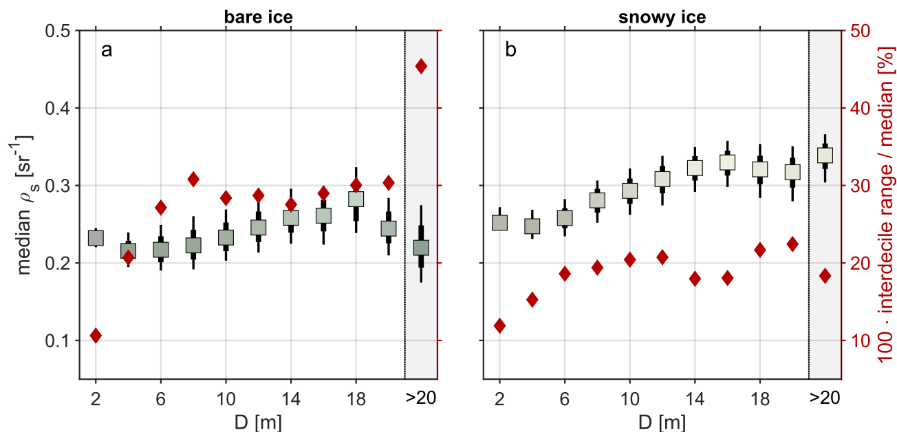
Figure 11. Variation of bare and snowy (a & b, respectively) ice feature surface reflectance \rho_s with feature size. Marker color indicates the mean feature color; thick and thin vertical lines mark the interquartile and interdecile ranges of \rho_s for each bin. Rust-colored diamonds indicate the ratio between the interdecile range and median value of \rho_s , represented as a percentage. The markers in the gray shaded region represent values computed for all features with D > 20 m.
