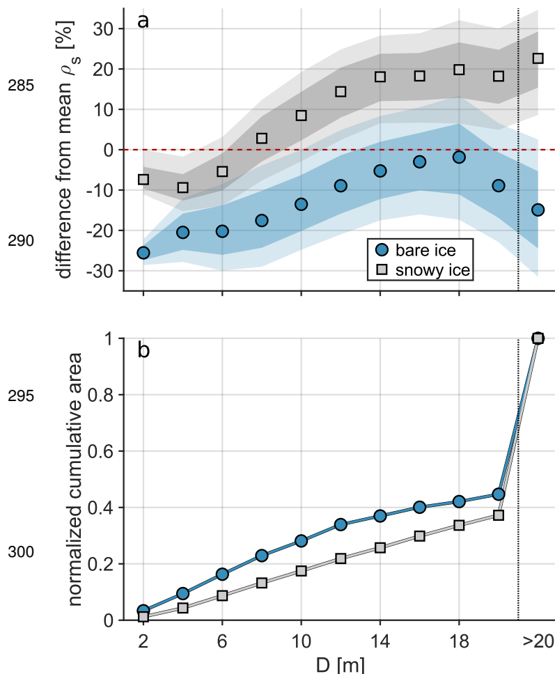
Figure 12. a Variation of \rho_s with feature size D , expressed as percent difference from the area-weighted average surface reflectance and partitioned into bare (teal circles) and snowy (gray squares) categories. Shaded regions indicate interquartile and interdecile ranges of variation. b normalized cumulative area of features with diameter less than or equal to D .
