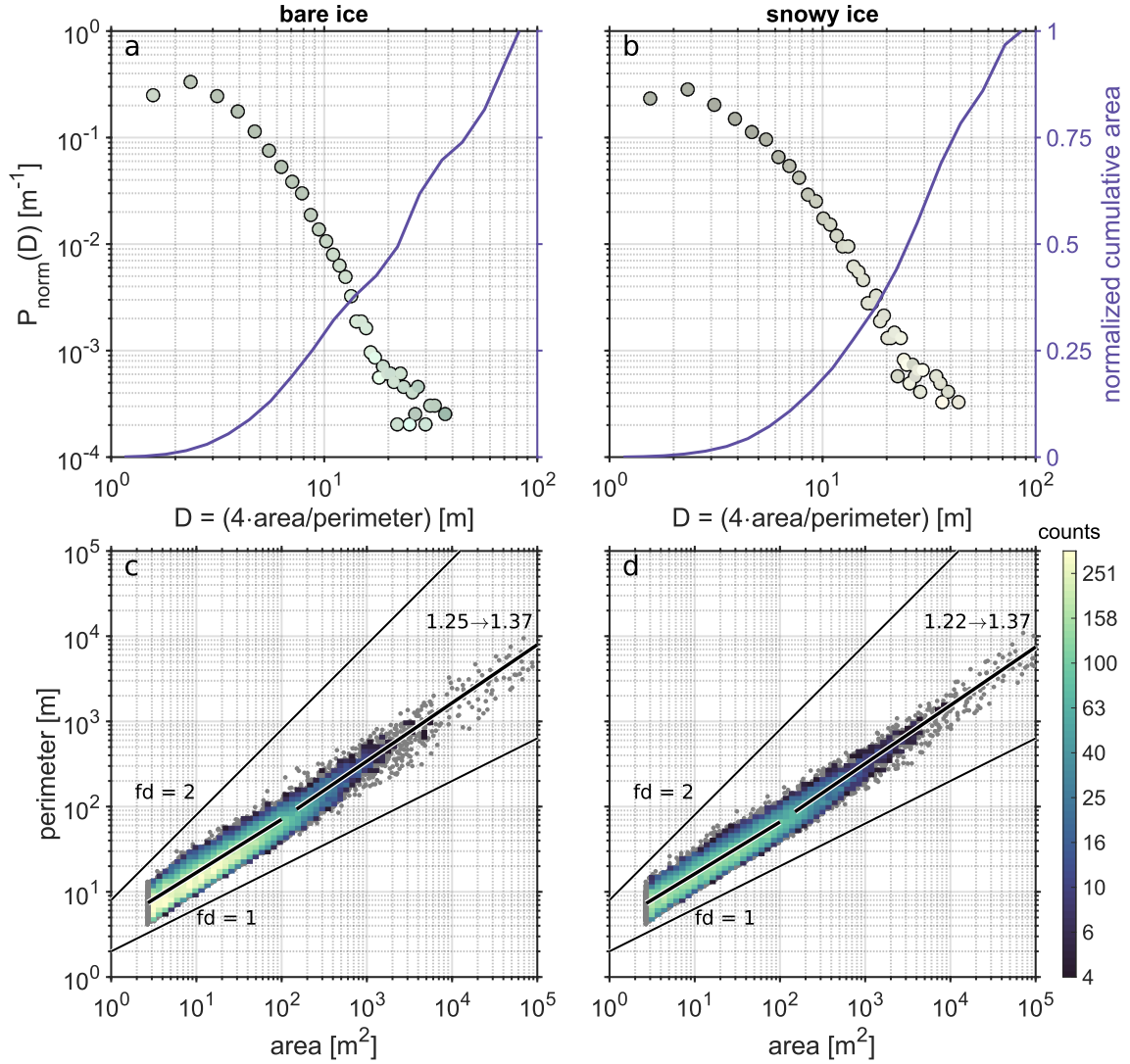
Figure 9. a,b Bare and snowy ice feature size probability density functions (left axes) & normalized cumulative area (right axes). PDF marker color corresponds to the mean feature color for a particular size bin. c,d Bare and snowy feature area-perimeter plots, with individual measurements overlaid with a bivariate histogram. Two lines in panels c & d correspond to fractal dimensions of 1 and 2; the piecewise linear functions correspond to fractal dimensions computed over two regimes: areas ranging from 2.6 \text{ m}^2 - 100 \text{ m}^2 and 150 \text{ m}^2 - 100,000 \text{ m}^2 .
