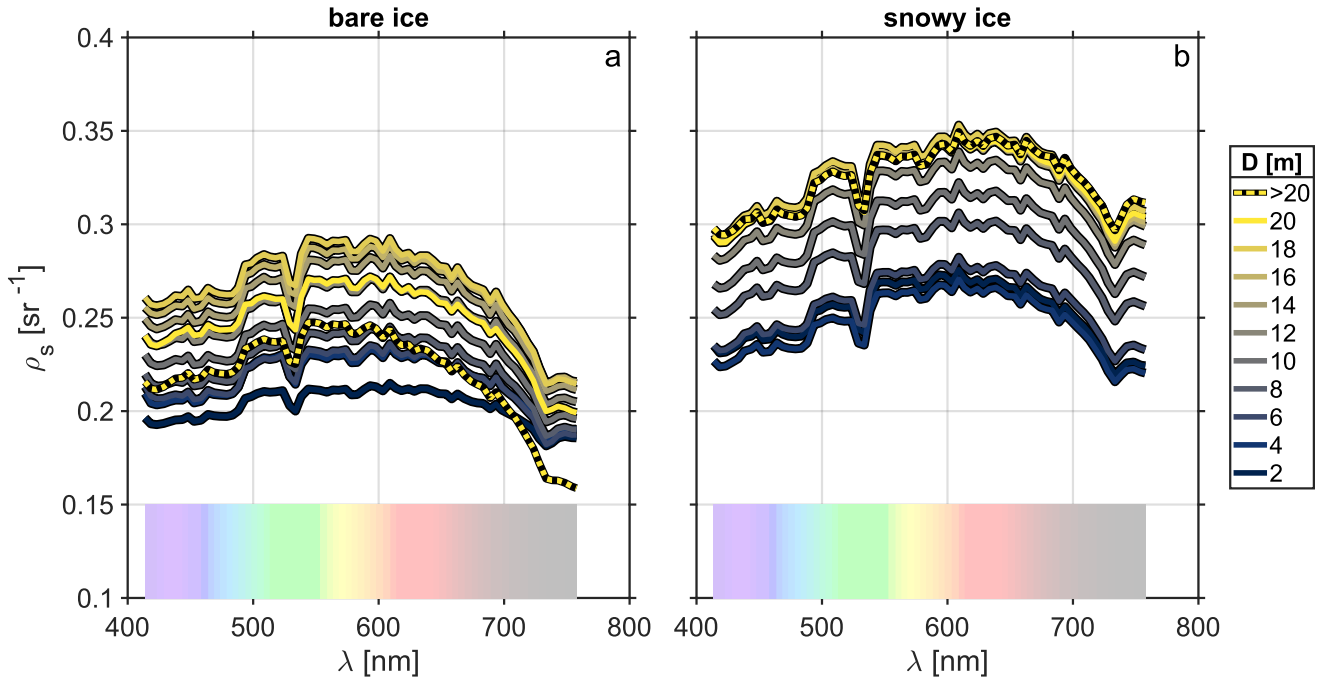
Figure 10. Surface reflectance spectra \rho_s(\lambda) for bare and snowy ice (left and right panels, respectively). Reviewer #2: The thickness of each trace corresponds to The color of each trace indicates the mean effective feature diameter D for which the spectra were bin-averaged. The dotted trace corresponds to the average for D > 20 m. The translucent rainbow bar at the base of the plot indicates the approximate color corresponding to each particular wavelength.
