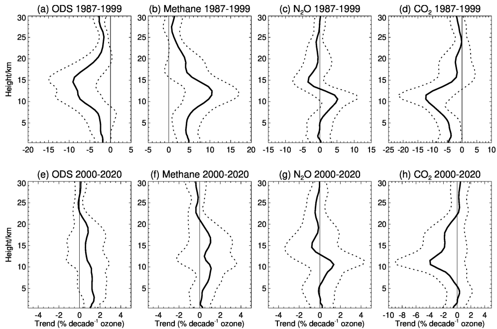
Figure B1. Ozone trend changes due to changes in the ozone depleting substances (ODS), methane, nitrous oxide (N 2 O), and CO 2 for the periods of 1987-1999 (a, b, c, d, respectively) and 2000-2020 (e, f, g, h, respectively) simulated in NIWA-UKCA CCM1 simulations. The 2σ uncertainty range is marked by dotted lines. Trends in ozone are averaged in the area of 160°E-180°E and 40°S-50°S (representing the location of Lauder).
