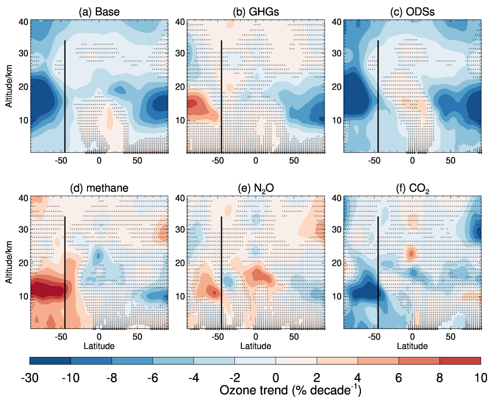
Figure B2. Trends in zonal mean ozone between 1987 and 1999 from the NIWA-UKCA CCM1 RefC2 simulation (a), and the change in zonal mean ozone trend due to changes in (b) greenhouse gases (GHGs), (c) ozone depleting substances (ODSs), (d) methane, (e) nitrous oxide ( \text{N}_2\text{O} ), and (f) \text{CO}_2 over the same period. Black vertical lines indicate the latitude of Lauder Station.
