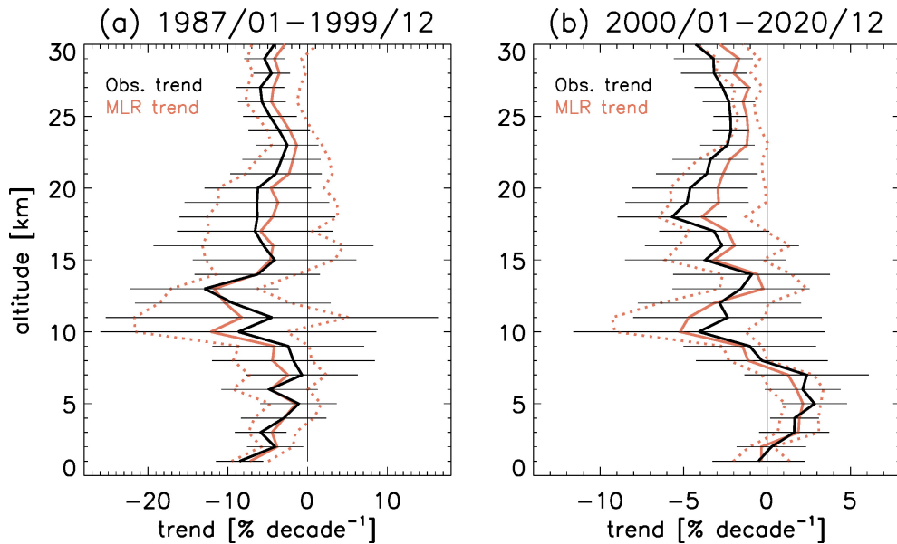
Figure 4. Vertically resolved linear trends in regressed ozone (orange) and in the homogenised observed ozone (black) and their uncertainties ( \pm 2\sigma ) at Lauder over two periods, i.e., 1987–1999 (a) and 2000–2020 (b). Data used for linear trend calculations in both cases are annual mean anomalies.
