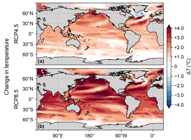
Figure C1. (a) Change in vertical mean euphotic temperature, \Delta T , for the RCP4.5 scenario. (b) As (a) but for RCP8.5.
