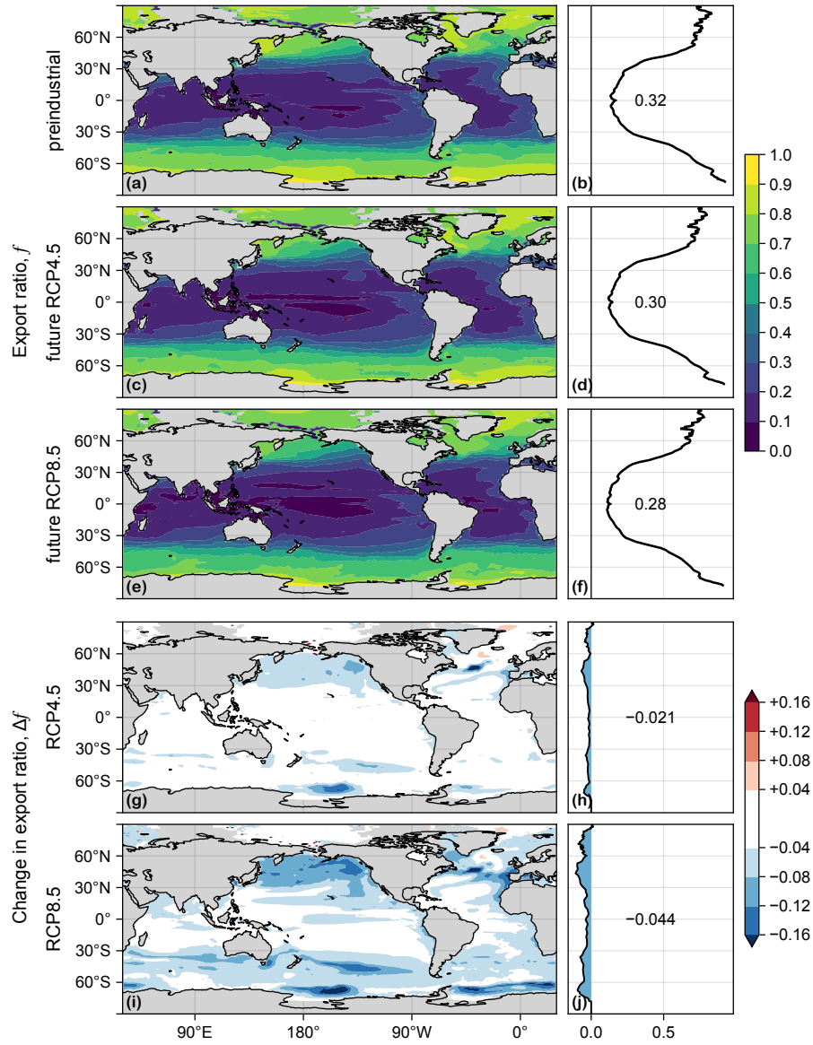
Figure D2. As Fig. 2 but for (a) Map of export ratio, f , in the preindustrial state. (b) Zonal mean of (a). (c–d) As (a–b) for the future RCP4.5-based state. (e–f) As (c–d) for RCP8.5. (g–j) As (c–f) for \Delta f .
