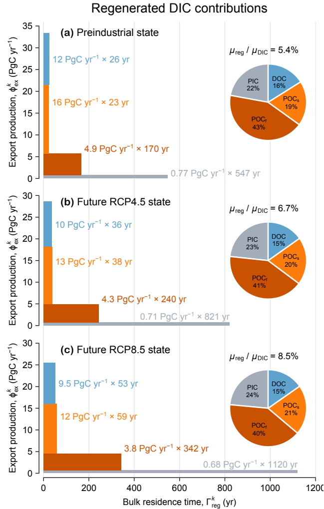
Figure 5. (a) Regenerated DIC contributions from each mechanism k = \text{DOC}, \text{POC}_s, \text{POC}_f, \text{and PIC} (blue, orange, red, and grey) for the preindustrial state represented as both a pie chart and a bar chart. The pie chart quantifies the fractional contribution \mu_{reg}^k / \mu_{reg} . Pump sequestration strength, as quantified by \mu_{reg} / \mu_{DIC} , is indicated above the pie chart. Each bar can be interpreted as a pipe flowing from left to right and whose area represents the regenerated DIC inventory, \mu_{reg}^k , which equals globally integrated export production, \Phi_{ex}^k (pipe width, y -axis) multiplied by bulk residence time, \Gamma_{reg}^k (pipe length, x -axis). (b) As (a) but for the future RCP4.5 state. (c) As (b) but for RCP8.5.
