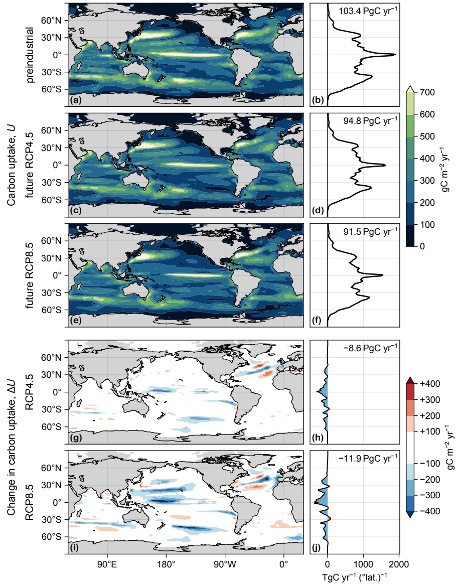
Figure D1. (a) Map of carbon uptake, U(\mathbf{r}) , vertically integrated, in the preindustrial state. (b) Zonal integral of (a). (c–d) As Fig(a–b) for the future RCP4.5-based state. 2 but (e–f) As (c–d) for DIC uptake, U_{\text{RCP8.5}} . (biological production–j) As (c–f) for \Delta U .
