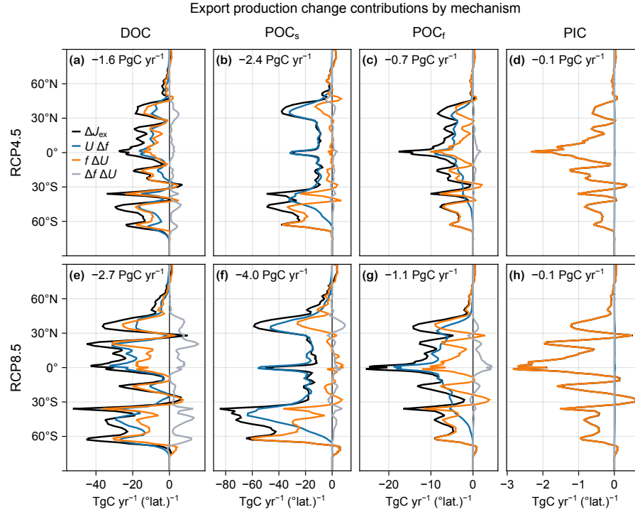
Figure D3. (aa-d) -(d) Change in DOC (a), POC r_s (b), POC r_f (c), and PIC (d) zonally integrated export production, \Delta J_{\text{ex}} (black), for the RCP4.5-based state, decomposed into contributions from U \Delta f (blue), f \Delta U (orange), and \Delta f \Delta U (gray). The globally integrated contribution to \Delta J_{\text{ex}} is indicated in each panel. (ee-h) -(h) As (aa-d) -(d) but for the RCP8.5-based state.
