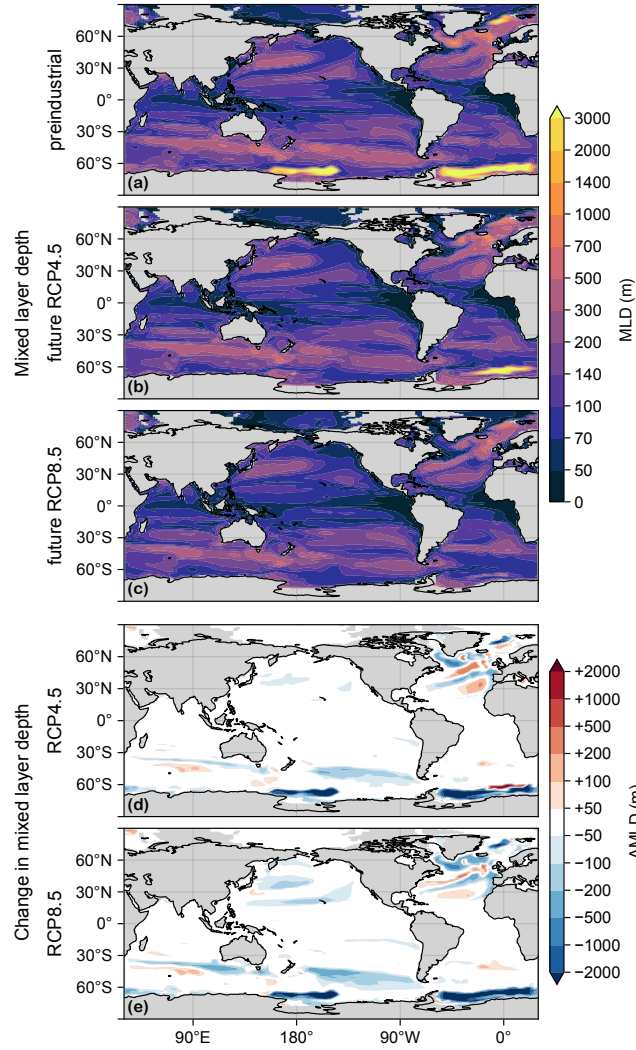
Figure C2. (a) Mixed layer depth (MLD) for the preindustrial state. (b) As (a) for the future RCP4.5 state. (c) As (b) but for RCP8.5. (d-e) As (b-c) for the change in mixed layer depth, \Delta MLD.
