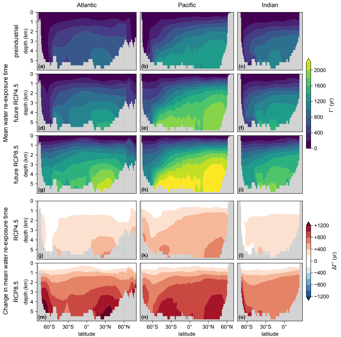
Figure C3. (aa-c)-(e) Mean water reexposure -re-exposure time, \Gamma^\uparrow , for the preindustrial circulation, zonally averaged over the Atlantic (a), Pacific (b), and Indian Ocean (c). (dd-f)-(f) As (aa-c)-(e) but for the RCP4.5 state. (gg-i)-(i) As (dd-f)-(f) but for RCP8.5. (jj-o)-(o) As (dd-i)-(i) but for \Delta\Gamma^\uparrow .
