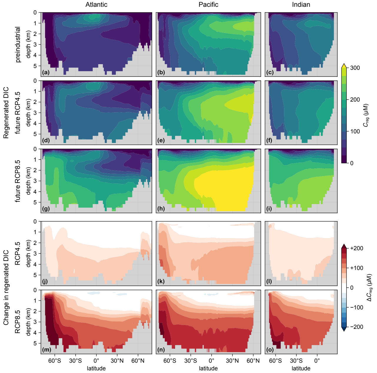
Figure 4. (aa–c)–(e) Zonal mean C_{\text{reg}} for the preindustrial state in the Atlantic (a), Pacific (b), and Indian Ocean (c). (For all zonal means shown in this work, the Atlantic basin excludes the Gulf of Mexico and the Caribbean, and the Pacific basin excludes the Sea of Japan so that the averages are more cleanly interpretable.) (dd–f)–(f) As (aa–c)–(e) but for the future RCP4.5-based state. (gg–i)–(i) As (dd–f)–(f) but for RCP8.5. (jj–o)–(o) As (dd–i)–(i) but for \Delta C_{\text{reg}} .
