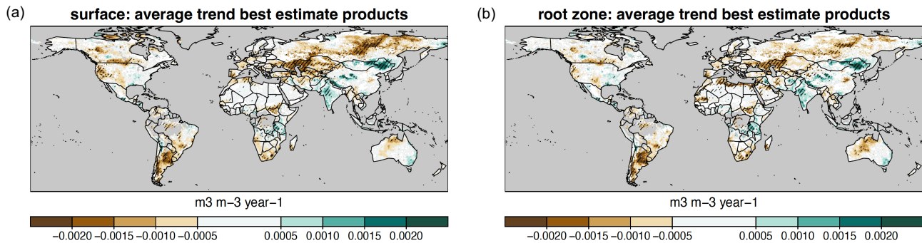
Figure 9 Best-estimate products average of 2000–2022 Theil-Sen trends ( \text{m}^3 \text{m}^{-3} \text{yr}^{-1} ) on yearly mean (a) surface and (b) root-zone soil moisture. Underlying daily data is masked based on the ESA-CCI-COM (a) (and -RZSM, b) data availability, and non-frozen soil conditions of ERA5-Land (a, b). The mean trends are only shown in areas with trend direction agreement of both respective best-estimate products, while white colour denotes no consensus in the trend direction. Additionally, areas of common significant trends are hatched.
