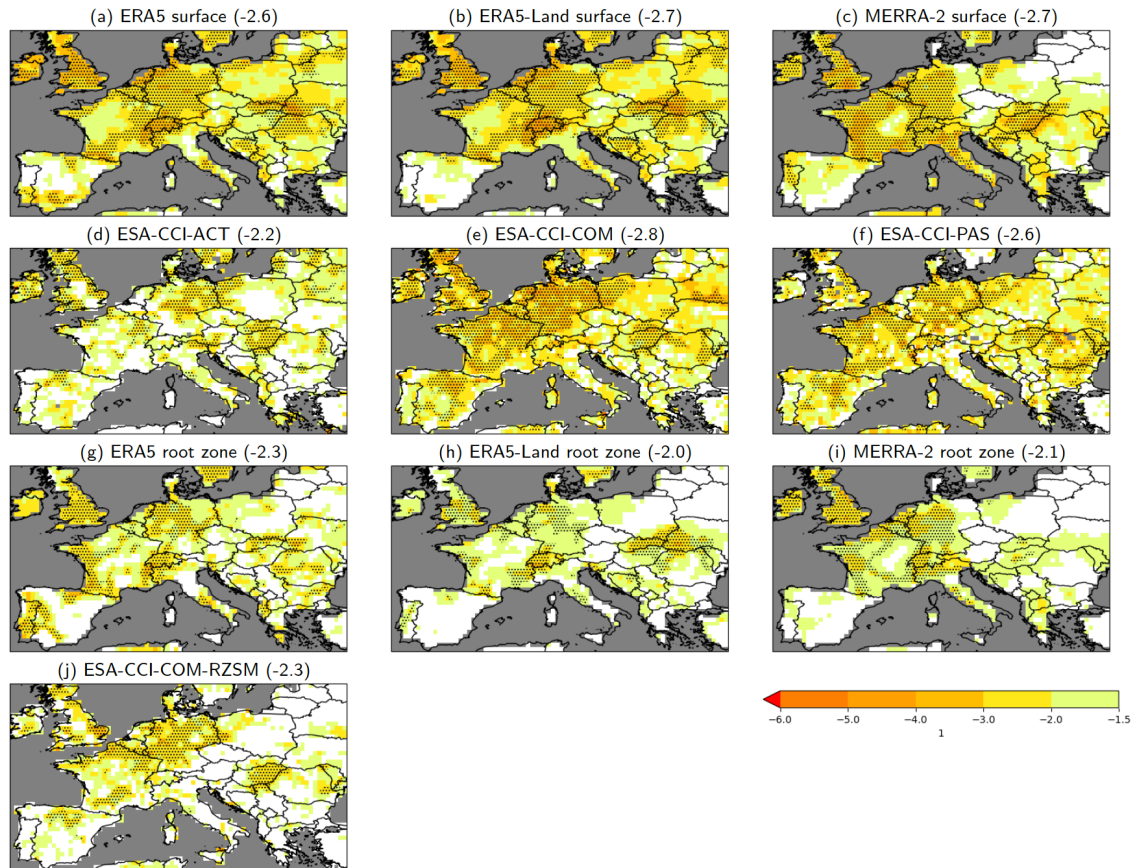
435 Figure 4 Magnitude of the 2022 Europe drought event (in standard deviations) based on the temporal minimum of the standardised soil moisture anomalies in (a–f) the surface and (g–j) the root zone layer. The core of the event region is stippled, and the area mean of the magnitude over the respective core of the event region is denoted in brackets.
