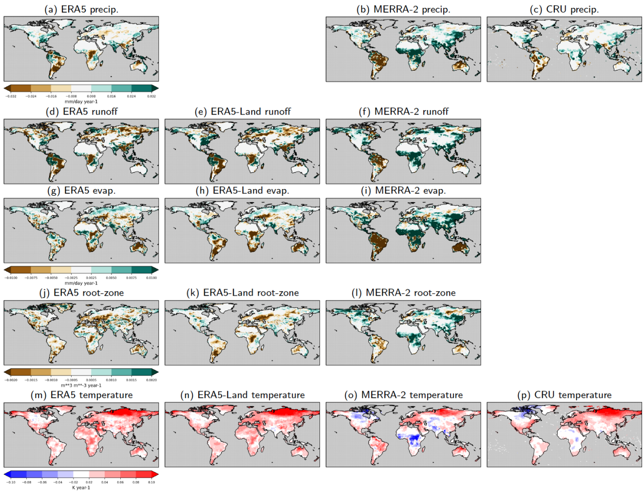
405 Figure 2 Theil-Sen trend estimate (2000–2022 period) on yearly means of monthly precipitation (a–c), runoff (d–f), evapotranspiration (g–i), root-zone soil moisture (j–l) and surface air temperature (m–p) from the reanalysis products as well as two gridded stations-based datasets for precipitation and temperature. Values are in mm/d yr -1 for the fluxes, respectively m 3 m -3 yr -1 for soil moisture and K yr -1 for temperature. Regions with non-significant trends are not masked out for easier comparison with the trends in soil moisture. Note that ERA5-Land is forced by ERA5 precipitation and is thus not shown for the former.
