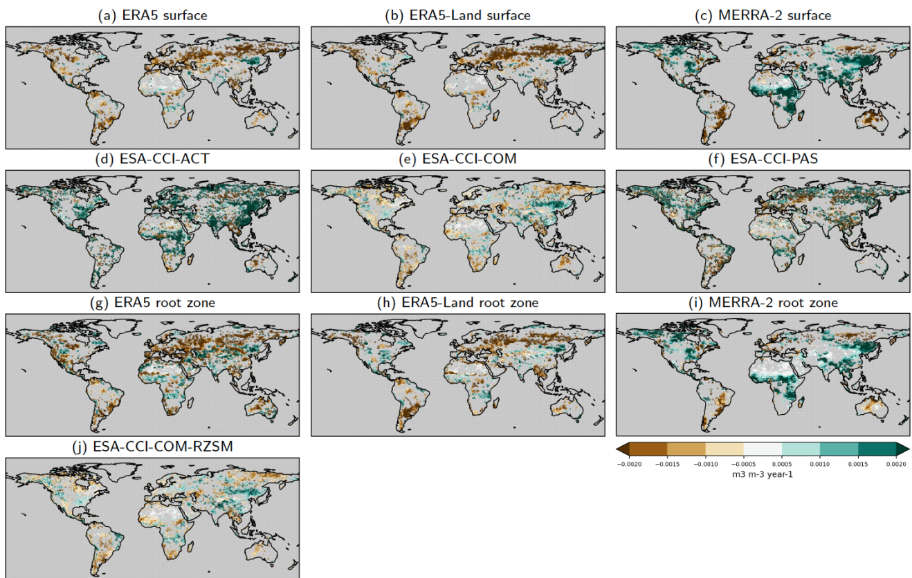
Figure 1 Theil-Sen trend estimate ( \text{m}^3 \text{m}^{-3} \text{yr}^{-1} ) on yearly mean soil moisture (based on daily data mutually masked for ESA CCI data availability and non-frozen soil conditions of the reanalysis products) in (a–f) the surface and (g–j) the root zone layer, 2000–2022 period. A Mann-Kendall test with a false rejection rate (or alpha value) of 0.05 was performed to mask out regions where no significant trend is present.
