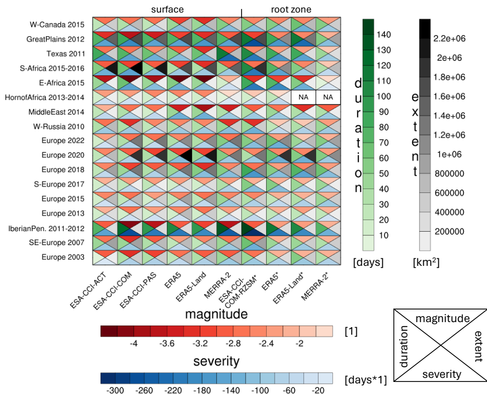
500 Figure 7 Drought metrics of recent major drought events. The values are based on surface soil moisture and root-zone soil moisture (products denoted with *) and represent the area mean over the respective core of the event region in case of severity, magnitude, and duration, and the temporal maximum in case of the spatial extent. NA is displayed when products do not exhibit standardized anomalies below -1.5 for a specific event.
