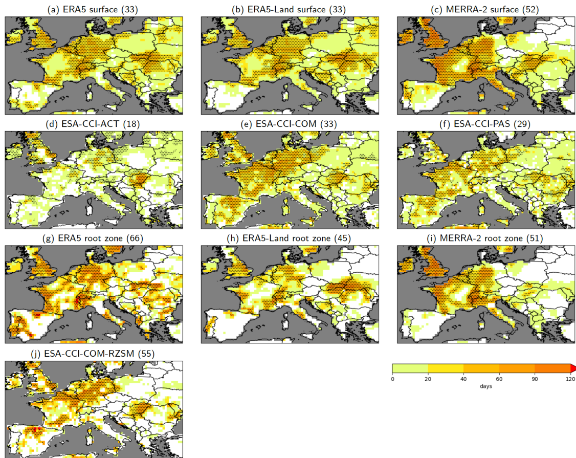
440 Figure 5 Duration of the 2022 Europe drought event (in days) based on the number of days within the event period with standardised soil moisture anomalies below -1.5 in (a–f) the surface and (g–j) the root zone layer. The core of the event region is stippled, and the area mean of the duration over the respective core of the event region is denoted in brackets.
