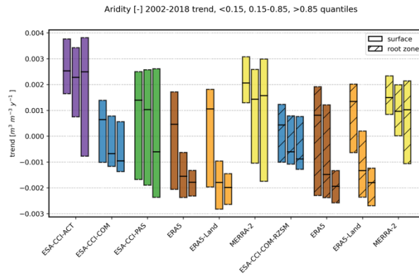
745 Figure A1 Distributions (median, inter-quartile range) of global soil moisture trends in the different products in relation to different quantile bins of trends in aridity (i.e., <0.15, 0.15-0.85, >0.85). Note that trends are not masked for significance.
