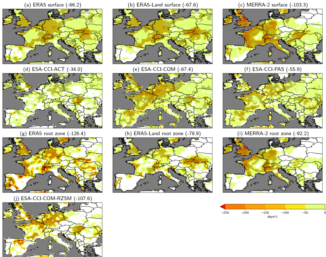
Figure 3 Severity of the 2022 Europe drought event (in days*1) based on the time accumulated soil moisture anomalies in (a–f) the surface and (g–j) the root zone layer. The core of the event region is stippled, and the area mean of the severity over the respective core of the event region is denoted in brackets.
