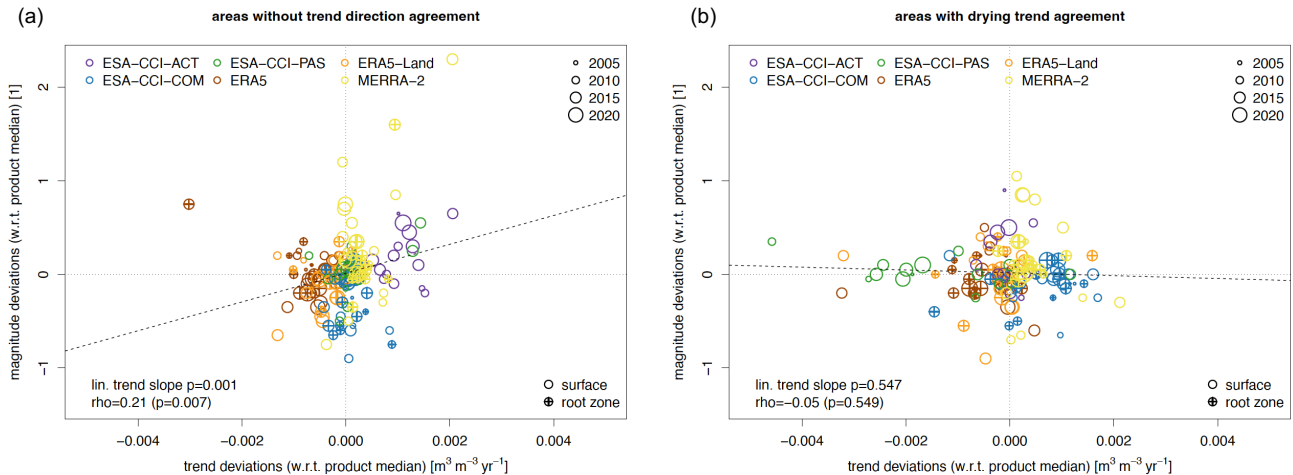
595 Figure 10 Product deviations in drought magnitude as a function of product deviations in the 2000–2022 soil moisture trends, with circle sizes depending on the chronology of the events within the investigated period (i.e., later events are displayed with larger circles). (a) Relation in areas without trend direction agreement of the products, (b) relation in areas with drying trend agreement. Deviations are displayed with respect to the product median of the individual events, separately calculated for the surface and the root zone (the latter additionally indicated with a “+”). The trends and drought magnitudes are averaged over the respective areas of drying trend agreement and trend direction disagreement within the drought regions. The p-values of the linear trend slope (dashed line) and the Spearman rank correlation rho between the drought metrics and the soil moisture trends are noted as well.
