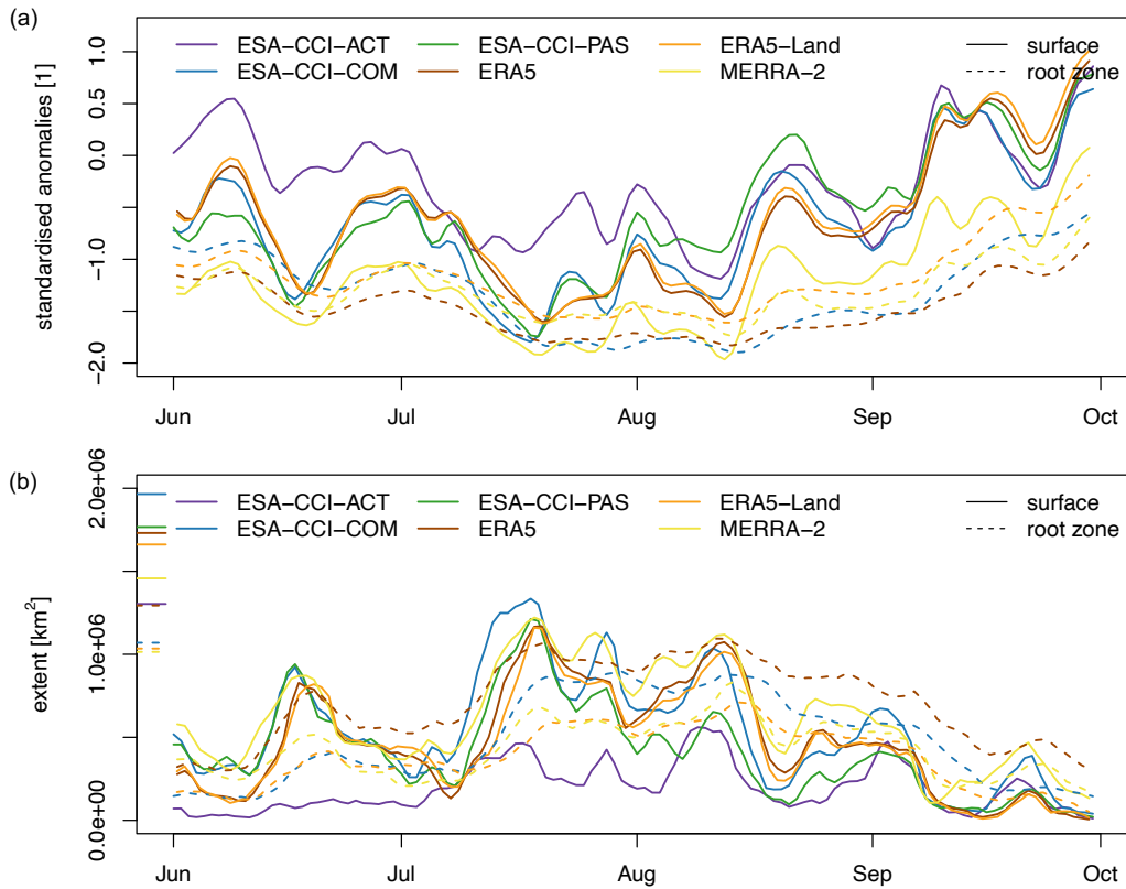
Figure 6 (a) Average of the standardised surface (full lines) and root-zone (dashed lines) soil moisture anomalies within the respective core of the event regions (cf. stippled regions in Figs. 1–3) during the 2022 Europe drought event period. (b) Spatial extent of the standardised surface (full lines) and root-zone (dashed lines) soil moisture anomalies below -1.5 within the core of the event region during the 2022 Europe drought event (full lines). Line segments at the left border of the figure indicate the extent of the core region for each dataset (i.e., corresponding to the extents of the stippled areas of Figs. 1–3 where the severity is larger than the median of all non-zero severity grid points).
