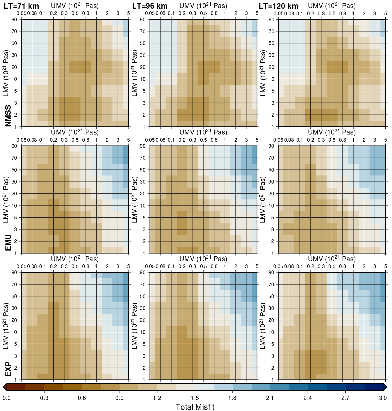
Figure 6. Plot shows proxy-data: model misfit for using the North-American-RSL composite database (Sect. 2.4) for the NMSS model (top row), the emulator (EMU, middle row), and the explicit 3D-SS RSL output from Seakon added onto the NMSS RSL output (EXP, bottom row) from top-to-bottom respectively. Misfit varies as a function of global mean lithosphere thickness from left to right. Results are for the S40RTS+LR18 3D model configuration.
