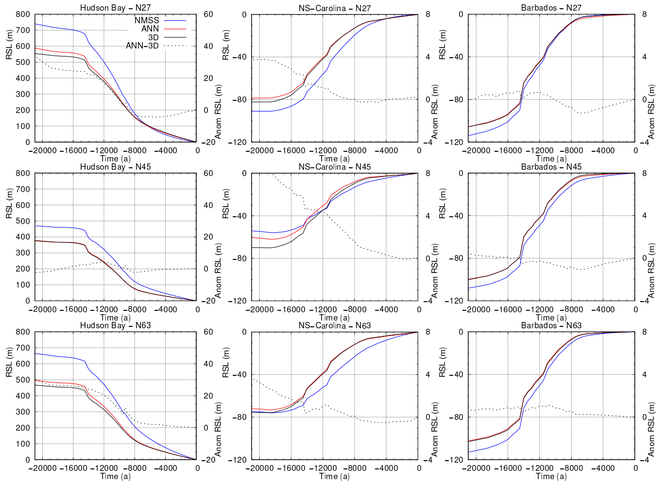
Figure 5. RSL timeseries for a near- (Hudson Bay), intermediate- (Northern S-Carolina), and far-field (Barbados) locations, for the N=27, 45 and 63 ANN training sets. Parameter vectors shown RSL curves are drawn from computed using the validation ensemble and are the median members (when considering the full spatio-temporal mean square error of the ANN). The 3D Earth model configuration shown is S40RTS+LR18. Note that since the parameter vector correspond vector corresponding to the median member of the MSE for each validation ensemble. As the parameter vector for the mean MSE generally varies with N, the resulting RSL curves themselves vary between N values also change.
