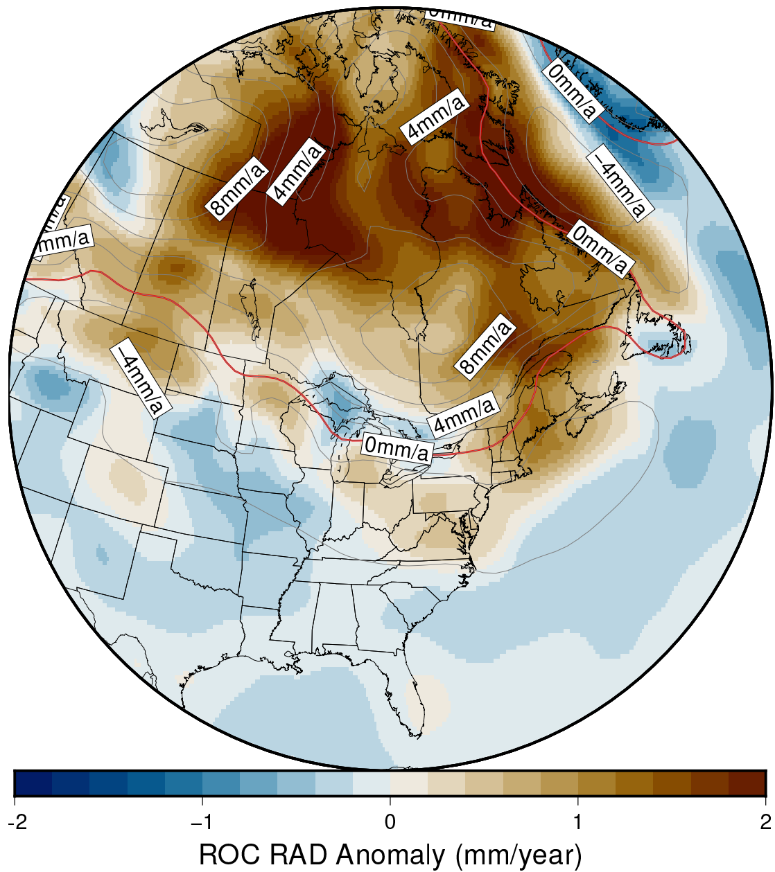
Figure 4. ROC Emulated RAD anomaly , emulated-RSL field minus explicit (3D-SS Seakon + NMSS) field for the S40RTS+LR18 case at present day. Contours denote the total, modelled ROC RAD field (from the explicit case) in 2 mm/yr increments; the red line denotes the 0 mm/yr contour. The parameter vector plotted is that with the median MSE, calculated for all spatio-temporal data, for the N = 45 ANN. A global map of the same field is shown in Fig. S4S7 , and an equivalent map but for 10 ka is shown in Fig. S5S8 .
