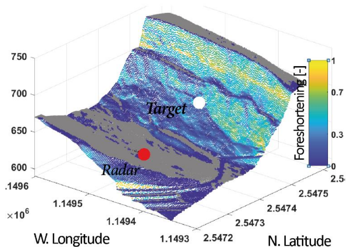
Figure A3: Additional output map for the second dataset, La Cornalle. a) The input map with the altitude, aimed at choosing the radar and target location b) The distance-to-radar map. The distance between the radar and the target should not be greater than 4 km. c) The foreshortening map, after the Equation 8.
