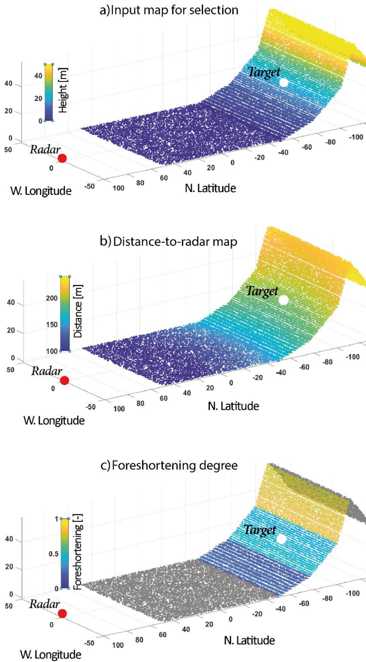
Figure A1: Additional output map for the synthetic dataset. a) The input map with the altitude, aimed at choosing the radar and target location b) The distance-to radar map. The distance between the radar and the target should not be greater than 4 km. c) The foreshortening map, after the Equation 8.
