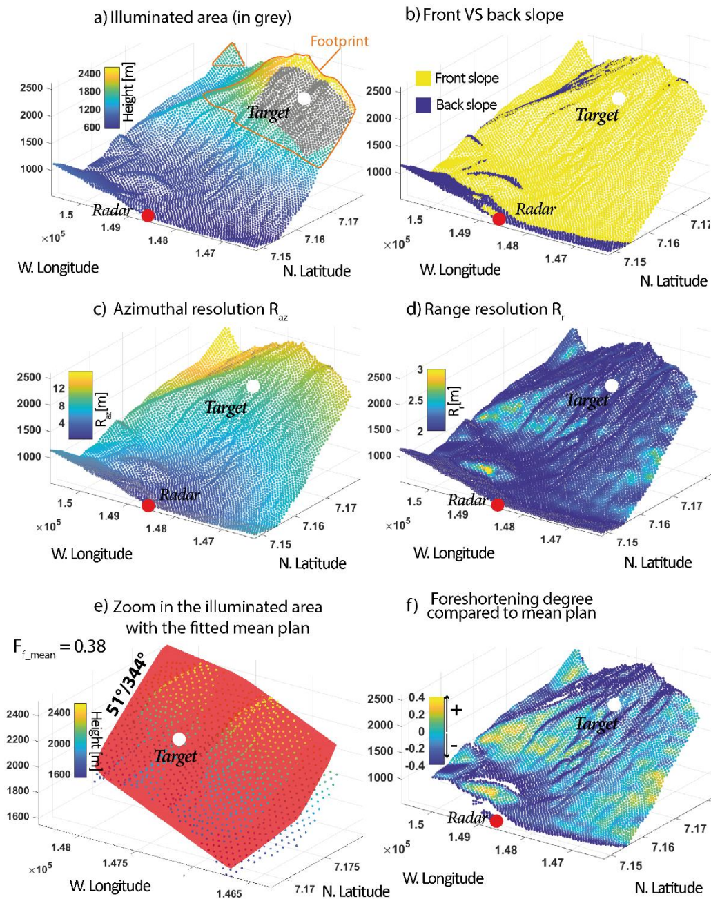
405 Figure 15 : Output maps for the first dataset, Cima del Simano. a) Illuminated area and footprint for the chosen parameters. b) Front VS back slope. The back slope corresponds to areas in shadow. c), d) Azimuthal and range resolutions. Since the chosen bandwidth is 75 MHz to be sure to record the backscattered signal, the resolutions are poor. Only a monitoring of major volume instabilities is relevant here. e) Zoom in the illuminated area for which a mean plan fitting is estimated. The mean dip of the area is 51^\circ with a mean foreshortening of 0.38. f) Foreshortening degree compared to the mean plan one. The lower part is more affected by foreshortening than the top of the mountain, which is the area of interest. The other output maps are presented in the Appendix B.
