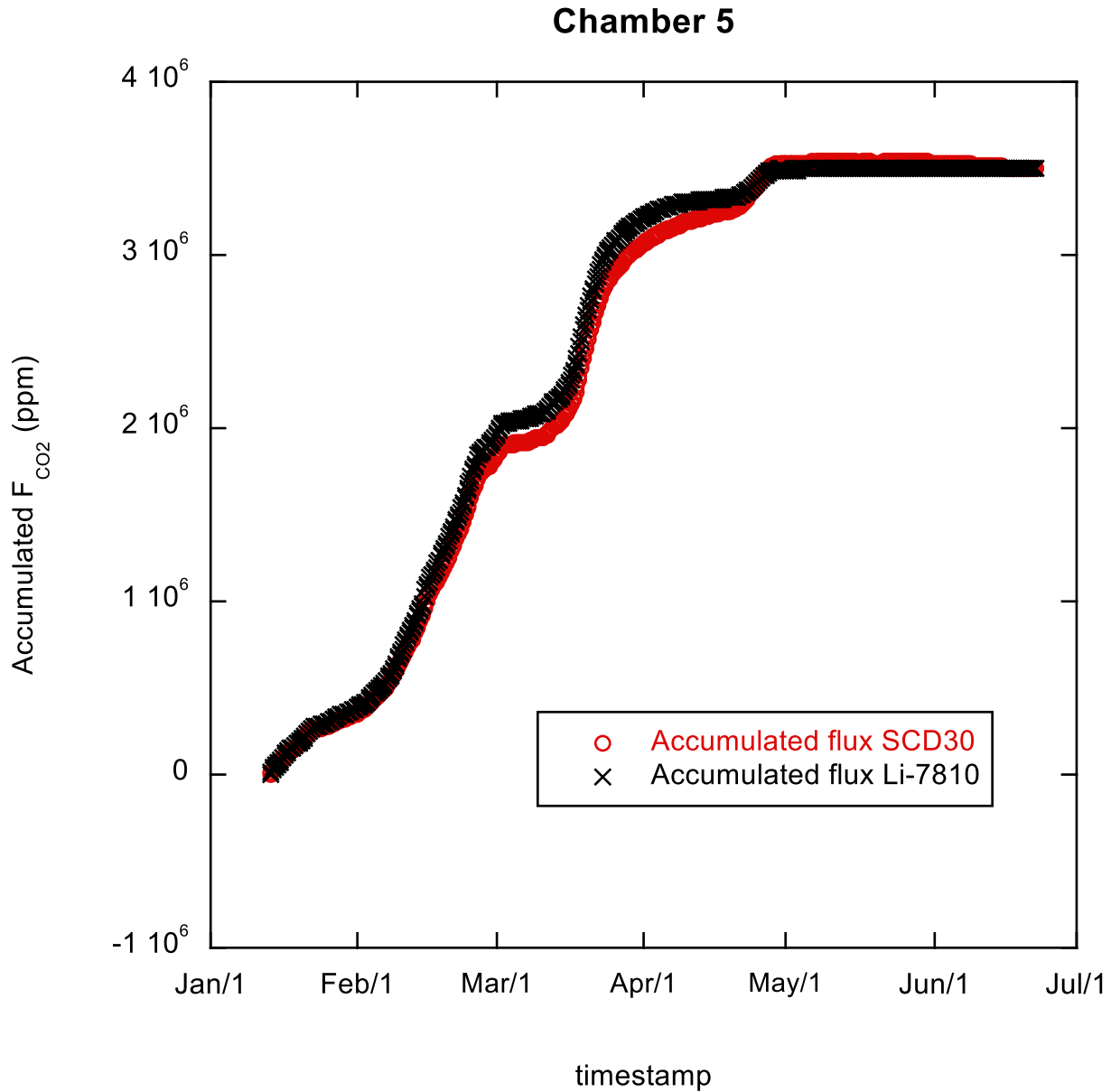
Figure 10. Accumulated fluxes from SCD30 and Li-7810 data.
