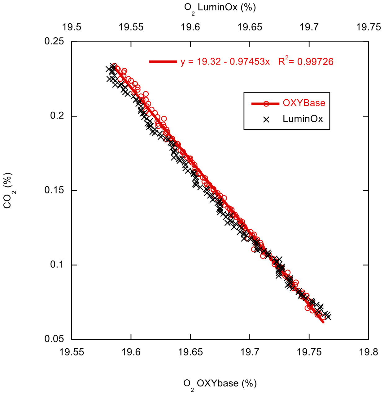
Figure 4415. CO 2 part measurements versus O 2 part measured by OXYBase (lower abscissa) and O 2 part measured by LuminOx (upper abscissa). The red solid line represents a linear regression of CO 2 versus O 2 measured by OXYBase.
