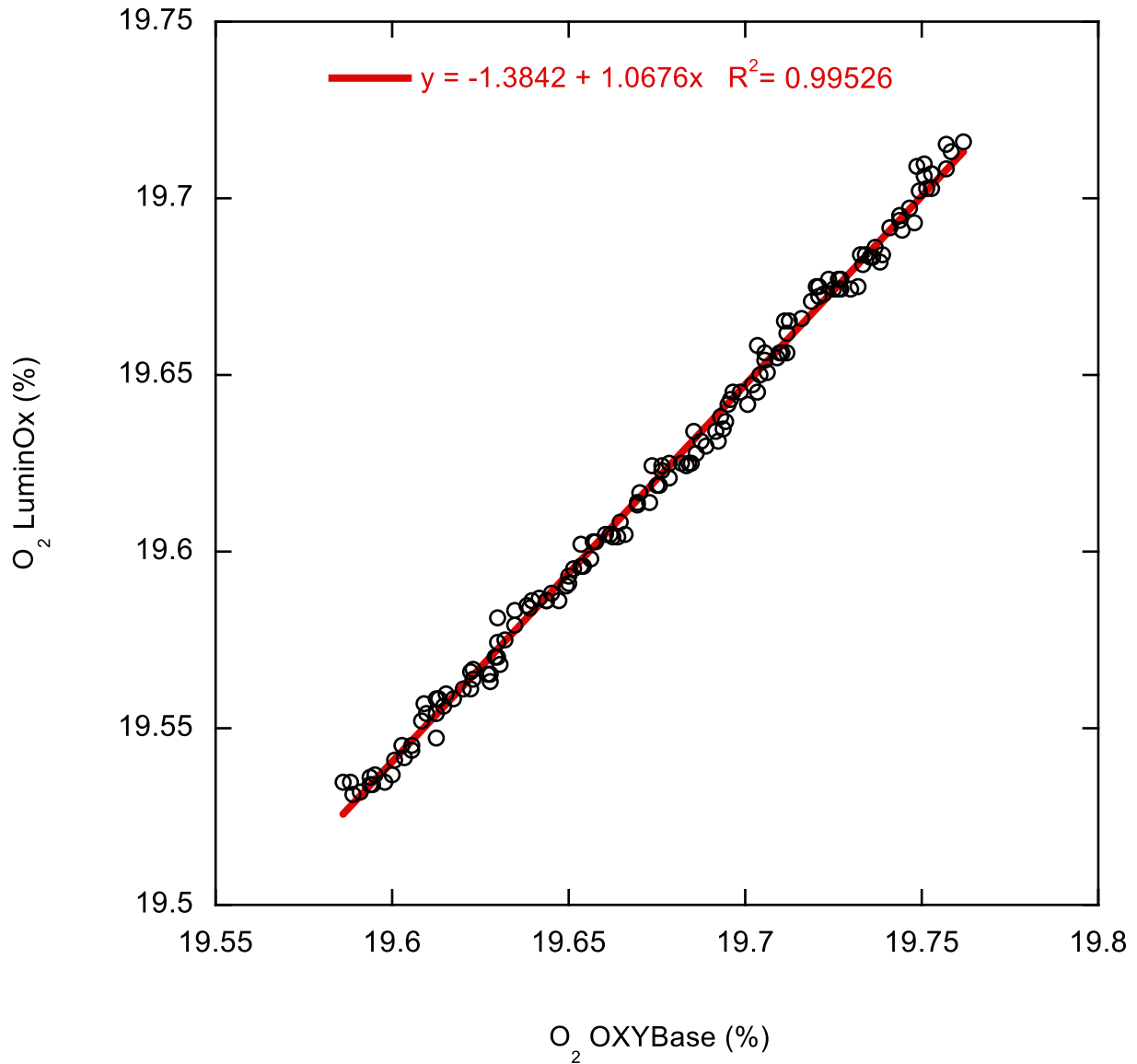
Figure 4014. Measured O 2 part with LuminOx versus O 2 measured with OXYBase during the respiration experience. The red solid line represents a linear regression.
