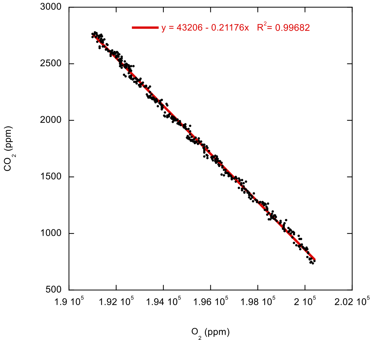
330 Figure 1418. CO 2 concentrations versus O 2 concentrations. The solid red line represents a linear regression.
