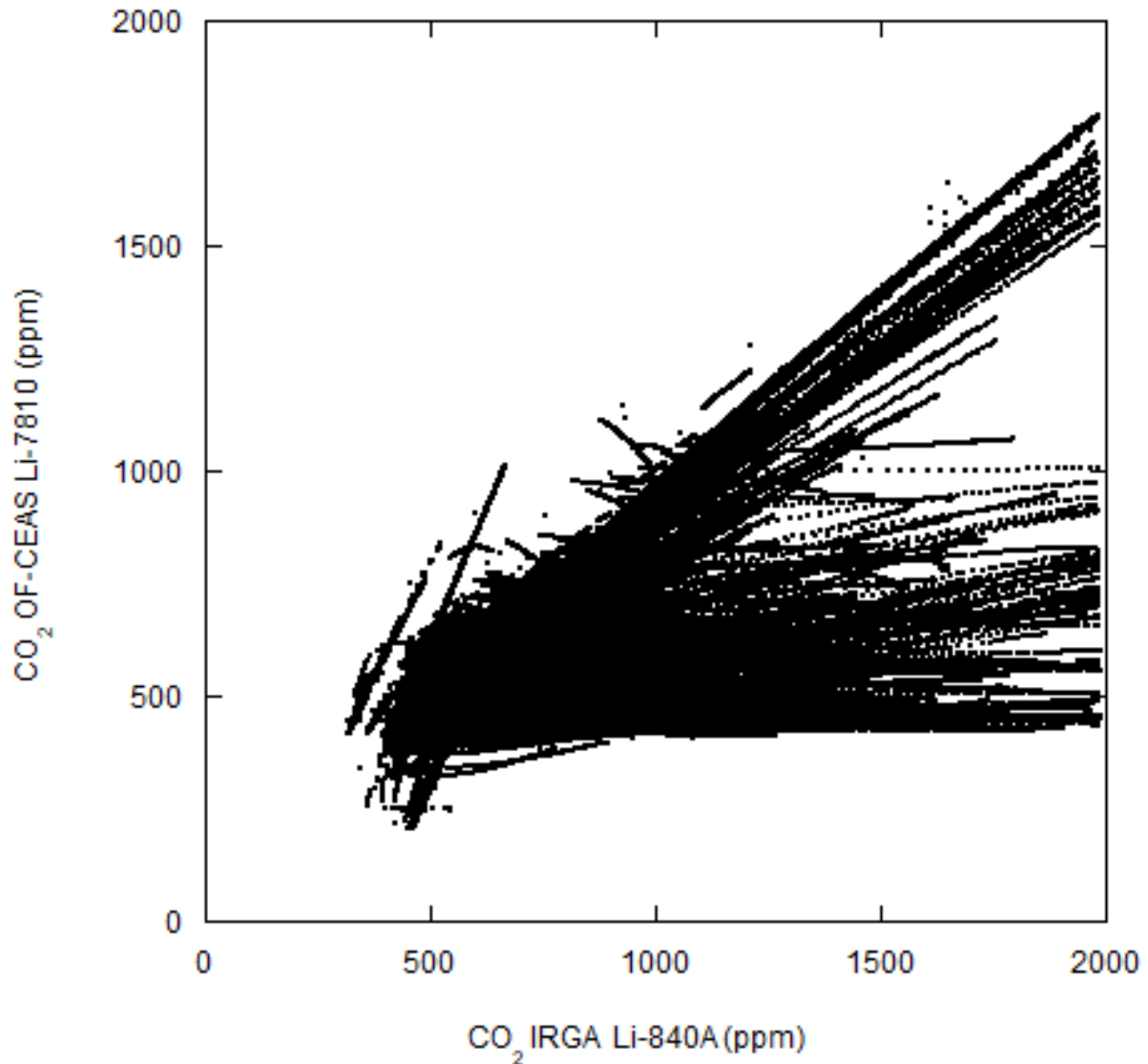
185 Figure 8. OF-CEAS Li-7810 measurements versus IRGA Li-840A measurements during three months. Li-840A derived during the test and presents measured CO 2 saturation for 2000 ppm due to the analog output configuration.
