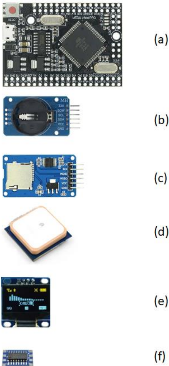
Figure 1. Data logger built with a) Arduino Mega Pro, b) RTC, c) \mu SD card reader, d) GPS, e) OLED display, f) RS232 to TTL module.
