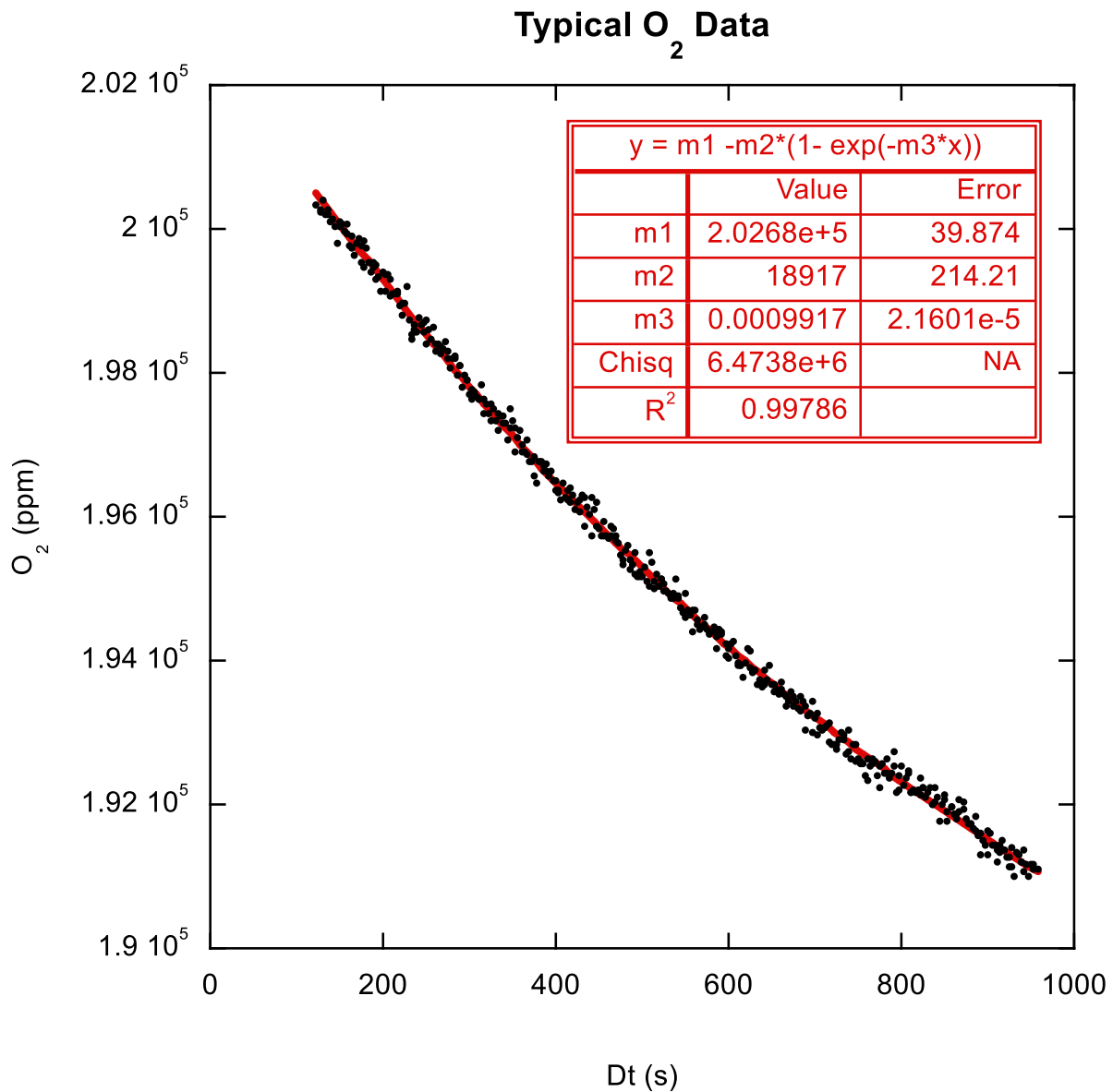
Figure 1317. Oxygen concentration measurement versus time. The solid red line represents an asymptotic regression.
