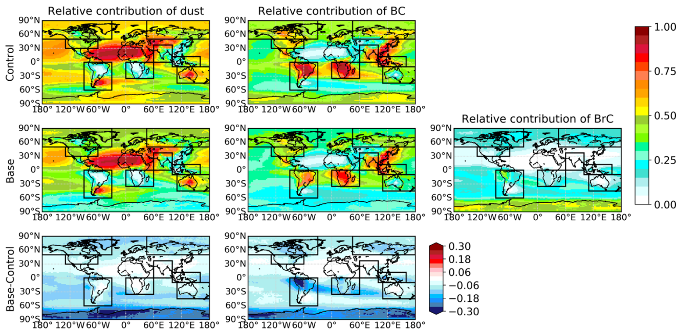
Figure 10. Average over the 2007-2016 period of ModelE light-absorbing dust (left), BC (middle), and BrC (right) contribution to total UV-VIS AAOD in control (top) and base (middle) simulations, with each BB region of interest, identified in Sect. 2.3.2, outlined in black. (Bottom) Difference in dust and BC contributions between base and control cases. Relative contribution of BrC in BB regions appears to come from a greater reduction in that of BC, rather than dust.
