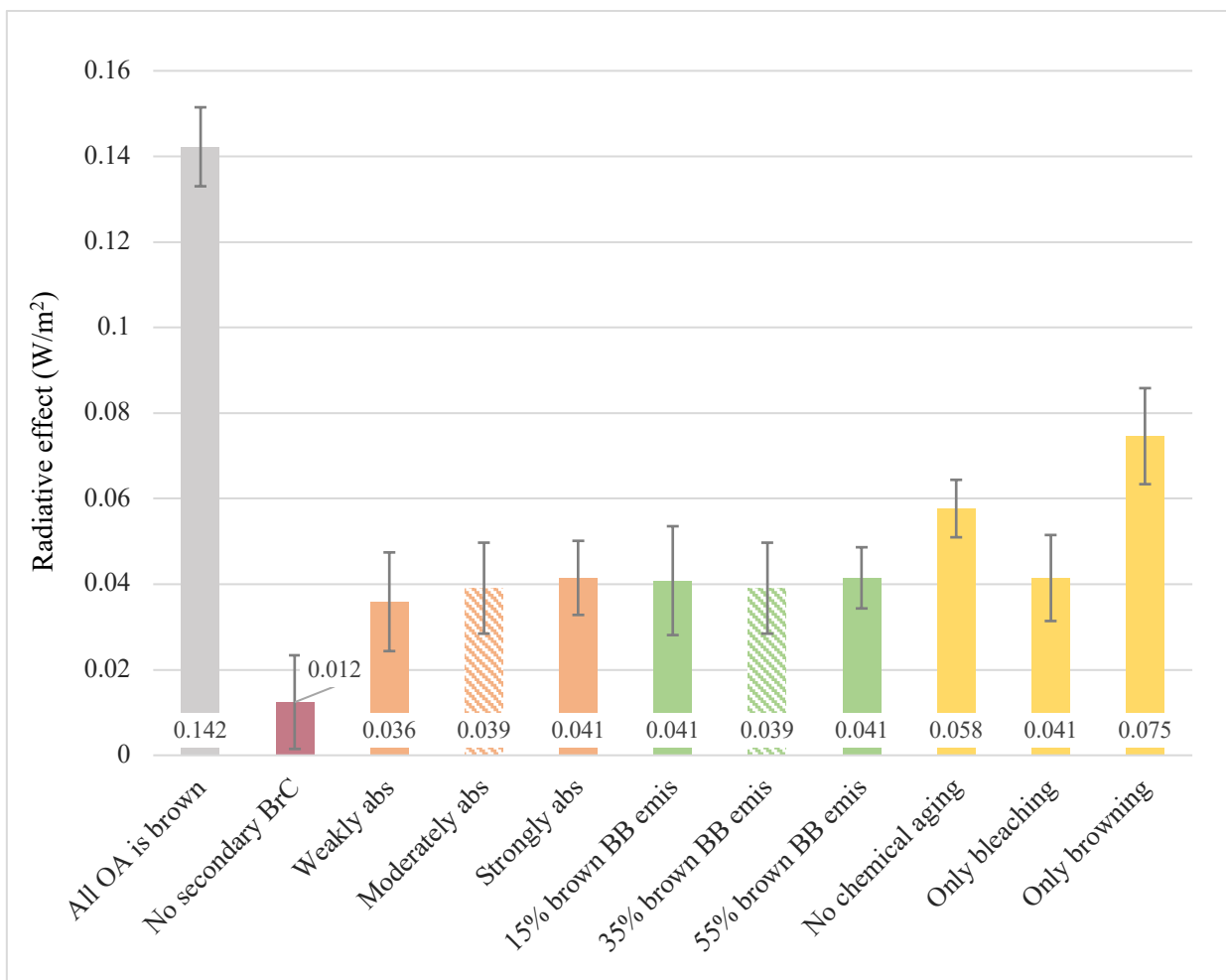
Figure 14. Global, annual average radiative effect of each BrC simulation, calculated according to equation 8. Error bars show the standard deviations, which can be interpreted as the variability of each simulation across repeated years of simulation. Different colored bars indicate a different BrC property varied, and dashed bars indicate the base case of BrC representation (this is shown twice for ease of comparison to other simulations), consistent with Figs. 7 and 8.
