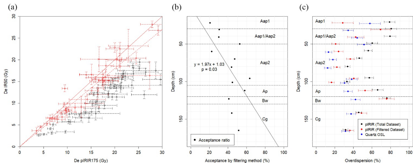
350 Figure 6: (a) Example of grains characterized as well-bleached (red) versus poorly bleached (black) through comparison between D_{e\text{ IRSL}} and D_{e\text{ pIRIR}} values for sample NCL-1117123. The solid diagonal line marks the 1:1 ratio between equivalent doses obtained from IRSL 50 and pIRIR 175 signals. The dashed diagonal line marks the 1:0.9 ratio adopted as a threshold to identify well-bleached grains. (b) Acceptance ratio indicating the percentage of well-bleached grains with depth. The line demonstrates the trend between the relationship between depth and acceptance ratio obtained by linear regression. (c) Comparison of relative overdispersion obtained from the total dataset of feldspar pIRIR 175 (black), filtered dataset of feldspar pIRIR 175 (red), and quartz OSL (blue). Note 355 that the points are slightly displaced vertically for visibility.
