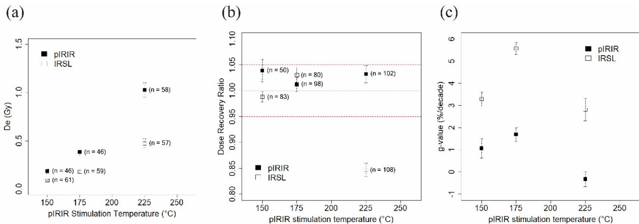
330 Figure 5 The results of (a) remnant dose after bleaching in a solar simulator; (b) dose recovery test; (c) fading rate with different preheat / stimulation temperatures. The tests were performed on samples NCL-1117023 and NCL-1117029 after bleaching in the SOL2 solar simulator for 48 hours. The number of grains used for the analyses is indicated next to each data point (a, b). Six aliquots were used for fading analyses for each pIRIR stimulation temperature (c).
