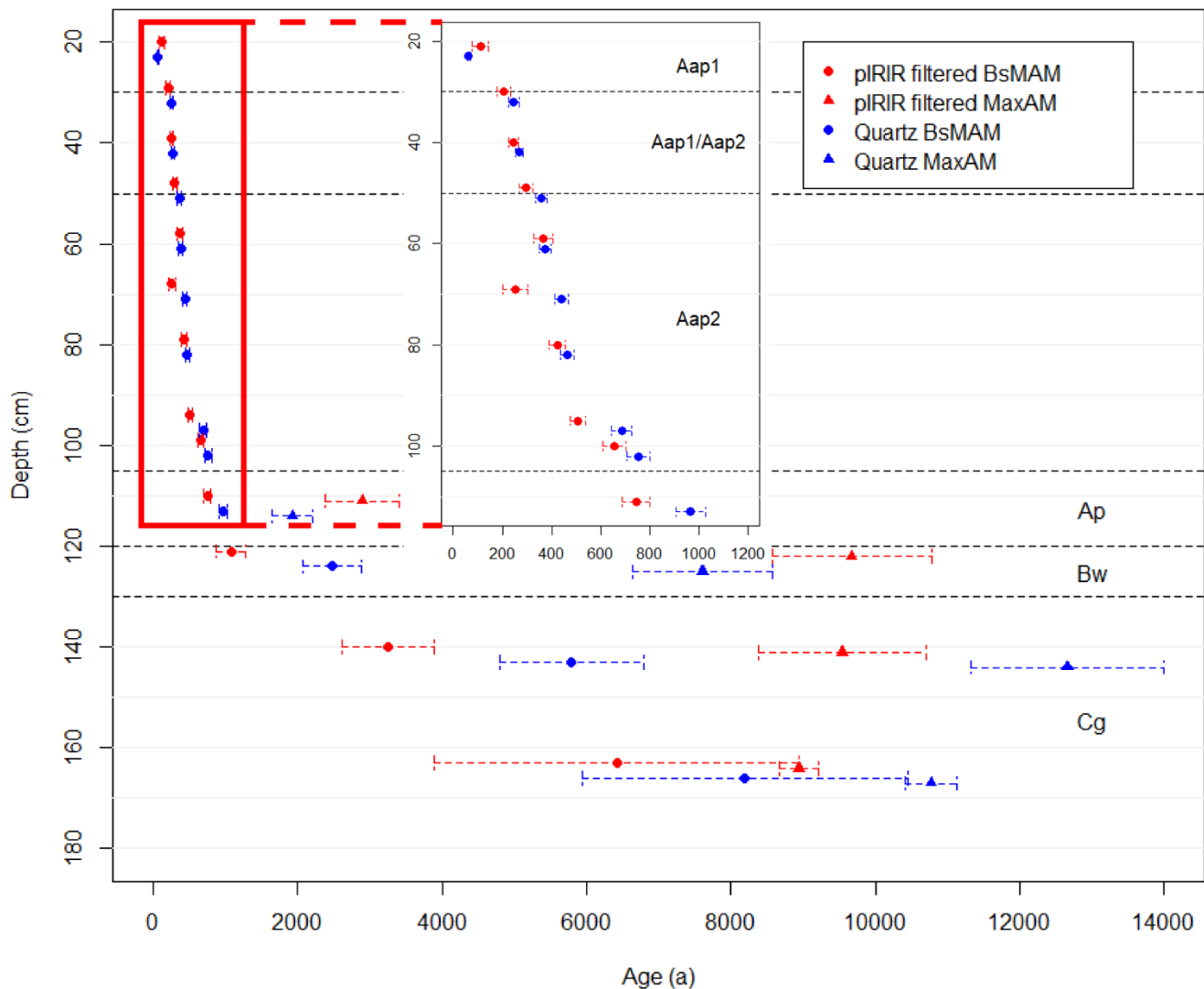
380 Figure 8: Comparison between ages obtained by applying BsMAM to multigrain quartz (blue) and filtered single-grain feldspar pIRIR 175 (red) D e datasets. Note that the points are slightly displaced from their original position (quartz – bottom; feldspar – top) for the sake of visibility.
