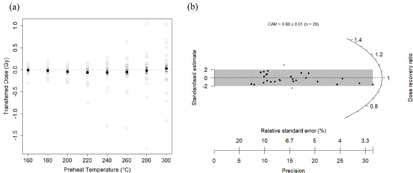
Figure 4: The results of (a) thermal transfer test; (b) dose recovery test on quartz samples from the Braakmankamp site.
