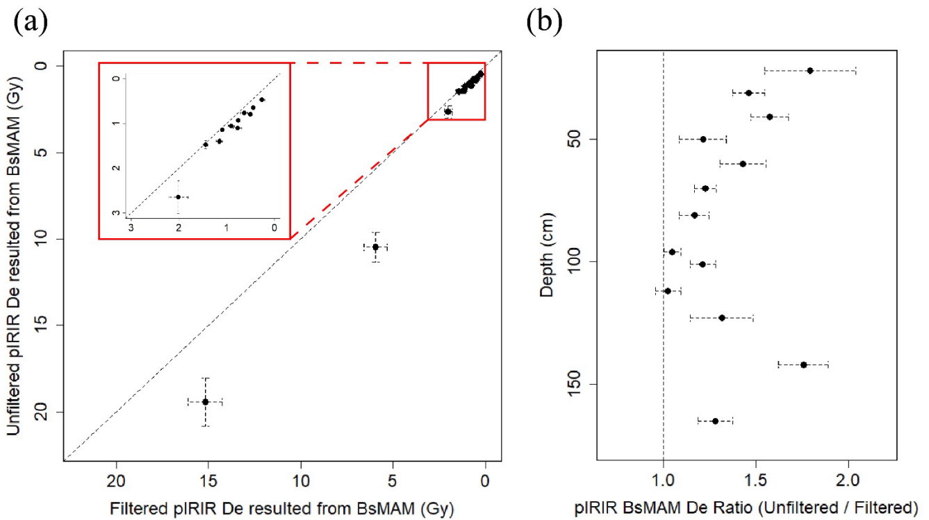
Figure 7: (a) Comparison of D_e obtained by applying BsMAM to the filtered pIRIR dataset and the unfiltered pIRIR dataset. The dotted diagonal line represents unity. (b) The comparison between depth and ratio obtained by dividing the D_e of the total pIRIR dataset by the D_e of the filtered pIRIR dataset. The dotted vertical line represents unity. The majority of the samples (11 out of 13) demonstrate smaller D_e when the filter is applied.
