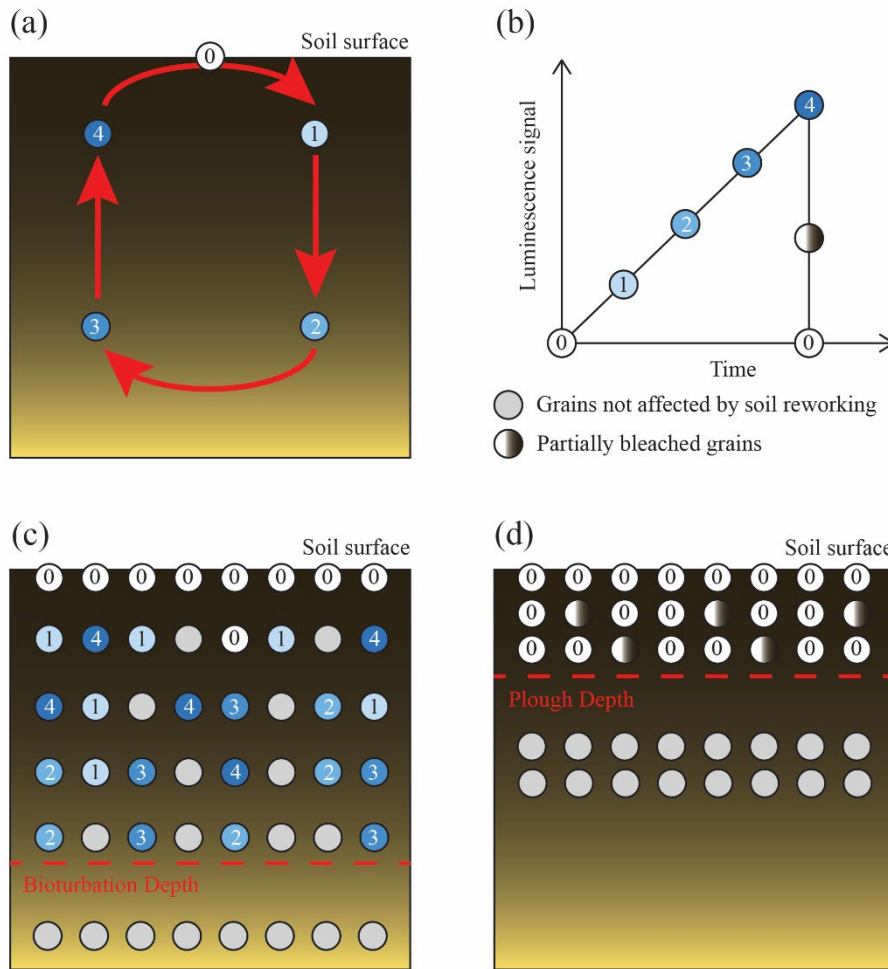
105 Figure 2: Conceptual diagrams illustrating the expected luminescence signals of grains experiencing soil reworking by agricultural activities and bioturbation, which (a) deliver grains from the surface to depth and from depth to the surface over time. (b) Luminescence signals accumulate with time while the grains are buried and are bleached by light exposure when the grains are at the surface position. While some grains may be fully bleached, others may be partially bleached if they are not sufficiently light- exposed at the soil surface. (c) Exposed scenario when grains are reworked by bioturbation, and (d) expected scenario when grains are reworked by agricultural activities, mainly ploughing. The soil reworking process by bioturbation is relatively slow compared to ploughing, so bioturbated grains may spend more time at the surface than sediments. Bioturbation is also less intense and can reach a greater depth than ploughing. This may result in greater heterogeneity in the equivalent doses of well-bleached bioturbated grains at a given depth. In contrast, ploughed grains are more likely homogenised by the intense mixing process and exhibit less heterogeneity in the equivalent doses of the well-bleached grains.
