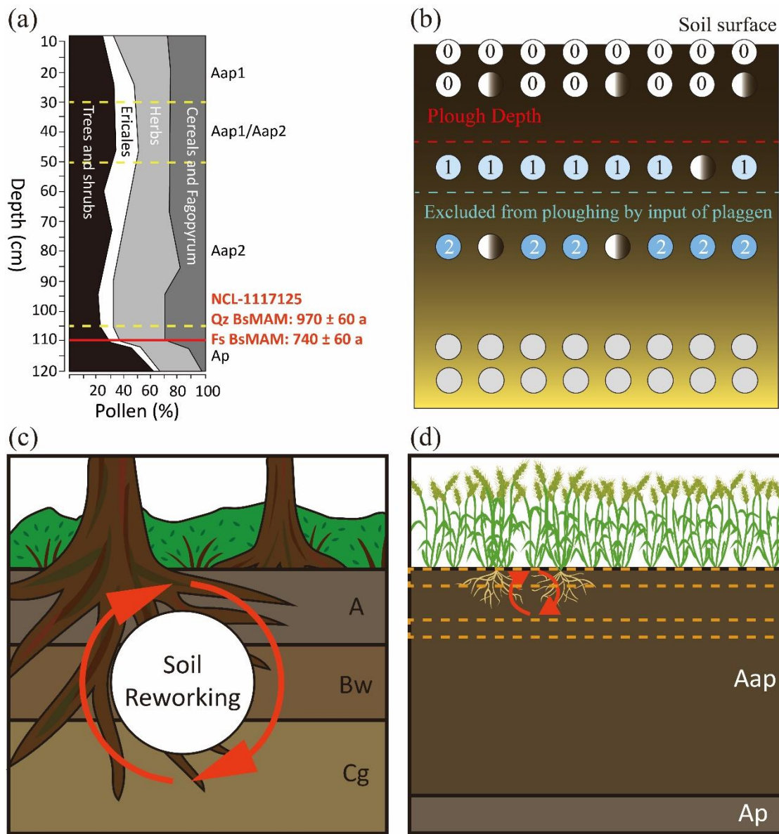
Figure 9: (a) Simplified pollen analysis result of Braakmankamp from Smeenge (2020). A sharp decrease in trees and shrubs coincides with the increase in herbs, cereals, and Fagopyrum. (b) A conceptual diagram illustrating the expected luminescence signals of grains within the plaggen layer at Braakmankamp (see Fig. 2 for symbol reference). While the topsoil is continuously reworked by ploughing, a certain depth of the soil layer is excluded from the soil reworking by accretion of plaggen, creating a series of layers with grains of a certain age range. (c) Possible scenario of soil reworking before the introduction of plaggen agriculture at Braakmankamp. The deeper soil food chain, mainly deep-rooted trees, moves the grains from the surface to relatively deep layers. (d) Possible scenario of soil reworking after the introduction of plaggen agriculture at Braakmankamp. The decrease of the depth affected by the soil food chain, due to cereals and herbs with shallower roots and the decrease of soil fauna dependent on deep roots, cause decreased movement of grains. Also, the yearly addition of plaggen materials (indicated by the dashed box) results in previous deposits being excluded from the soil reworking process.
