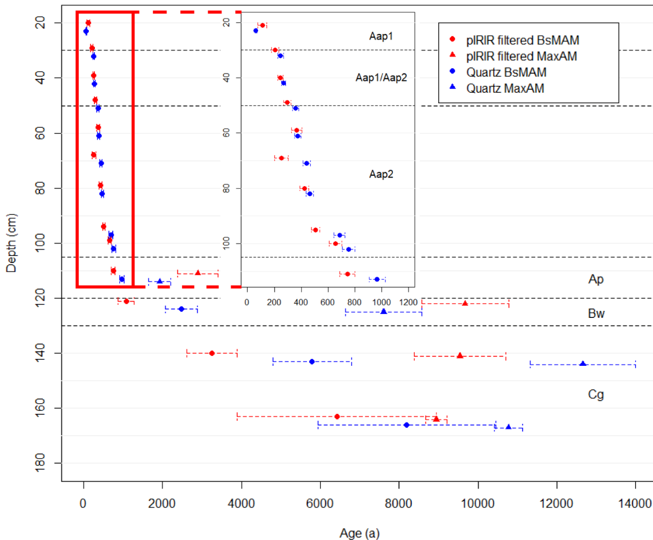
425 Figure 8: Comparison between ages obtained by applying BsMAM to multigrain quartz (blue) and filtered single-grain feldspar pIRIR 175 (red) D e datasets. Note that the points are slightly displaced from their original position (quartz – bottom; feldspar – top) for the sake of visibility.
