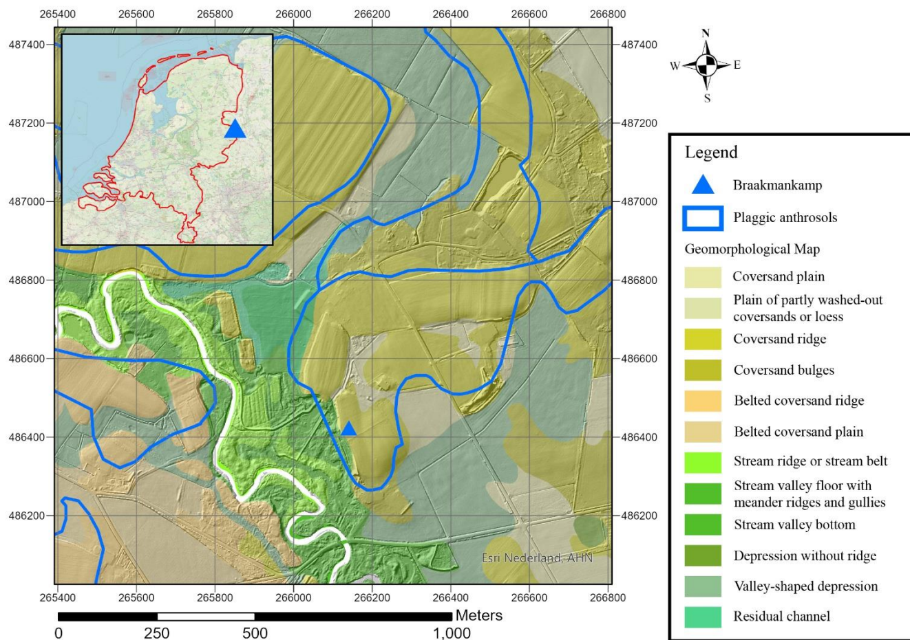
Figure 32: The location of the Braakmankamp site on the geomorphological map of the Netherlands (BRO, 2023). Plaggic anthrosols occur mostly in areas with coversand deposition. The projected coordinate system is Amersfoort / RD New (EPSG:28992).
