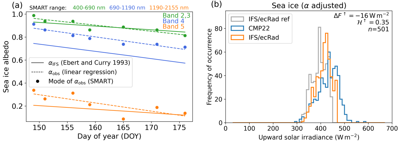
Figure 3. (a) Time series of modes of measured sea ice albedo in the 400-690 nm, 690-1190 nm and 1190-2155 nm band and IFS sea ice albedo climatology. The dashed lines show the parameterization for the measurements. (b) Distribution of upward solar irradiances for above Polar 5 cloud-free scenes above sea ice measured by the CMP22 (blue) and simulated by ecRad with the adjusted sea ice albedo (orange) together with the reference simulations (grey).
