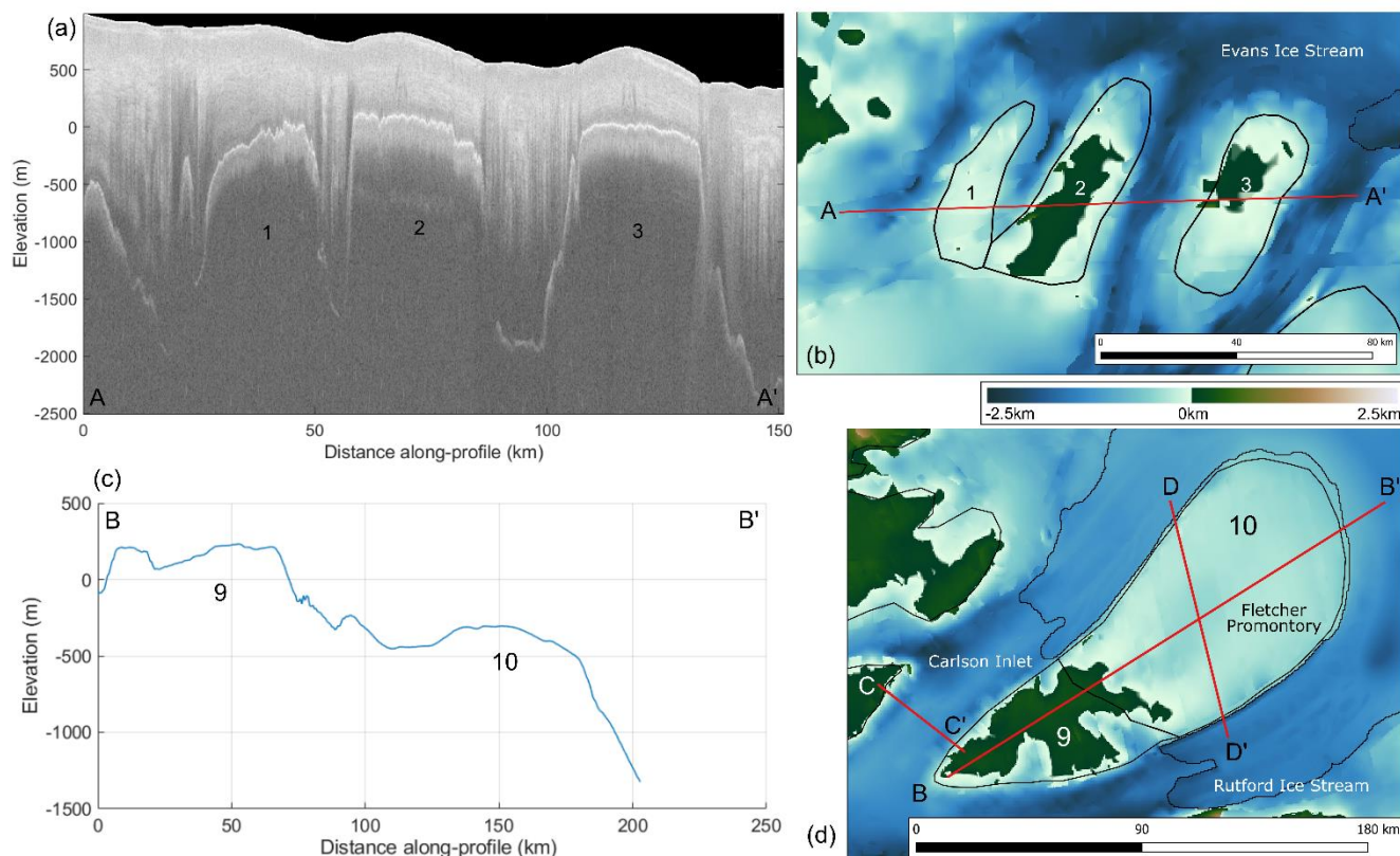
Figure 6: (a) Radargram illustrating plateau surfaces 1-3 along profile A-A'. (b) Profile line (A-A', displayed in red) over plateau surfaces 1-3. (c) Interpolated elevations from BedMachine subglacial topography data (Morlighem et al., 2020) along profile B-B'. BedMachine data were used for this profile as there were no directly overflown flightlines from the GRADES-IMAGE RES survey. (d) Profile line (B-B', displayed in red) over the Fletcher Promontory, plateau surfaces 9 and 10. Profile lines C-C' and D-D' illustrate the locations of radargrams in Figures 7 and 9.
