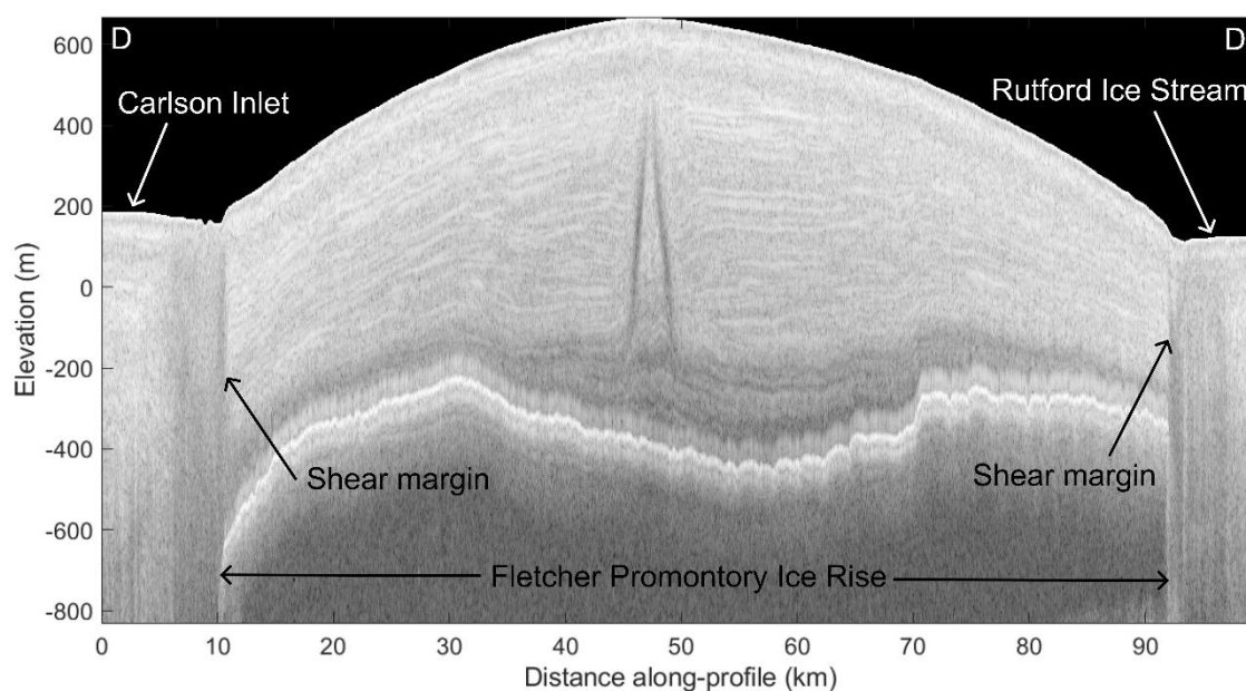
Figure 9: Radargram illustrating continuous undisturbed layering overlying the Fletcher Promontory flat surface. Location of D-D' profile line is illustrated in Figure 6d. The centre of Fletcher Promontory demonstrates a well-developed Raymond Bump, indicating an ice-divide triple junction (Hindmarsh et al., 2011).
