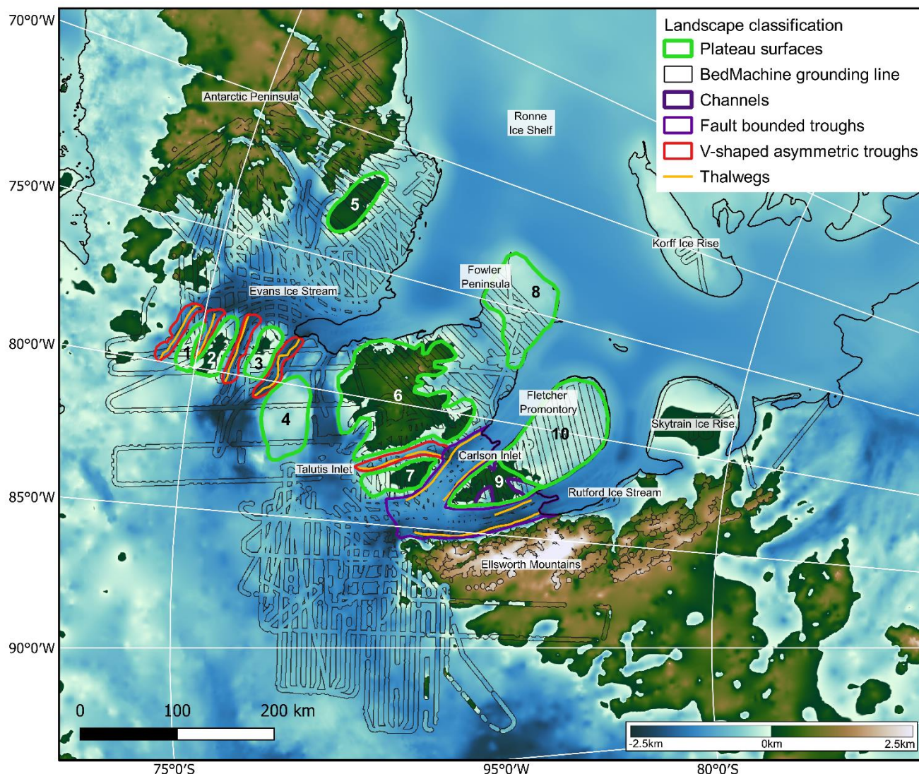
250 Figure 5: Regional subglacial topography of the Evans-Rutford region. The background is BedMachine (Morlighem et al., 2020) but with our interpolated radar lines (outlined in black) of the Evans-Rutford region surveys overlain, along with mapped plateau surfaces and troughs.
