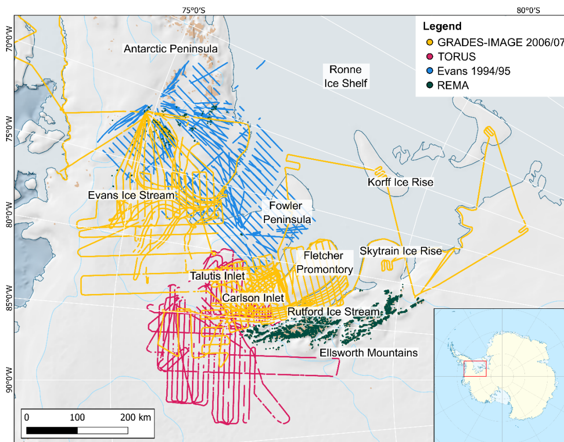
Figure 1: Study site map of the Evans-Rutford region. Data points illustrate the RES surveys used in the study: GRADES-IMAGE 2006/07 carried out by British Antarctic Survey (BAS), TORUS, REMA exposed bedrock, and Evans 1994/95. Detailed basemap sourced from Quantarctica (Matsuoka et al., 2021). Inset map shows location of the study region in relation to the Antarctic continent (red box).
