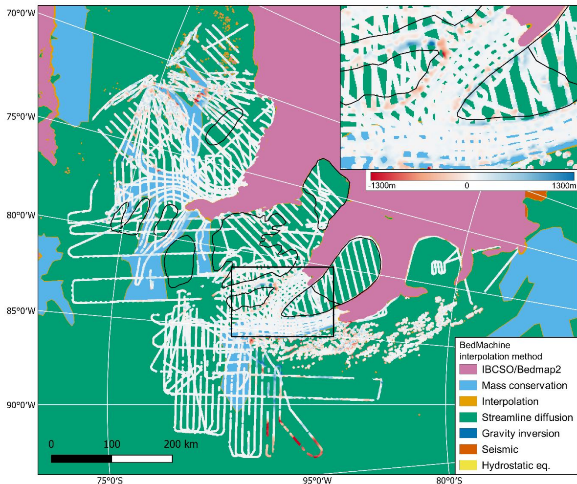
Figure 4. Difference between BedMachine bed elevation and our picked bed elevation radar line data from GRADES, TORUS and Evans surveys. Legend shows different interpolation methods used in compiling the BedMachine topography (Morlighem et al., 2020). Black line illustrates the grounding line derived from BedMachine (Morlighem et al., 2020). Colour ramp shows the difference between BedMachine and our picked line data. Reds show areas where Bedmachine topography is lower, blues where BedMachine is higher. Inset shows detail of mid-Rutford and Carlson Inlet. The biggest differences occur around the edges of plateaus and troughs and in the area of the TORUS survey. Inspection of individual radargrams shows that prominent breaks in topography are smoothed in BedMachine and so we use our line data in our analysis.
