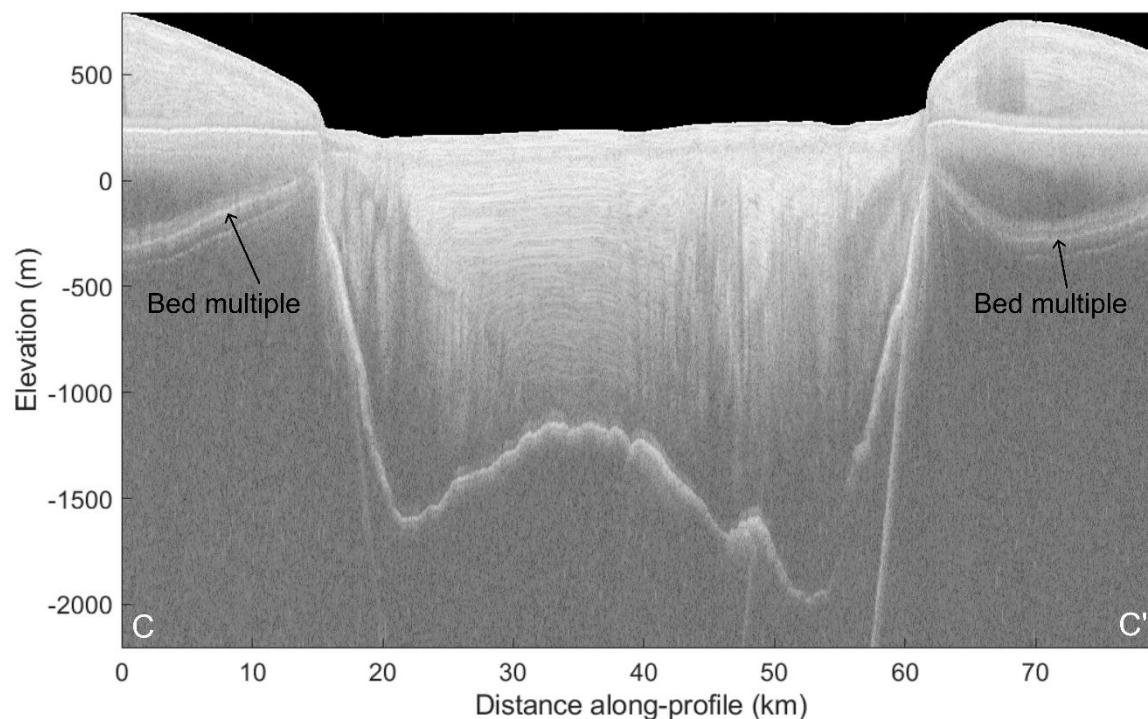
Figure 7: Radargram demonstrating the W-shaped cross-profile in the Carlson Inlet trough. Location of C-C' profile line is illustrated in Figure 6d. Bed multiples are due to an additional reflection between initially transmitted radar wave with ice surface and the aircraft. 280
