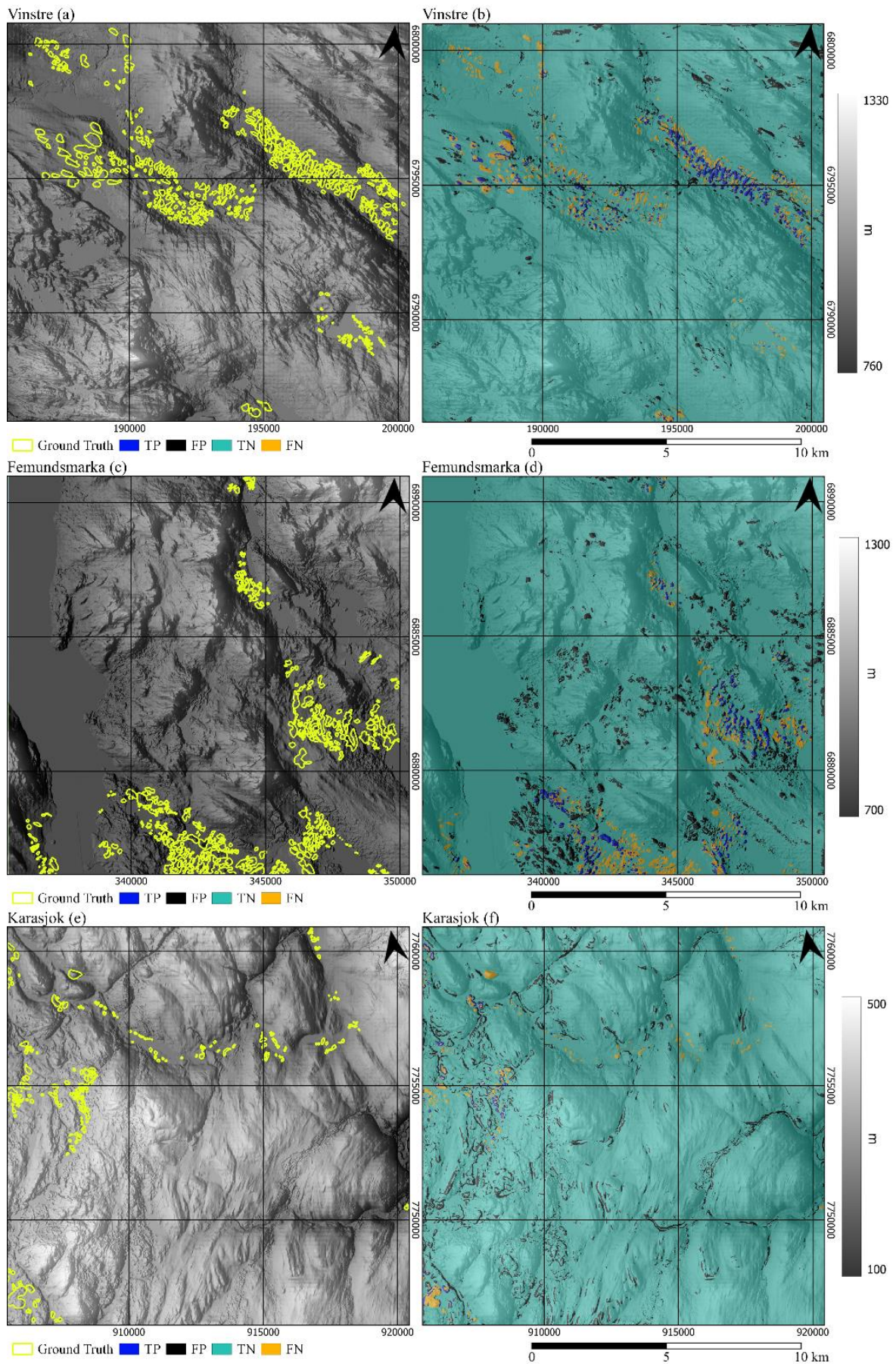
Figure 6: Comparison of input to output in the three study regions. (a, c, e) show ground truth data, while (b, d, f) show accuracy maps denoting confusion matrix (Fig. 5) values for the clustered output of the KM method. Outputs are superimposed on a hillshade of the input DEMs (Kartverket, 2021b).
