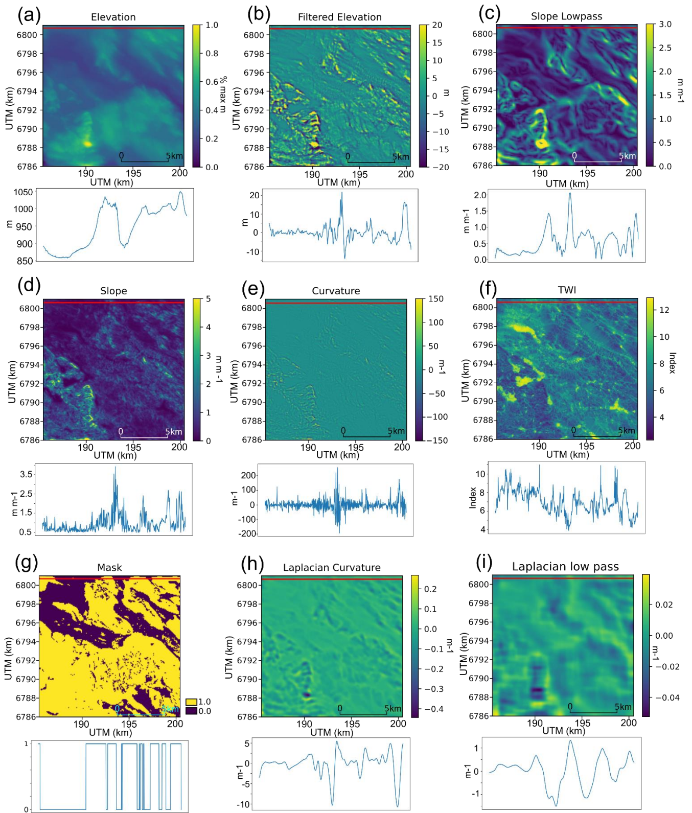
Figure 4: Illustration of morphometrics used in this study, with red line indicating the transect taken for subchart figures. (a) to (f) show clustering values, whilst (g) to (i) show masking values. (a) Shows elevation from the 1 m resampled to 10 m DEM data (Kartverket, 2021), (b) shows elevation with km-scale features filtered out, (c) shows the output of the general slope (low frequency slope) filter, (d) shows the local slope values used for clustering, (e) shows curvature values used for clustering, (f) shows topographic wetness index (TWI), (g) shows masking values used for excluding regions where ribbed moraine cannot form, (h) shows curvature derived from a laplacian of gaussian filtered DEM for masking mountain peaks (i) shows a similar plot at 1 km resolution for excluding large wavelength features.
