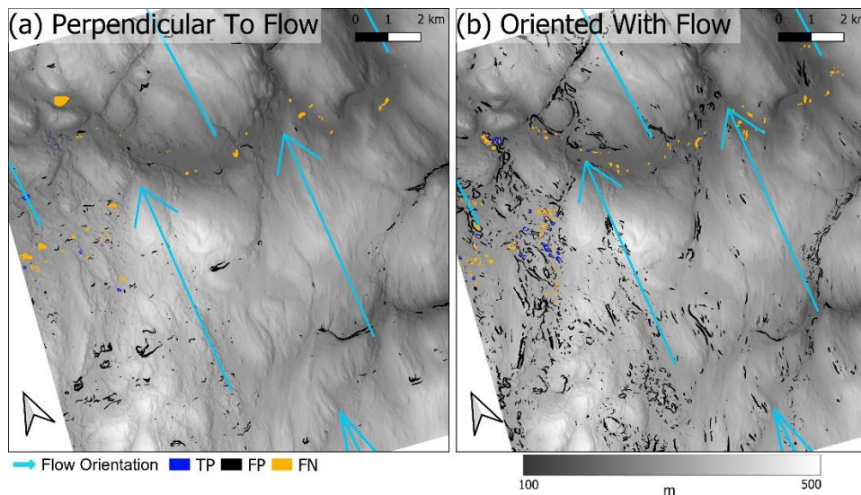
510 Figure 8: Detected features versus LGM ice flow direction in the Karasjok region. (a) shows values \pm 25^\circ from orientation perpendicular to mean flow direction (blue arrows) during the FIS (Fennoscandian Ice Sheet) (Patton et al., 2016; 2017) and (b) shows values not oriented perpendicular to average flow angle during FIS (Patton et al., 2016; 2017). Both figures superimposed on 10 m DEM and hillshade (Kartverket, 2021b).
