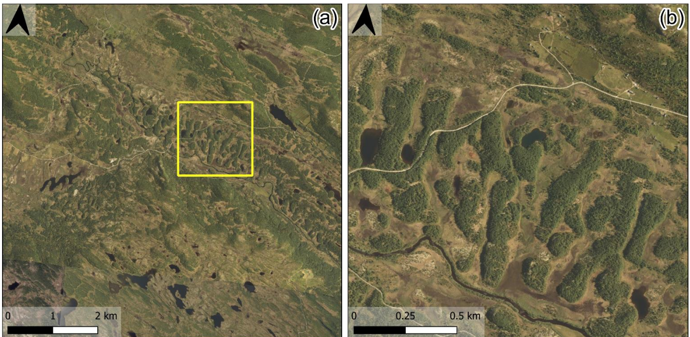
90 Figure 1: Aerial imagery of ribbed moraine at the Vinstre study area site (Fig. 3d) with (a) showing a general overview, and (b) showing a close-in view of ribbed moraine landforms. Ribbed moraine at this site appear to be partially anastomosed and form in a linear track (Dunlop & Clark, 2006). Aerial imagery from Norwegian national mapping data (Kartverket, 2021a, c).
