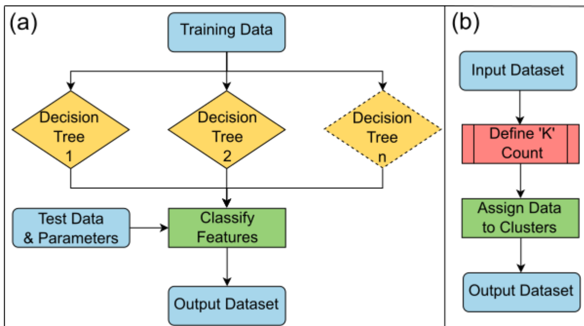
Figure 3: Flowcharts describing (a) the basic principles behind the RF algorithm. (b) The basic principles behind the operation of a KM methodology. The model is first run to determine the number of K points required to represent the input data, and then run a second time to produce an output.
