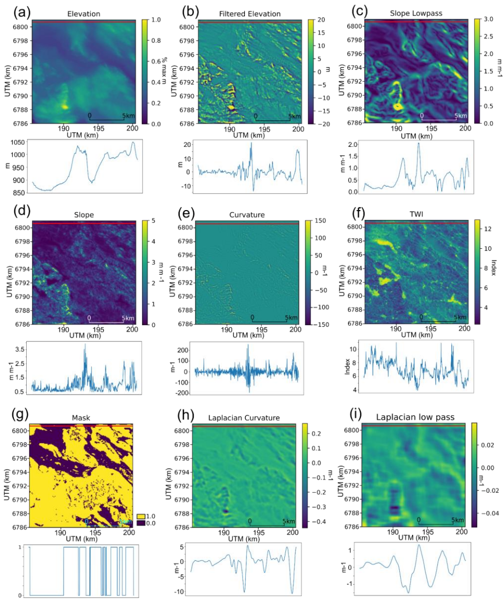
250 Figure 43: Illustration of morphometrics used in this study, with red line indicating the transect taken for subchart figures. (a) to (f) show clustering values, whilst (g) to (i) show masking values. (a) Shows elevation from the 1 m 255 resampled to 10 m DEM data (Kartverket, 2021), (b) shows elevation with km-scale features filtered out, (c) shows the output of the general slope (low frequency slope) filter, (d) shows the local slope values used for clustering, (e) shows curvature values used for clustering, (f) shows topographic wetness index (TWI), (g) shows masking values used for excluding regions where ribbed moraine cannot form, (h) shows curvature derived from a laplacian of gaussian filtered DEM for masking mountain peaks (i) shows a similar plot at 1 km resolution for excluding large wavelength features. 2.5 Comparative Analysis
