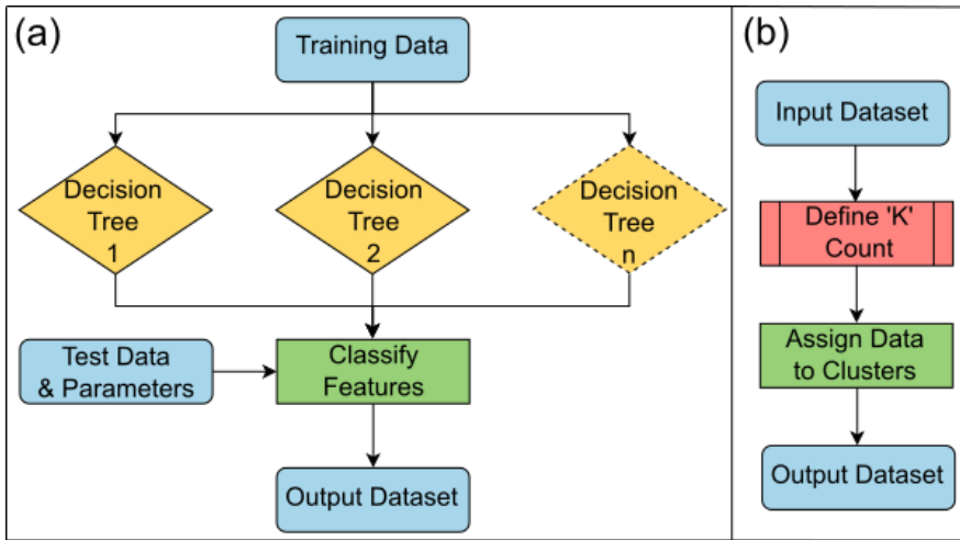
Figure 32: Flowcharts describing (a) the basic principles behind the RF algorithm. (b) The basic principles behind the operation of a KM methodology. The model is first run to determine the number of K points required to represent the input data, and then run a second time to produce an output.
