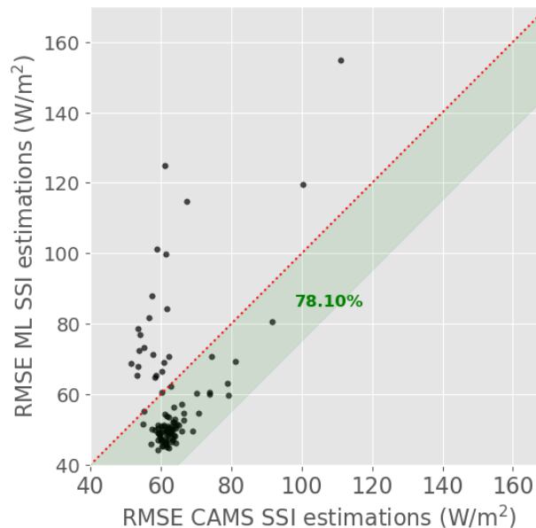
Figure 10. Comparison of RMSE of ML model (training setup 3-4) and CAMS for each station. The green band indicates for which stations ML model outperforms CAMS; the percentage of such station is indicated in bold green.
