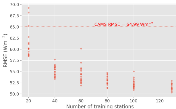
Figure 9. Test RMSE as a function of the number N of stations used for the training with 20 random picks of N among 129 (training setup 23 ).
