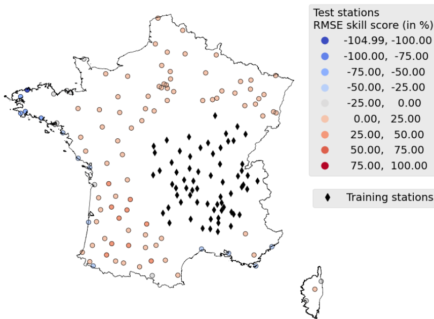
Figure 11. Geographical distribution of the RMSE skill score of ML model in training setup 3-4. Positive values show the stations where ML model outperforms CAMS.
