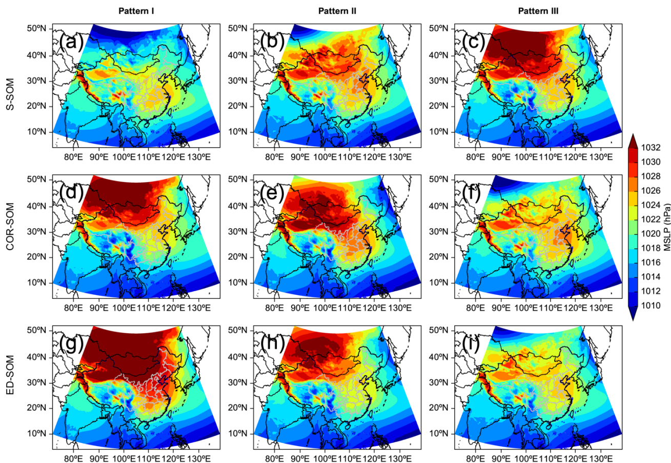
Figure 4: Spatial distributions of three weather patterns for MSLP (Mean Sea Level Pressure) identified by S-SOM (a, b and c), COR-SOM (d, e, and f), and ED-SOM (g, h, and i) during the first two months from 2015 to 2020.
