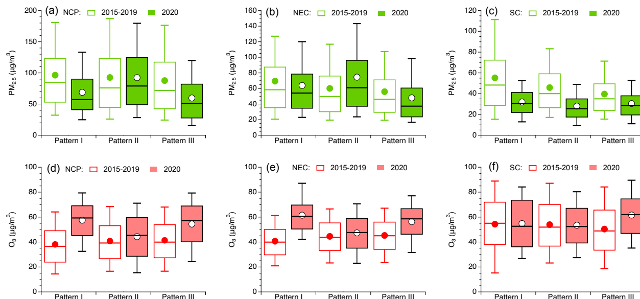
295 Figure 10: Comparisons of PM 2.5 (green colour) and O 3 (red colour) between days in 2020 (filled whisker-boxes) and in 2015-2019 (hollow whisker-boxes) for the three weather patterns in NCP (a and d), NEC (b and e), and SC (c and f).
