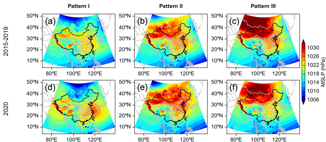
Figure 6: Comparison of the three weather patterns between days in 2020 (d, e, and f) and 2015-2019 (a, b, and c), respectively.
