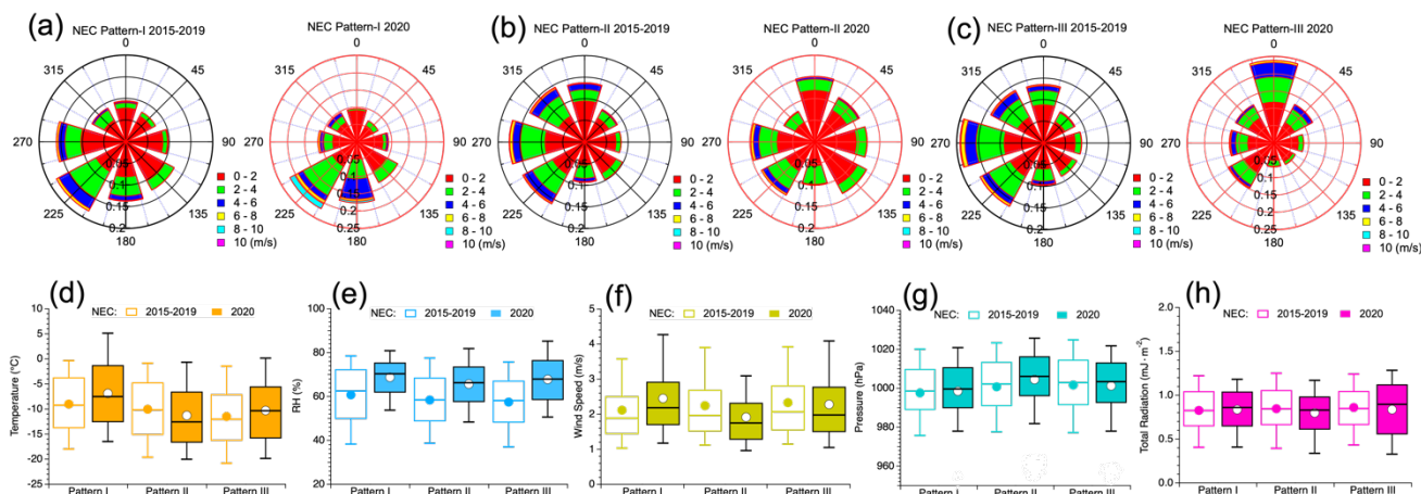
Figure 8: Comparisons of different weather factors (including Wind Speed, Wind Direction, Temperature, Relative Humidity, Pressure, and Total Radiation) between days in 2020 (red rings and solid whisker-boxes) and in 2015-2019 (black rings and hollow whisker-boxes) for the three weather patterns in NEC.
