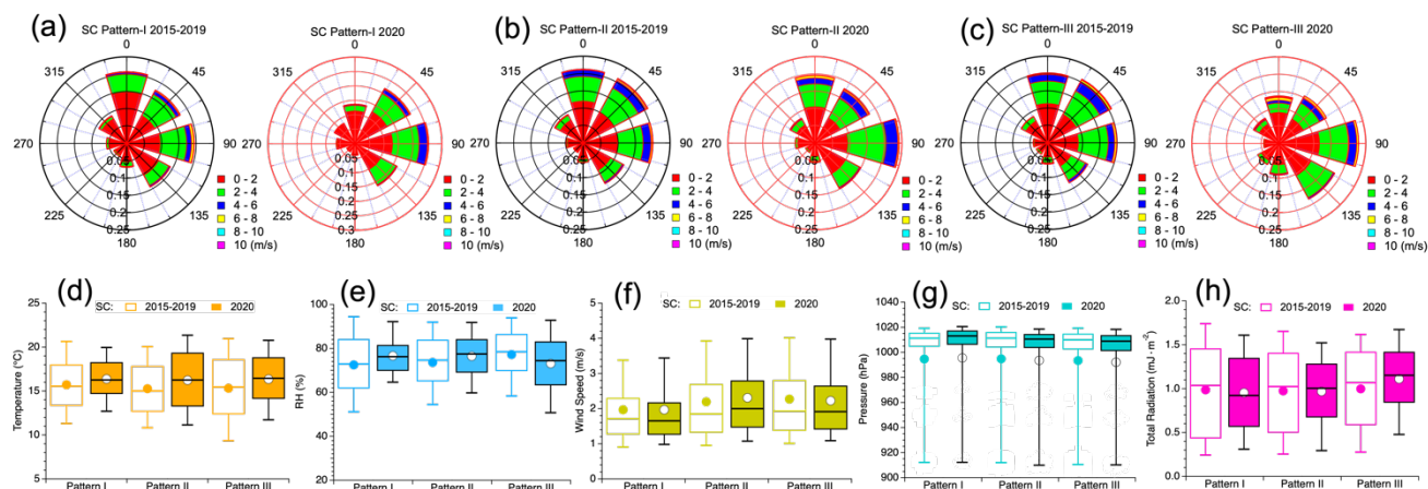
Figure 9: Comparisons of different weather factors (including Wind Speed, Wind Direction, Temperature, Relative Humidity, Pressure, and Total Radiation) between days in 2020 (red rings and solid whisker-boxes) and in 2015-2019 (black rings and hollow whisker-boxes) for the three weather patterns in SC.
