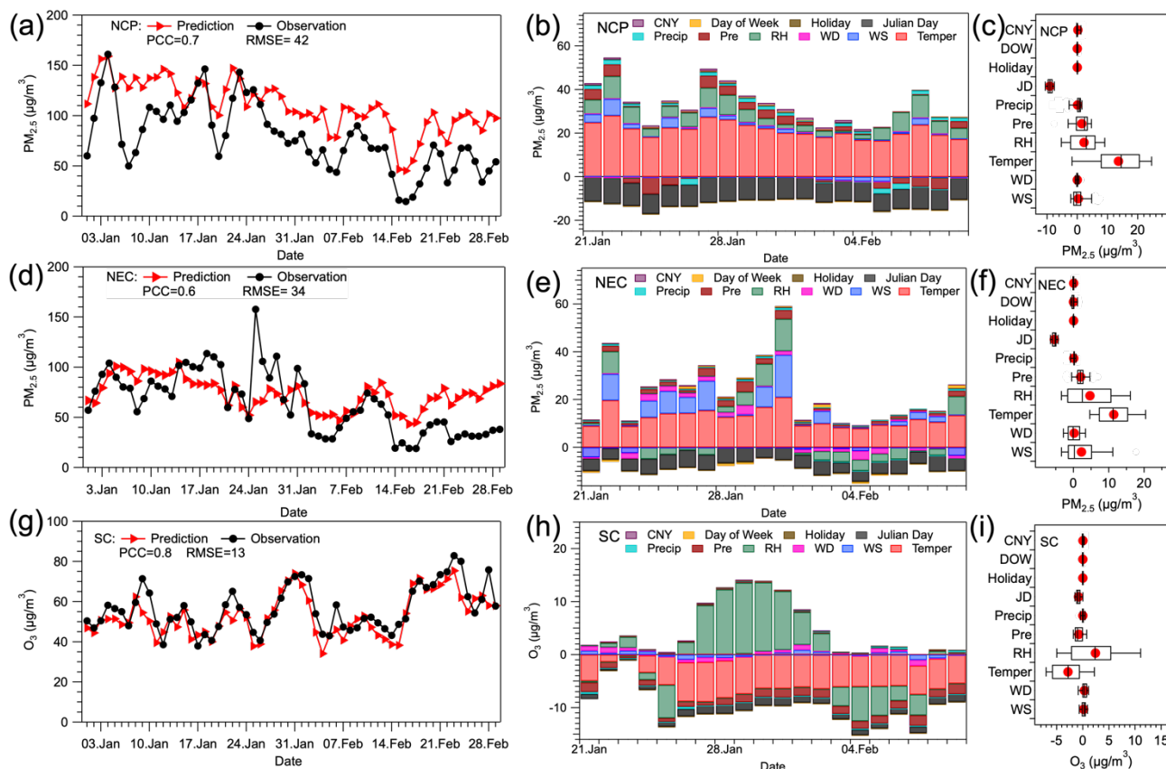
345 Figure 11: Time series comparisons between observations (black dot line) and predictions (red triangle line) combined with the contributions from the input variables (colourful bar) to the PM 2.5 and O 3 changes in NCP (a and b), NEC (d and e), and SC (g and h) respectively. Note that the whisker-box plots represent the mean importance of the input variables during the prediction in NCP (c), NEC (f), and SC (i) respectively
