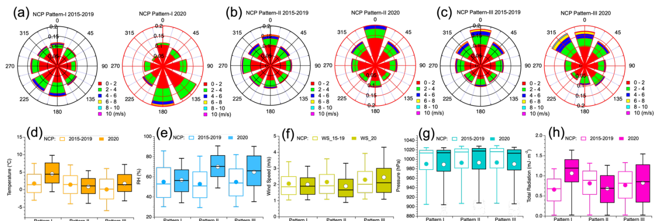
Figure 7: Comparisons of different weather factors (including Wind Speed, Wind Direction, Temperature, Relative Humidity, Pressure, and Total Radiation) between days in 2020 (red rings and solid whisker-boxes) and in 2015-2019 (black rings and hollow whisker-boxes) for the three weather patterns in NCP.
