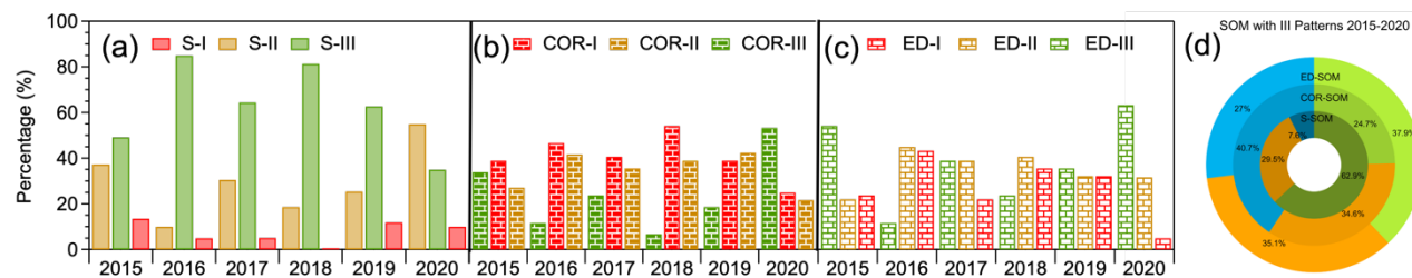
Figure 5: Cluster size distributions identified by S-SOM (inner ring), COR-SOM (middle ring) and ED-SOM (outer ring) over the years 2015-2020 (d) and days in each year (a: S-SOM; b: COR-SOM; c: ED-SOM).
