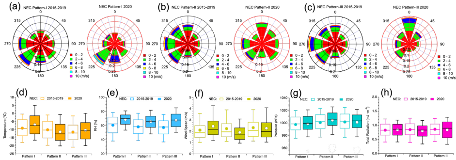
Figure 8: Comparisons of different weather factors (including Wind Speed, Wind Direction, Temperature, Relative Humidity, Pressure, and Total Radiation) between cluster days in 2020 (red rings and solid whisker-boxes) and in 2015-2019 (black rings and hollow whisker-boxes) for the three weather patterns in NEC.
