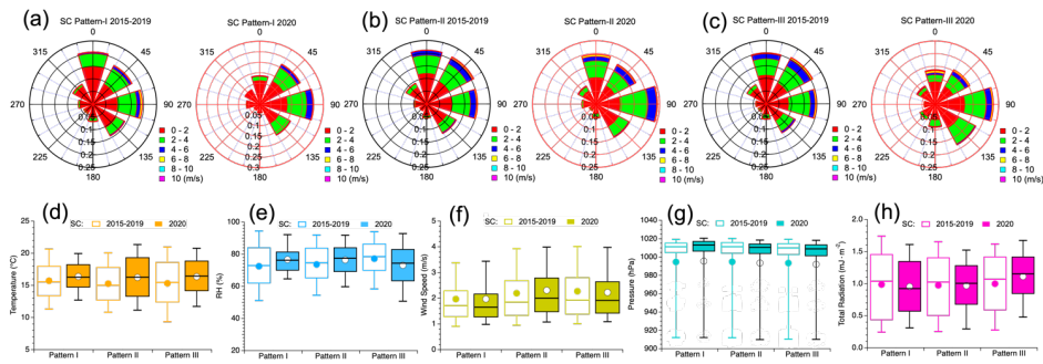
Figure 9: Comparisons of different weather factors (including Wind Speed, Wind Direction, Temperature, Relative Humidity, Pressure, and Total Radiation) between cluster days in 2020 (red rings and solid whisker-boxes) and in 2015-2019 (black rings and hollow whisker-boxes) for the three weather patterns in SC.
