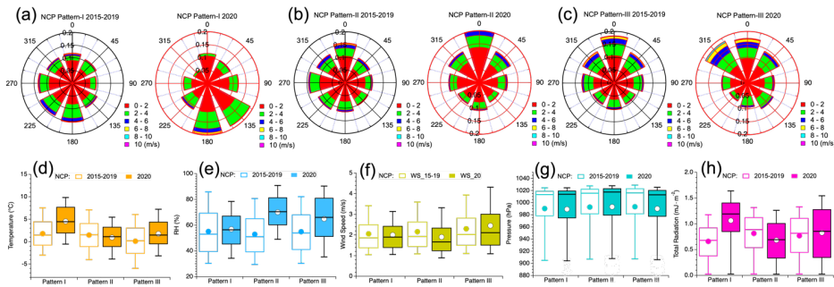
Figure 7: Comparisons of different weather factors (including Wind Speed, Wind Direction, Temperature, Relative Humidity, Pressure, and Total Radiation) between cluster days in 2020 (red rings and solid whisker-boxes) and in 2015-2019 (black rings and hollow whisker-boxes) for the three weather patterns in NCP.
