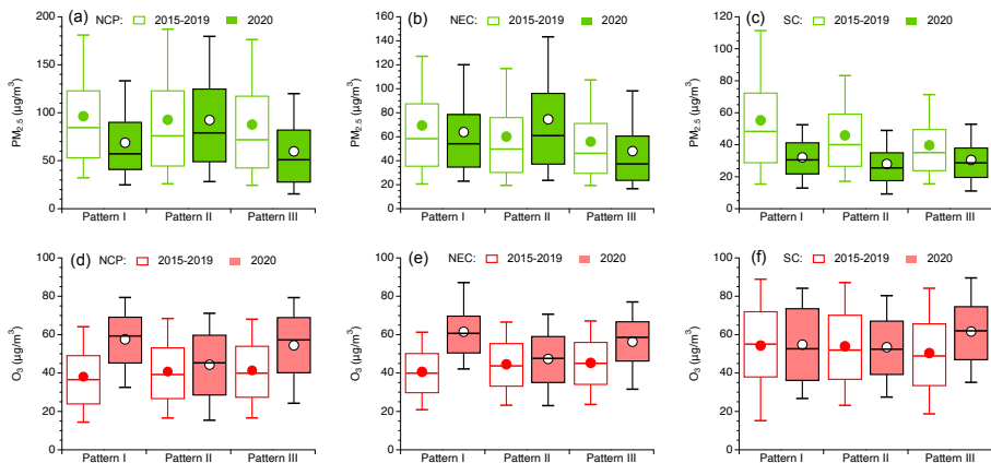
β65 Figure 10: Comparisons of PM 2.5 (green colour) and O 3 (red colour) between cluster days in 2020 (filled whisker-boxes) and in 2015-2019 (hollow whisker-boxes) for the three weather patterns in NCP (a and d), NEC (b and e), and SC (c and f).
