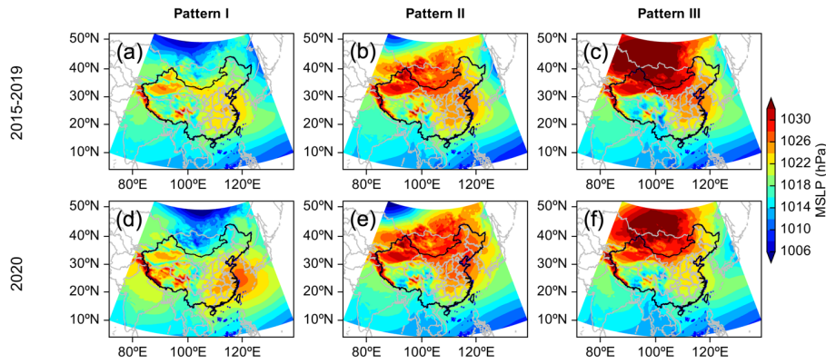
Figure 6: Comparison of the three weather patterns between cluster days in 2020 (d, e, and f) and 2015-2019 (a, b, and c), respectively.
