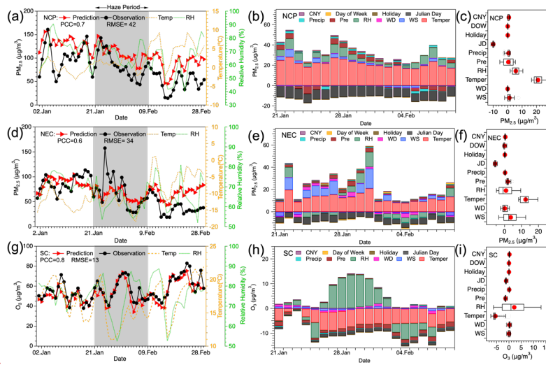
Figure 11: Time series comparisons between observations (black dot line) and predictions (red triangle line) combined with the SHAP values of the input variables (colourful bar) for the \text{PM}_{2.5} and \text{O}_3 predictions in NCP (a and b), NEC (d and e), and SC (g and h) respectively. Note that the whisker-box plots represent the mean SHAP value of the input variables during the prediction in NCP (c), NEC (f), and SC (i) respectively and shaded areas (a, d, g) indicates the haze event period.
