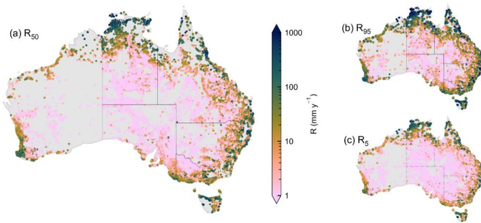
Figure 3. Groundwater recharge rates ( R ; \text{mm y}^{-1} ) estimated using CMB from 98,568 bores. Maps show: (a) median recharge ( R_{50} ), (b) 95 th percentile recharge ( R_{95} ) and (c) 5 th percentile recharge ( R_5 ) rates.
