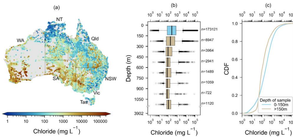
Figure 1. Spatial distribution of groundwater chloride ( \text{Cl}_{\text{gw}} ) shown as (a) locations and concentrations of \text{Cl}_{\text{gw}} , with Australian states and territories marked as NT (Northern Territory), Qld (Queensland), NSW (New South Wales), Vic (Victoria), Tas (Tasmania), SA (South Australia) and WA (Western Australia); (b) box plots showing the depth distribution of \text{Cl}_{\text{gw}} . Box plots were binned by 150 m depth intervals except for the last box which contains \text{Cl}_{\text{gw}} measurements sampled from a depth of >1,050 \text{ m} . The blue box corresponds to the data used for recharge estimation. The upper and lower extents of the boxes represent the 75 th and 25 th percentiles of \text{Cl}_{\text{gw}} , respectively. The upper and lower whiskers represent the 95 th and 5 th percentiles of \text{Cl}_{\text{gw}} , respectively. The medians are shown as black lines and outliers are shown as hollow black circles; (c) cumulative distribution function (CDF) of \text{Cl}_{\text{gw}} for shallow wells (depth of sample from 0–150 m) and deep wells ( >150 \text{ m} ).
