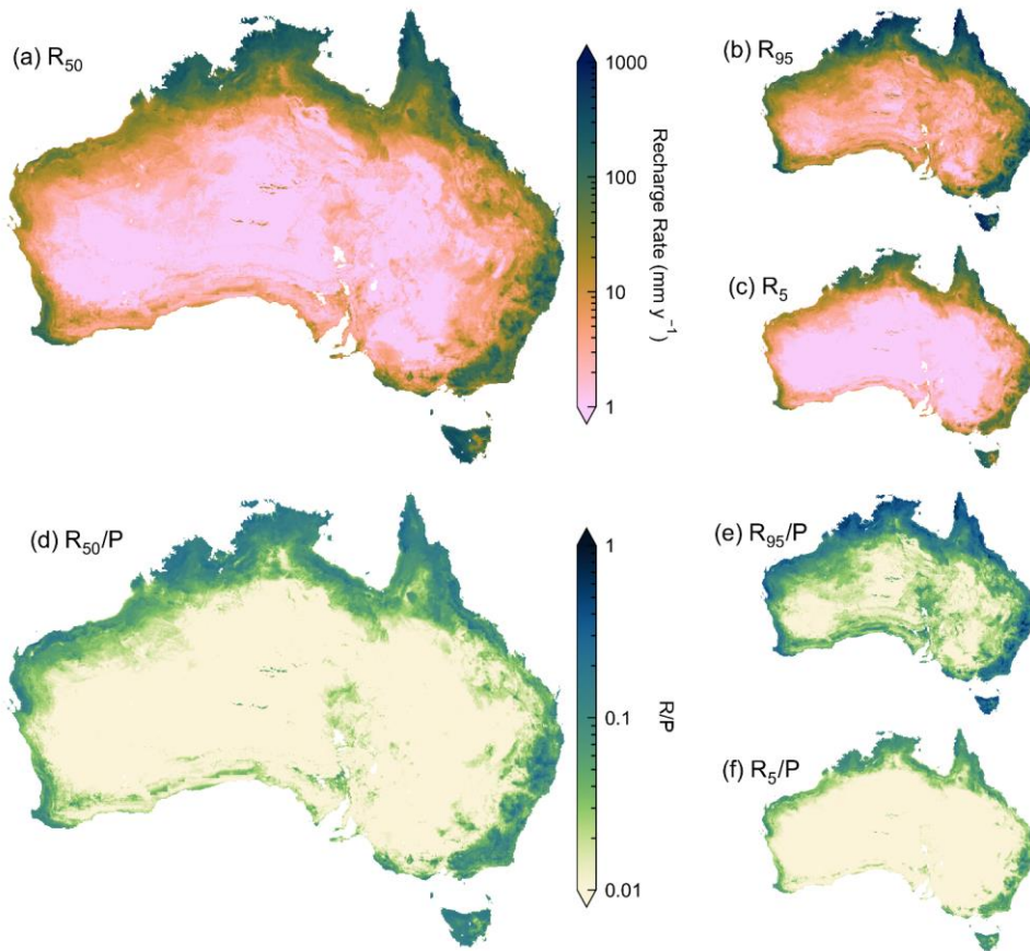
400 Figure 6. Gridded groundwater recharge rate map of Australia generated using the highest performing random forest model, shown as (a) median recharge rate ( R_{50} ), (b) 95 th percentile recharge rate ( R_{95} ) and (c) 5 th percentile recharge rate ( R_5 ) values, and gridded recharge ratio (R/P) map of Australia, shown as (d) R_{50}/P , (e) R_{95}/P and (f) R_5/P . Gridded datasets are available for download, see Code and data availability.
