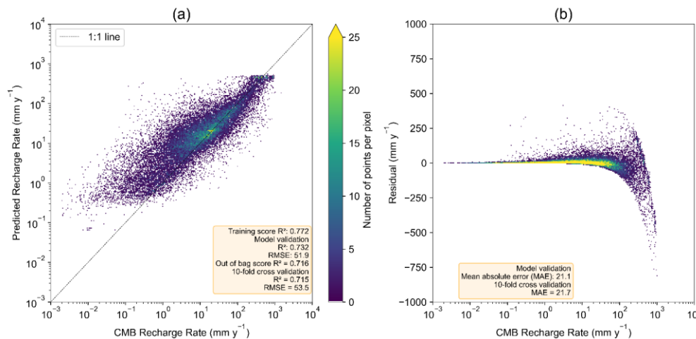
Figure 5. Model validation results for the selected R_{50} model trained using 250 trees, showing: (a) CMB recharge rate ( R_{50} ) versus predicted recharge rate, showing 1:1 line, and point density, and (b) CMB recharge rate ( R_{50} ) versus residuals (predicted recharge rate minus CMB recharge rate) and point density.
