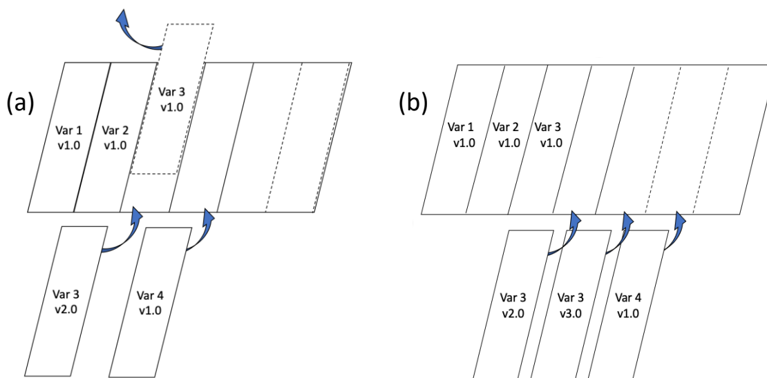
290 Figure 2: There are 2 approaches for MODF augmentation (as new variables become available) and modification (as variables proceed through processing levels). In both approaches, variables that are immediately available (Var 1, Var 2) can be immediately ingested and variables can be added as they become available (Var 3, Var 4). The 2 approaches accommodate two strategies for variables that undergo post processing resulting in products with quality-control (QC) levels. In (a), original data (Var 3 v1.0) can be replaced with QC'ed data (Var3 v2.0). In (b), original data (Var3 v1.0) can be retained in the MODF and QC'ed data (Var3, 2.0) can be added.
