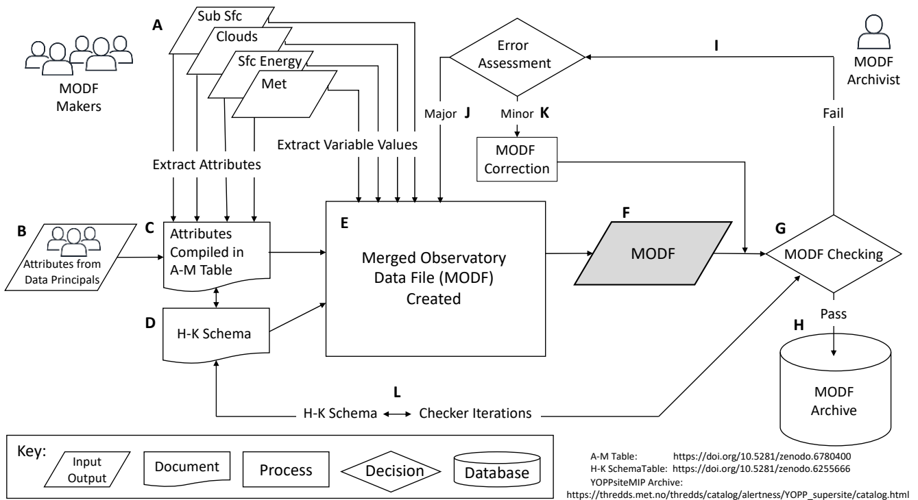
460 Figure 3: The MODF workflow process. A: Gather input files, B: Interview contributing data principals for necessary metadata not digitally encoded in data files, C: Utilize the A-M MODF template to construct the specific MODF framework based inputs from A and B compliant with the H-K Schema (D). MODF Makers create the MODF (E) with inputs from (C) and the data values from individual files collected (A). F: MODF file. G: MODF checking. H: Upon ‘pass’, send MODF to archive. I: Upon ‘fail’ assess MODF. J: Major fails, return MODF Makers. K: Minor fails, archivist corrects and sends MODF to archive after rechecking (G). 465 L: Iterative developments between H-K schema (D) and MODF checking (L). People icons adapted from one designed by vectorstock (Image #45970079 at VectorStock.com).
