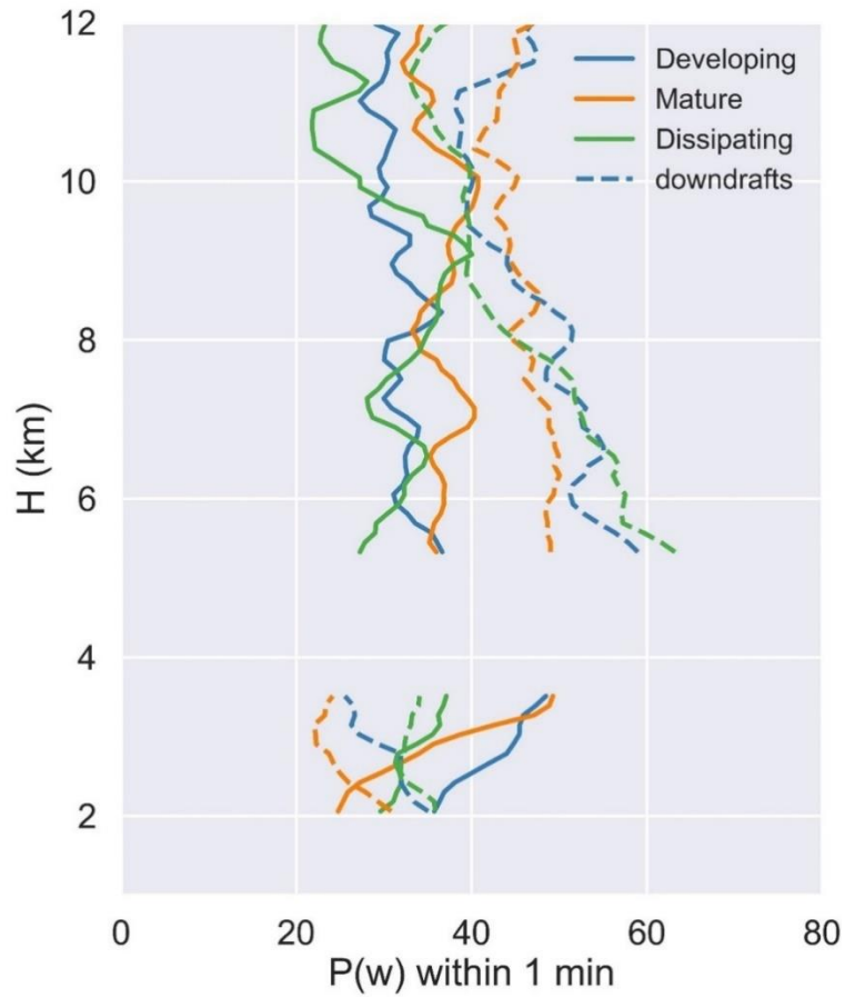
875 Figure 13: Vertical profiles of the average probability of sampling an updraft with w > 1 \text{ m s}^{-1} (solid lines) or a downdraft with w < -1 \text{ m s}^{-1} (dotted dashed lines) within 1 minute of the DCC overpass time.
