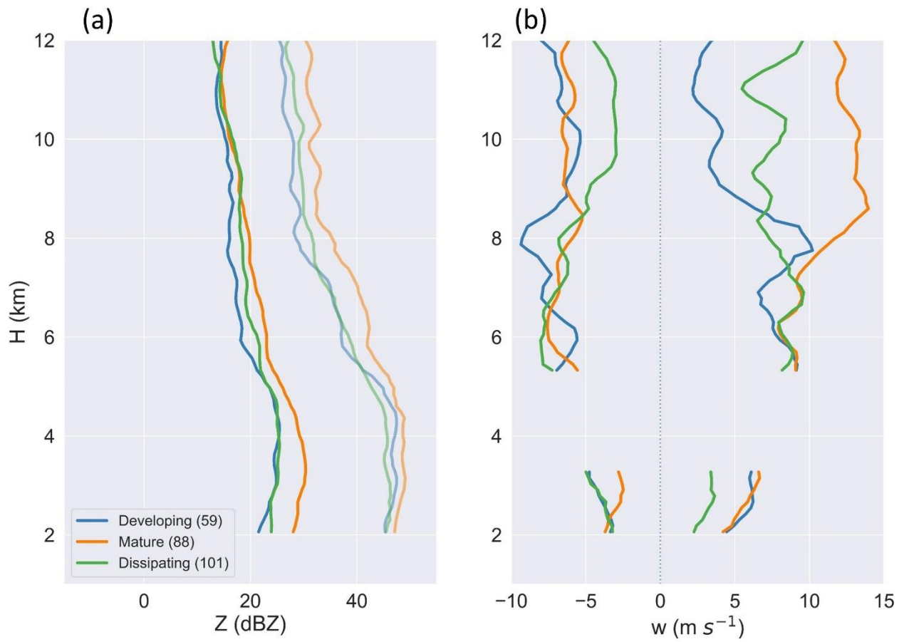
855 Figure 9: Profiles of (a) the average (darker lines) and maximum reflectivity ( Z ) and (b) 95 th percentiles of updrafts with w > 1 \text{ m s}^{-1} and downdrafts with w < -1 \text{ m s}^{-1} for developing, mature, and dissipating DCCs.
