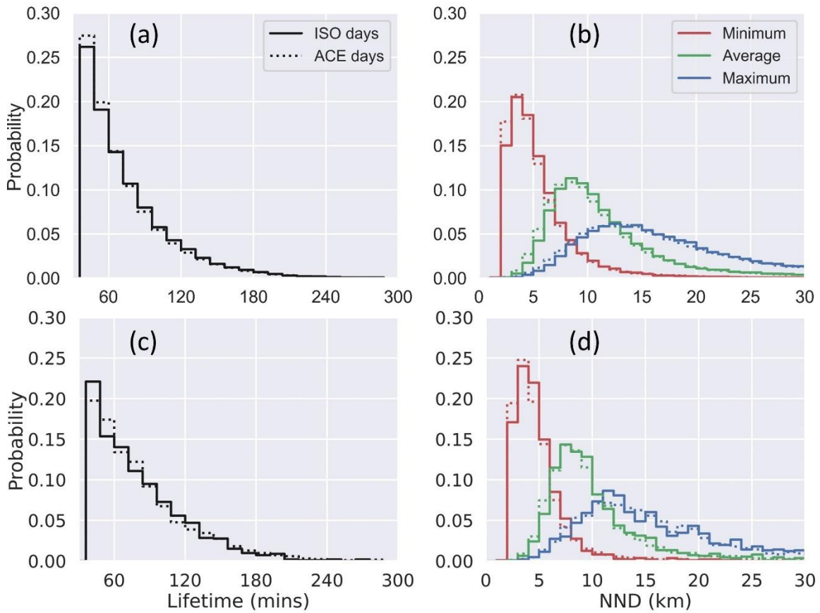
Figure 3: Probability distributions of (a,c) DCC lifetime and (b,d) nearest neighbor distance (NND) for cells with lifetime > 36 mins for (a,b) all cells within radar domain and (c,d) cells within 20 km of MAO with propagation speed > 0.5 m s -1 .
