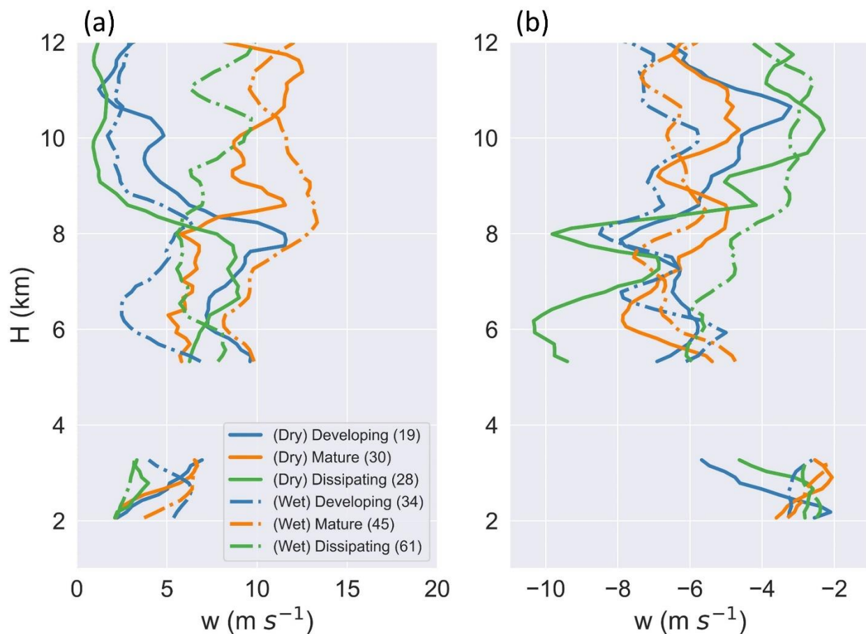
865 Figure 11: Profiles of (a) strongest updrafts (95 th percentile of w > 1 \text{ m s}^{-1} ) and (b) strongest downdrafts (5 th percentile of w < -1 \text{ m s}^{-1} ) for developing, mature, and dissipating DCCs from the dry season (solid lines) and wet season (dotted dashed lines).
