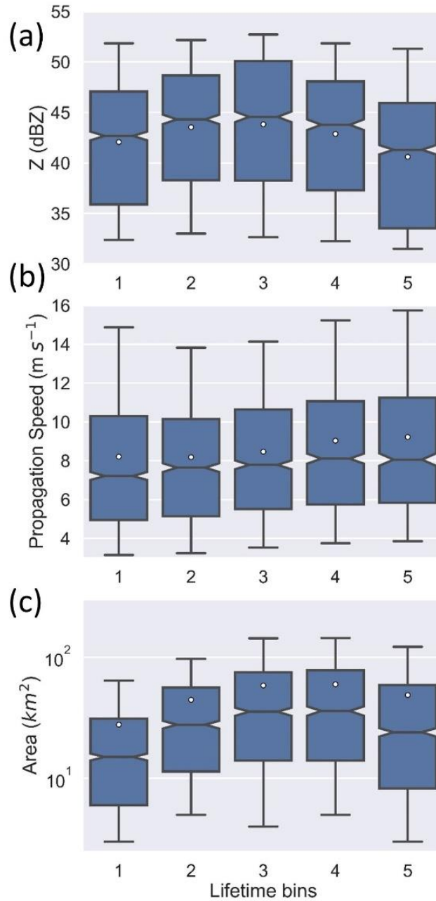
Figure 4: Boxplots of (a) reflectivity ( Z ) at feature position, (b) propagation speed, and (c) area as a function of lifetime bins for cells within 20 km of MAO (lifetime > 30 mins, propagation speed > 0.5 m s -1 , and maximum area < 500 km 2 ) on ISO days. Box lengths represent the interquartile range and whiskers extend to the 5 th and 95 th percentiles. White circles indicate average values and notches extend to the 95 % confidence intervals for the median value.
