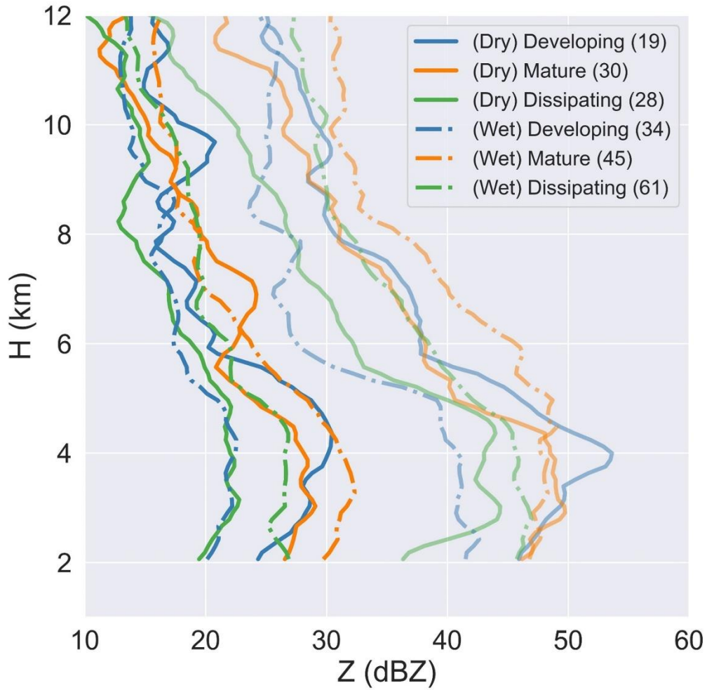
860 Figure 10: Profiles of the average Z (darker lines) and maximum Z (95 th percentile) for developing, mature, and dissipating DCCs from the dry season (solid lines) and wet season (dotted dashed lines).
