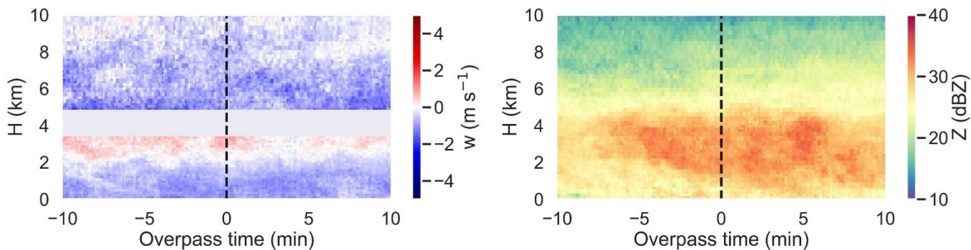
870 Figure 12: Time-height composites of vertical velocity ( w ) and reflectivity ( Z ) from the RWP for DCCs in the “mature” lifecycle stage (for each pixel, the composites represent the median value across all DCCs classified as “mature”).
