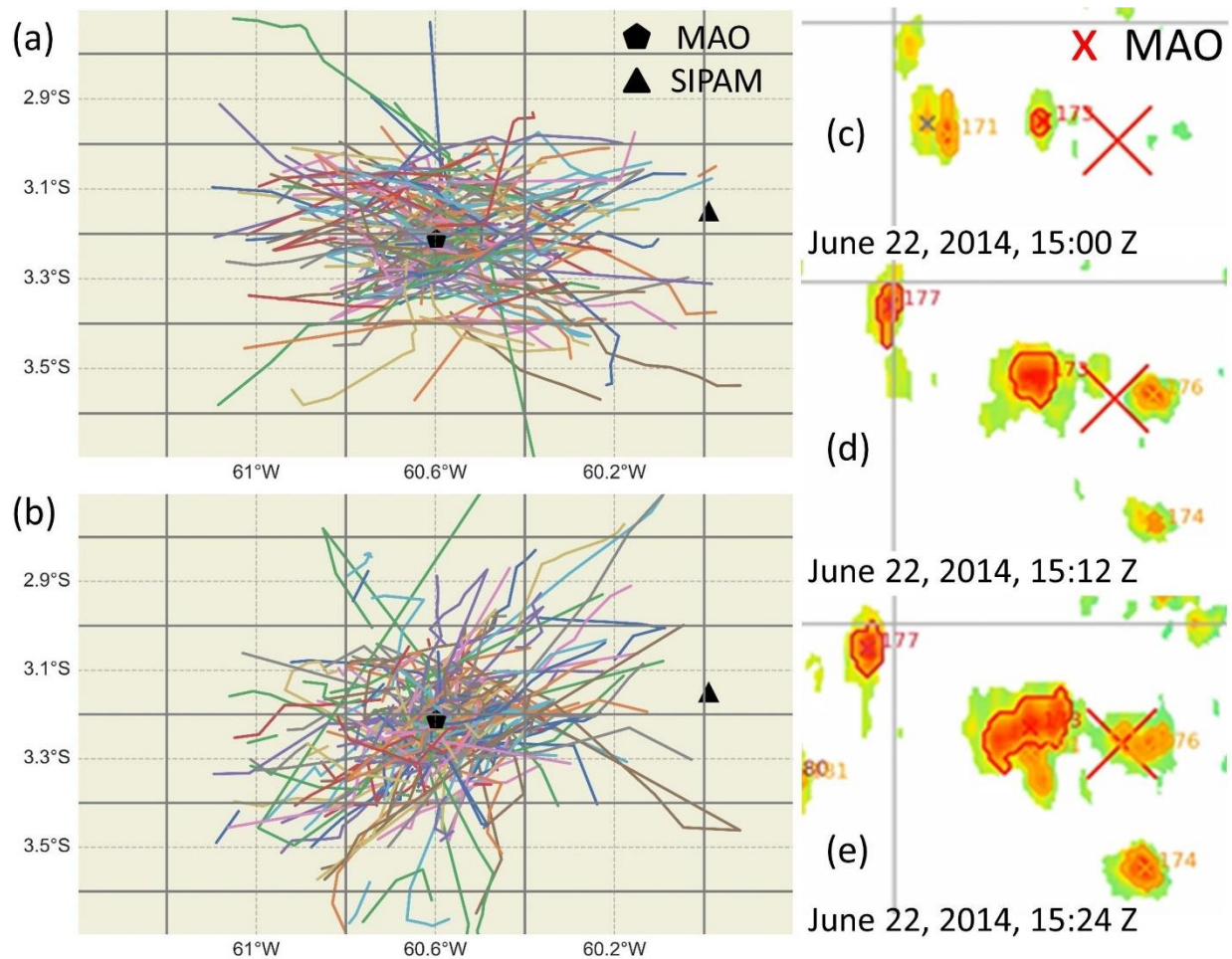
Figure 1: Cell tracks for isolated DCCs tracked during the (a) dry season (June-September) and (b) wet season (December to April). Panels (c), (d), and (e) show the gridded reflectivity field near MAO on June 22, 2014 from 15:00 to 15:24 Z with tobac-identified features surrounded by polygons representing their areal extent.
