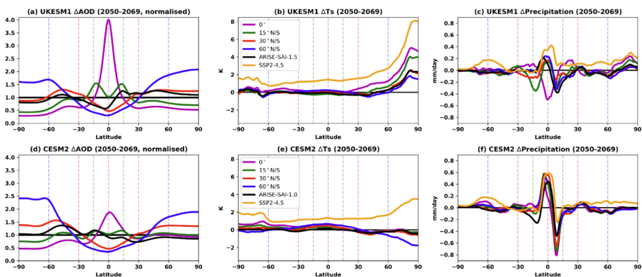
Figure 4. A comparison of aerosol optical depth (at 550 nm), surface air temperature change, and precipitation change for two Earth System Models (UKESM1 and CESM2) using different latitudes: injecting everything at the equator ( 0^\circ ), symmetric injection in both hemispheres ( 15^\circ N/S , 30^\circ N/S , and 60^\circ N/S ), or injection at 15^\circ N , 30^\circ N , 15^\circ S , and 30^\circ S with the objective of maintaining the equator-to-pole and interhemispheric differences in temperature at their reference levels (ARISE-SAI-1.5, Richter et al. 2022, Henry et al. 2023). The target for CESM2 is 0.5^\circ C below its reference period (2020-39), whereas the target for UKESM1 is 1.5^\circ C above its preindustrial temperature, which is reached in 2014-2033. Shown are the temperature and precipitation changes with respect to each model's reference period. UKESM1 has 1 ensemble member per experiment whereas CESM2 has 3 ensemble members per experiment.
