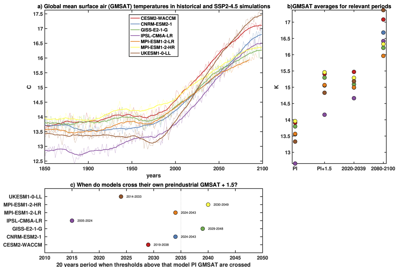
Figure 2. Global mean surface air temperature (GMSAT) in models participating in the sixth phase of GeoMIP for the historical (1850-2014) and SSP2-4.5 (2015-2100) period, showing annual means (thin lines) and 20-years running means (thick lines). b) GMSAT averages for periods relevant to the question of start and end dates for SRM experiments. PI is defined as the average, for each model, over their entire simulated PI control simulations. c) Time periods in which each model’s SSP2-4.5 simulation reaches PI+1.5 (considering a 20-year running average). The year 2035 (the proposed start date for PI+1.5 not considering the model PI) is indicated with a vertical dashed line. For this figure, only the first ensemble member for each model has been used for consistency.
