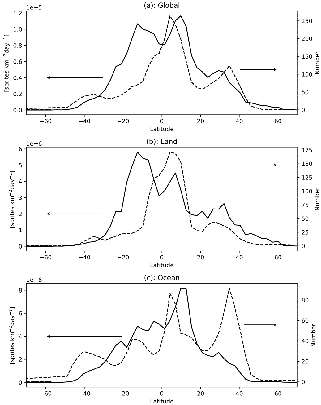
Figure 2. The solid lines depict the simulated annual average latitudinal sprite density, measured in sprites per square kilometer per day, spanning the years 2001 to 2009 (SPRI simulation), encompassing both, land and ocean regions. The dashed lines represent the total number of pure sprites and sprites accompanied by halos observed by ISUAL, as illustrated by (Lu et al., 2022, Figure 2(b)). The observations have been interpolated to the corresponding latitudes of the simulation results.
