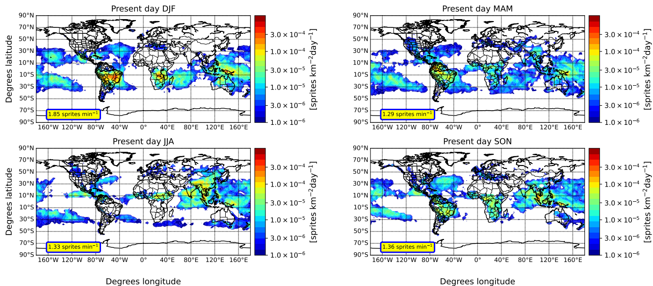
Figure 3. Simulated seasonally averaged sprite density in sprites per squared kilometer and day during 2001-2009 from the SPRI simulation. We annotate in boxes the seasonally averaged occurrence rate of sprites per minute.
