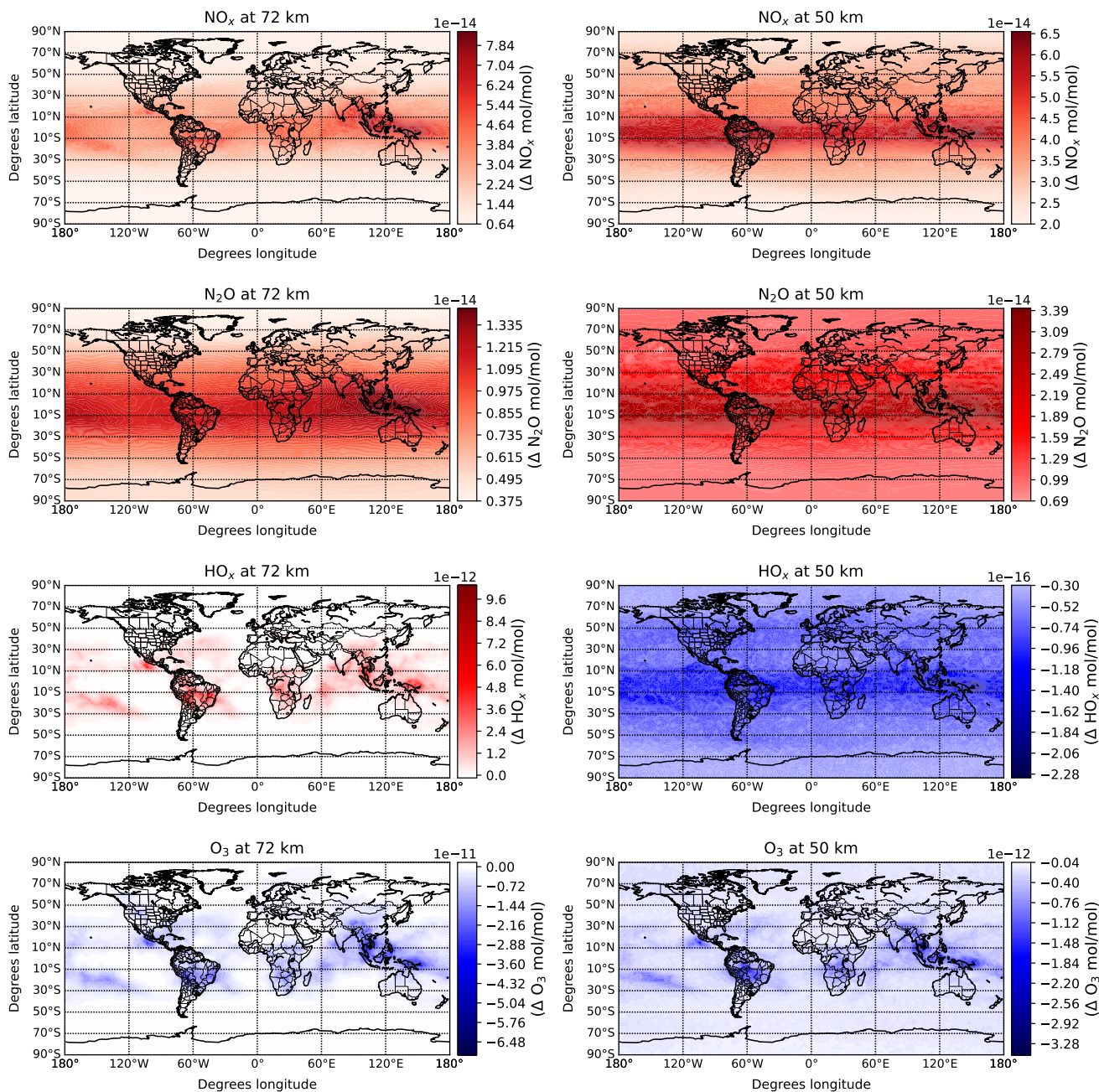
Figure 7. Same as Figure 6 but assuming that a single sprite injects 10^{25} \text{HO}_2 molecules (SPRI-SMI simulation) as reported by Yamada et al. (2020).
