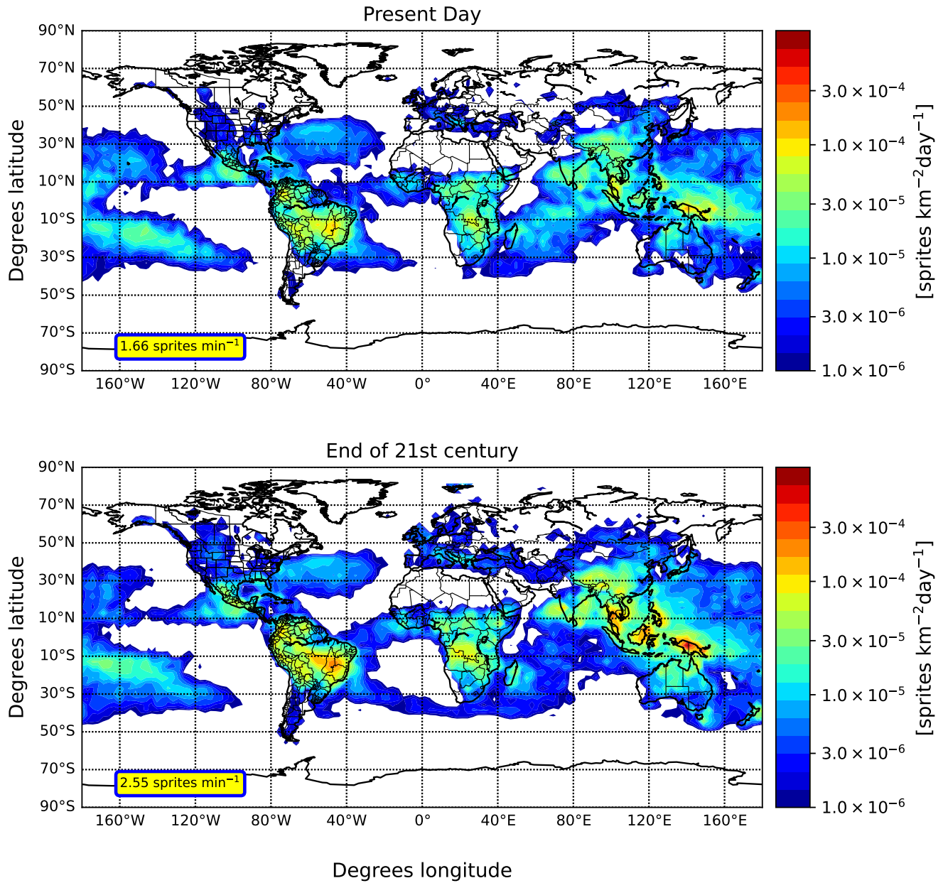
Figure 1. Simulated annually averaged sprite density in sprites per squared kilometer and day during 2001-2009 from the SPRI simulation (a) and during 2091-2095 from the RCP6.0 simulation (b). We annotate in boxes the annually averaged occurrence rate of sprites per minute.
