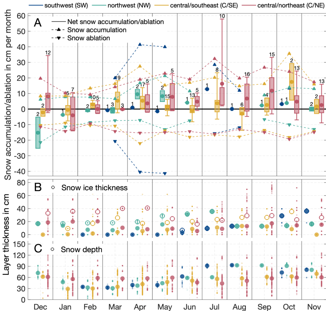
Figure 2. A Monthly mean snow accumulation rates (upward triangles), snow ablation (downward triangle), and net accumulation (positive) or ablation (negative) rates (boxplots) of all Snow Buoys separated for the four regions in the Weddell Sea (see Figure 1). Data were included if at least 25 days per cycle were available in the respective month and region. Numbers indicate the amount of annual buoy cycles contributing to the mean value. In the boxplots, boxes span over the first and third quartiles. The whiskers display the 10 th and 90 th percentiles; the circles indicate mean values, which may include contributions from both accumulation and ablation. Panels B and C display the calculated layer thicknesses of snow ice and snow, respectively, from the applied 1-D thermodynamic sea ice growth model. Small dots represent individual point calculations
