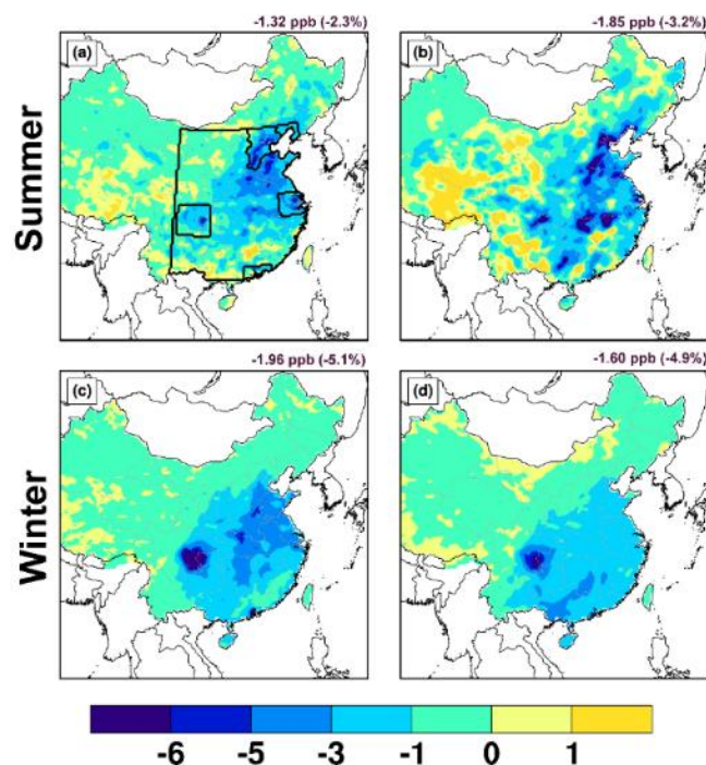
Figure R2. The effects of aerosol-radiation interaction on surface-layer MDA8 O 3 in summer (upper) and winter (bottom) 2017 calculated by (a, c) CBMZ-MOSAIC and (b, d) MOZART-MOSAIC chemical mechanisms. The changes (percentage changes) averaged over China are also shown at the top of each panel.
