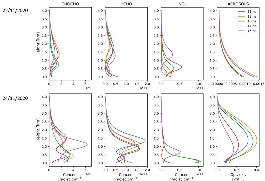
Figure 9. Retrieved gas and aerosol profiles for November 22 (top row) and November 24 (bottom row) at different hours during the day for the eastern direction.
