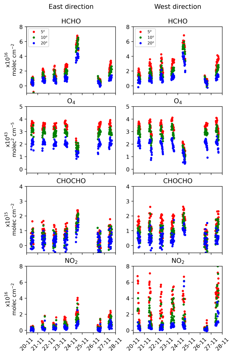
Figure 6. Differential Slant Column Densities for elevation angles 5° (red), 10° (green) and 20° (blue), for the trace gases HCHO, O 4 , CHOCHO and NO 2 (first to fourth row, respectively) for the study period. Results for east and west directions are separated in the left and right panels, respectively. An increase in the dSCD values of HCHO is observed on November 24. The O 4 dSCD values observed for that date are lower and coalesce for the different elevation angles, which indicates a high aerosol load. The glyoxal signal also increases on November 24, although not as clearly as that of formaldehyde. The observed changes in NO 2 dSCD values for that day with respect to background are relatively small and may not be attributed to the event.
