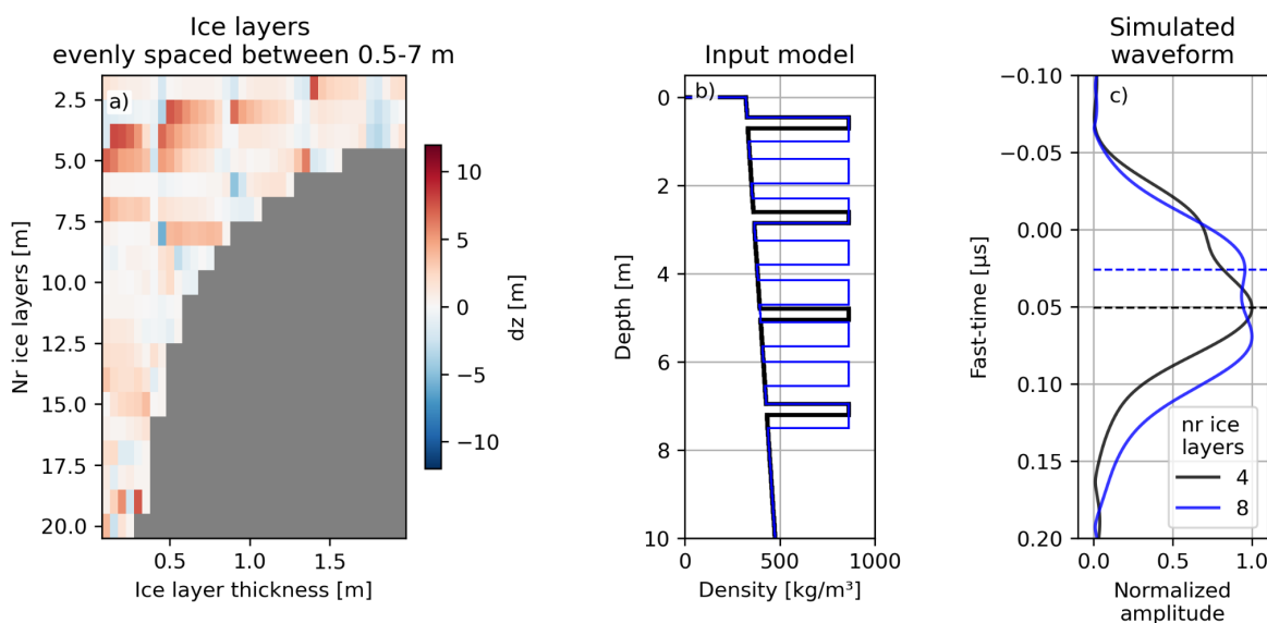
270 Figure 5: a) Surface peak offset ( dz ) for RadSPy simulated MCoRDS surface returns over firn stratigraphies with multiple ice layers of varying thickness. b) Two example input models, and c) the resulting simulated waveforms.
