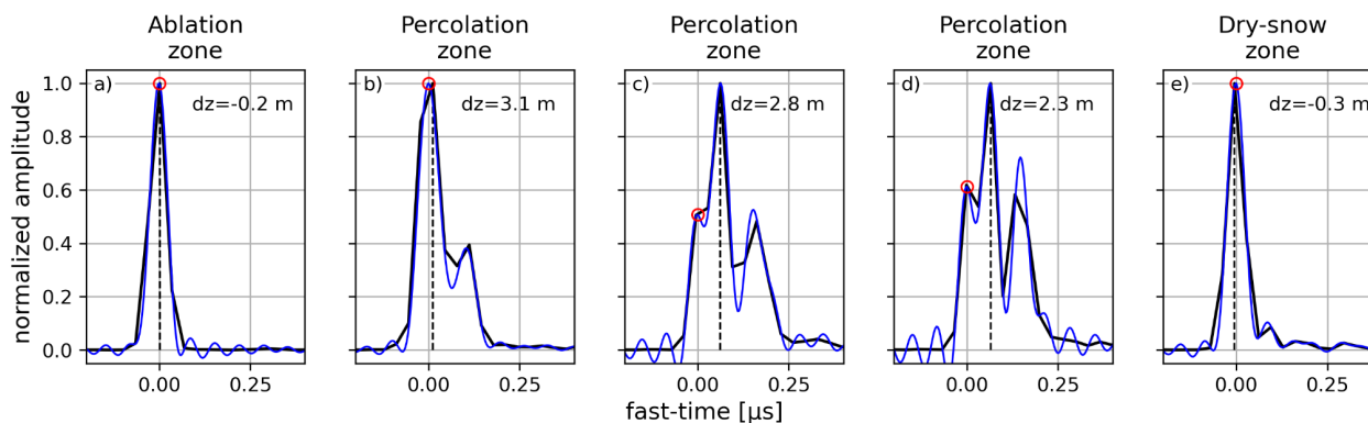
120 Figure 2: Example MCoRDS radar traces along Profile A (Figure 7) collected in 2017 (see Figure 1 for trace location) showing typical surface returns over the ablation zone (a), percolation zone (b-d, note the three traces are neighbouring traces and represented with one location marker on Figure 1), and dry snow zone (e). Black is the measured MCoRDS signal and blue is the up-sampled signal. The black dashed line shows the peak provided by CReSIS whereas the red dot is the re-picked reflection used as ice sheet surface representative and to calculate the radar peak offsets. The trace energy is normalised, and fast-times (traveltime) are presented relative to the re-picked surface.
