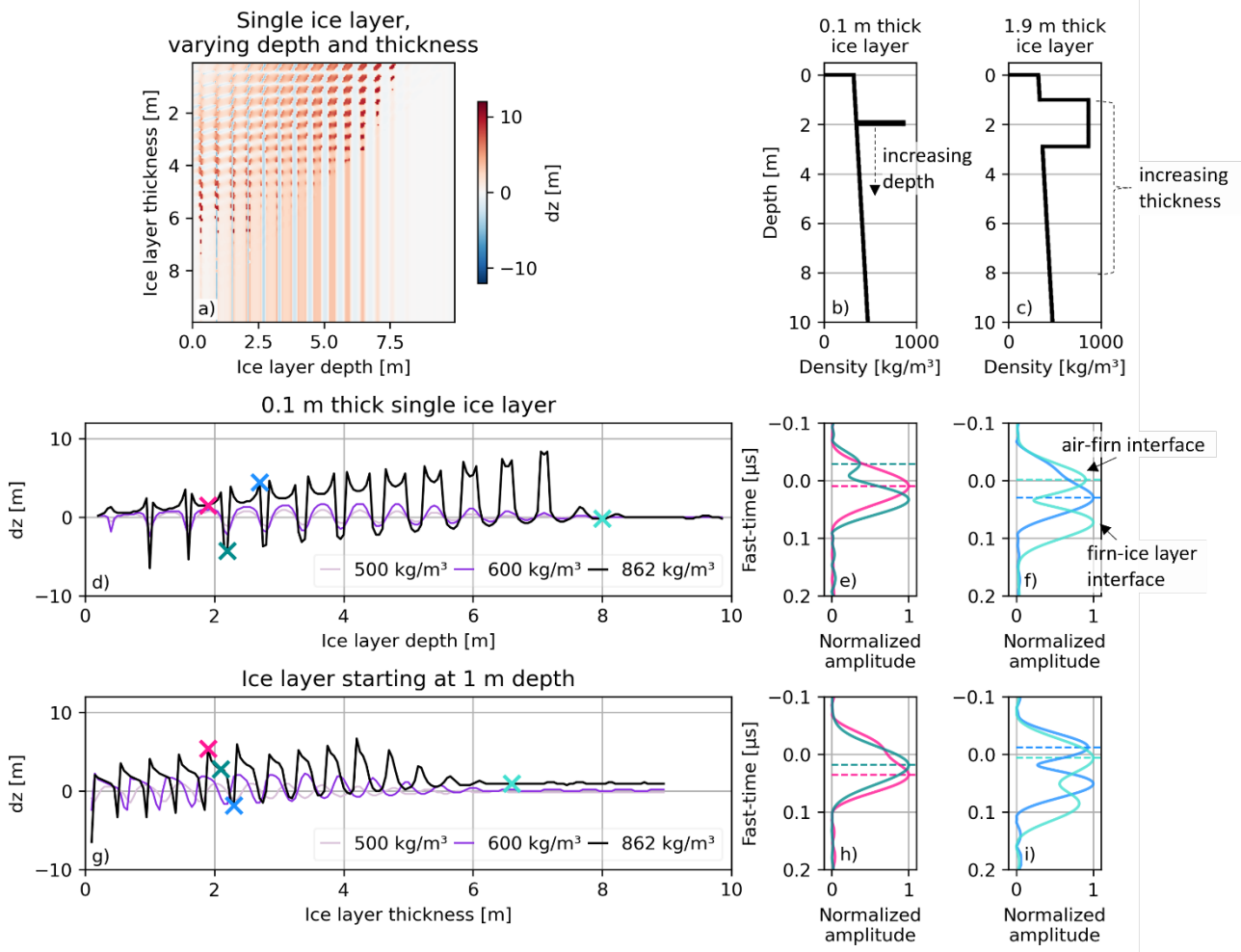
250 Figure 4: a) Surface peak offset ( dz ) for RadSPy simulated MCoRDS surface returns over firn stratigraphies consisting of a single ice layer placed at various depths and with different thicknesses. b) and c) show example model input profiles. d) dz for a 0.1 m 255 thick ice layer, as well as layers with densities of 500 \text{ kg/m}^3 and 600 \text{ kg/m}^3 at different depths, with waveforms for selected ice layer depths (marked with crosses) shown in e and f. g) dz for an ice layer, as well as layers with densities of 500 \text{ kg/m}^3 and 600 \text{ kg/m}^3 , starting at 1 m depth and with increasing layer thickness, with waveforms for selected ice layer thicknesses (marked with crosses) show in h and i. The dotted lines in the waveform plots show the picked peak identified used to calculate dz .
