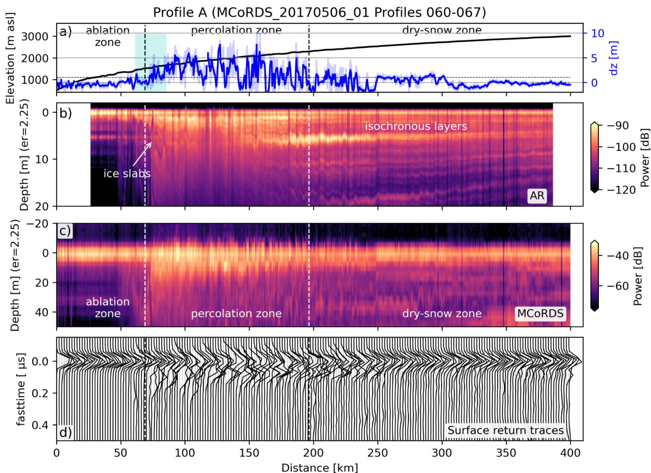
330 Figure 8: Radar surface peak offset ( dz ) over OIB CREStS MCoRDS and Accumulation Radar (AR) profile A in Central West Greenland (see Figure 7e for profile location). a) Ice sheet surface elevation (black) and dz (raw in light blue, and smoothed over a 1 km window in dark blue) along the profile. Vertical dotted black/white lines indicate the firn zone transitions (ablation zone, percolation zone, dry-snow zone) derived from MAR, and the blue shaded area marks the location of previously mapped ice slabs (Jullien et al., 2023). b) AR data showing the firn stratigraphy, including ice slabs and isochronous layers of the uppermost 20 m. 335 c) MCoRDS data of the uppermost 50 m in firn/ice. The radargrams have been flattened with respect to the picked surface reflection. d) MCoRDS traces along the profile showing the shape of the surface reflection along the profile. The traces are aligned with respect to the picked surface reflection, and normalised to the maximum energy.
