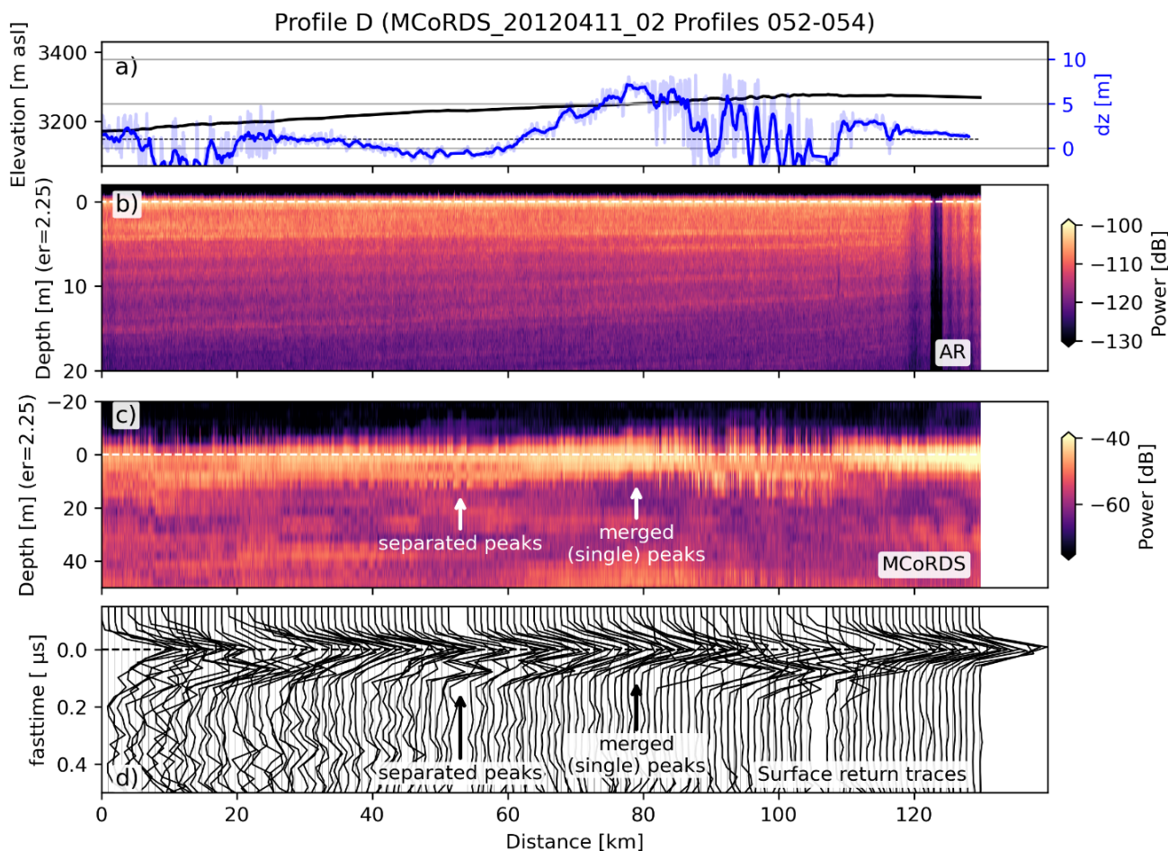
345 Figure 9: Radar surface peak offset ( dz ) over OIB CReSIS MCoRDS and Accumulation Radar (AR) profile D over the dz anomaly region near the summit (see Figure 7b for profile location). a) Ice sheet surface elevation (black) and dz (blue) along the profile. b) AR data showing the firn stratigraphy of the uppermost 20 m. c) MCoRDS data of the uppermost 50 m in firn/ice. The radargrams have been flattened with respect to the picked surface reflection. d) MCoRDS traces along the profile showing the shape of the surface reflection along the profile. The traces are aligned with respect to the picked surface reflection, and normalised to the maximum energy.
