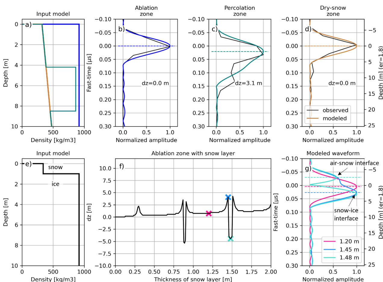
225 Figure 3: RadSPy model input depth-density profiles, representing the ablation- (blue), percolation- (teal), and dry-snow zones (brown). b-c) RadSPy modelled signals for the different input stratigraphies. The coloured curves represent the modelled signal, while the black curves represent typical MCoRDS traces observed over the different firn facies (Figure 2). e) RadSPy model input depth-density profile representing a snow layer on top of the ablation zone. f) Modelled surface peak offset over the ablation zone as function of the snow layer thickness. g) examples of modelled waveforms for selected snow layer thicknesses (marked with crosses on f).
