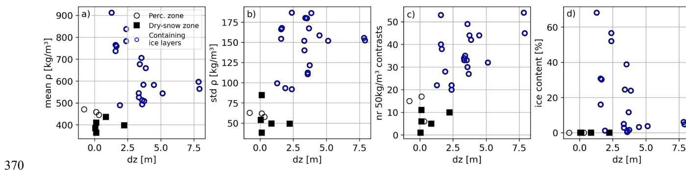
Figure 10: Radar surface peak offset ( dz ) versus firn core properties (extending from surface to 7.5 m depth): a) mean density, b) the standard deviation of the firn density, c) the number of density contrasts above 50 kg/m 3 , and d) the firn ice content (calculated as length percentage of firn density exceeding 862 kg/m 3 ). Blue markers indicate firn cores that contain ice layers.
