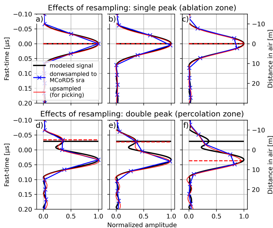
290 Figure 6: Effects of downsampled signals to the MCoRDS sampling rate (sra) with different starting lags (0 ns left panels, 5 ns middle panels, 15 ns right panels). a-c) show the RadSPy modelled waveform over the ablation zone (air-ice), and d-f) show the modelled signal over the percolation zone including a 10 cm thick ice layer at 2.1 m depth. Horizontal lines show which peak was identified from the modelled signal at original sampling rate (black) and downsampled signals (red dashed).
