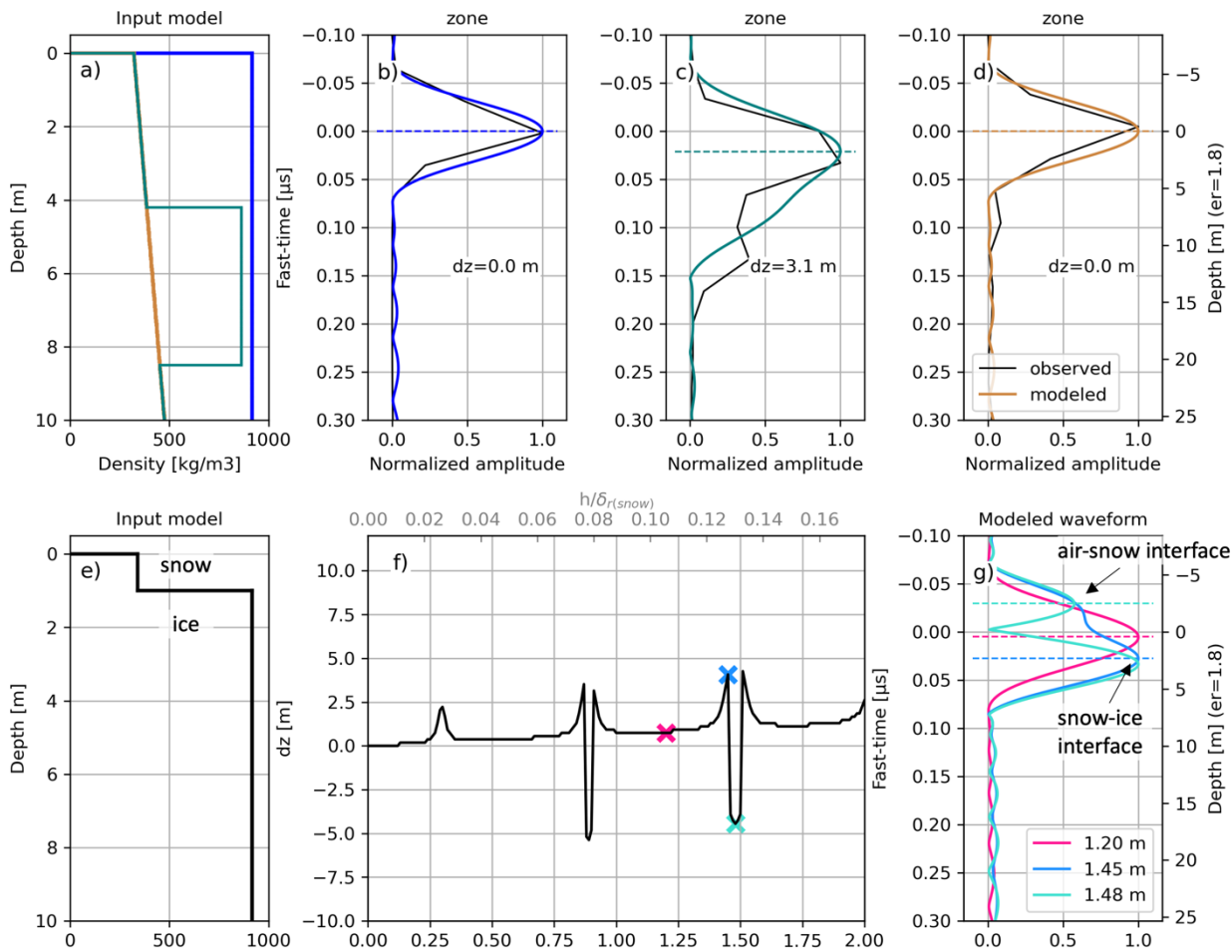
Figure 3: RadSPy model input depth-density profiles, representing the ablation- (blue), percolation- (teal), and dry-snow zones (brown). b-c) RadSPy modelled signals for the different input stratigraphies. The coloured curves represent the modelled signal, while the black curves represent typical MCoRDS traces observed over the different firn facies (Figure 2). e) RadSPy model input depth-density profile representing a snow layer on top of the ablation zone. f) Modelled surface peak offset over the ablation zone as function of the snow layer thickness. The x-axis on the top shows the snow layer thickness scaled by the rang resolution \delta_r of the modelled signal in snow ( \sim 11 m) g) examples of modelled waveforms for selected snow layer thicknesses (marked with crosses on f).
