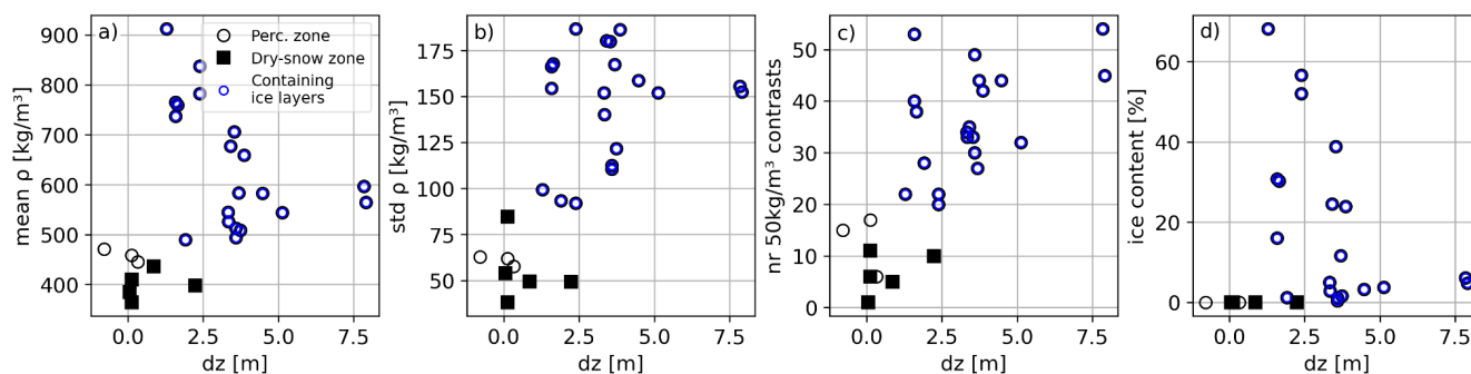
Figure 10: Radar surface peak offset ( dz ) versus firn core properties (extending from surface to 7.5 m depth): a) mean density, b) the standard deviation of the firn density, c) the number of density contrasts above 50 kg/m 3 , and d) the firn ice content (calculated as length percentage of firn density exceeding 862 kg/m 3 ). Blue markers indicate firn cores that contain ice layers.
