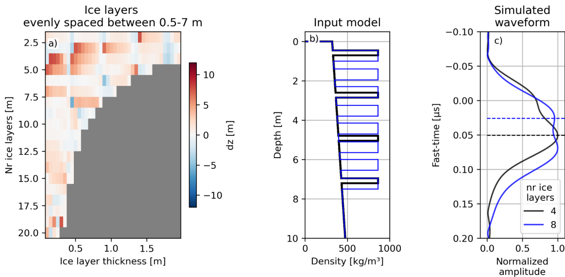
285 Figure 5: a) Surface peak offset ( dz ) for RadSPy simulated MCoRDS surface returns over firm stratigraphies with multiple ice layers of varying thickness. b) Two example input models, and c) the resulting simulated waveforms.
