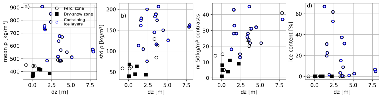
Figure 10: Radar surface peak offset ( dz ) versus firm core properties (extending from surface to 7.55.7 m depth): a) mean density, b) the standard deviation of the firm density, c) the number of density contrasts above 50 kg/m 3 , and d) the firm ice content (calculated as length percentage of firm density exceeding 862 kg/m 3 ). Blue markers indicate firm cores that contain ice layers.
