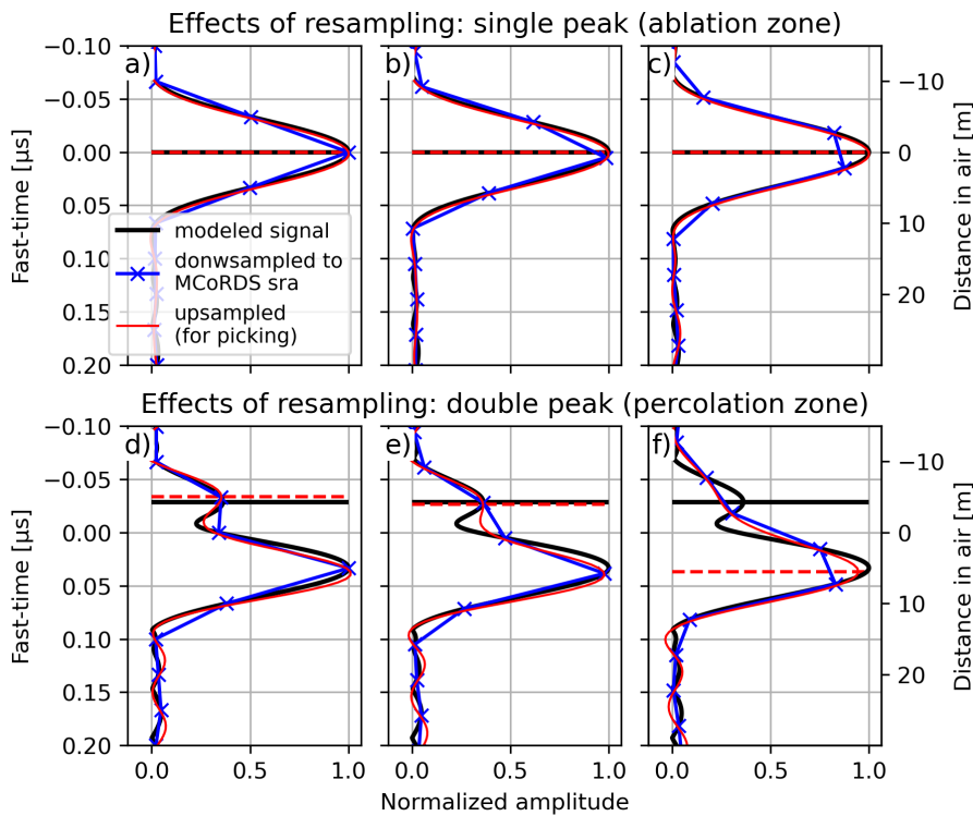
310 Figure 6: Effects of downsampled signals to the MCoRDS sampling rate (sra) with different varying starting lagtime-zero offsets (0 ns left panels, 5 ns middle panels, 15 ns right panels). a-c) show the RadSPy modelled waveform over the ablation zone (air-ice), and d-f) show the modelled signal over the percolation zone including a 10 cm thick ice layer at 2.1 m depth. Horizontal lines show which peak was identified from the modelled signal at original sampling rate (black) and downsampled signals (red dashed).
