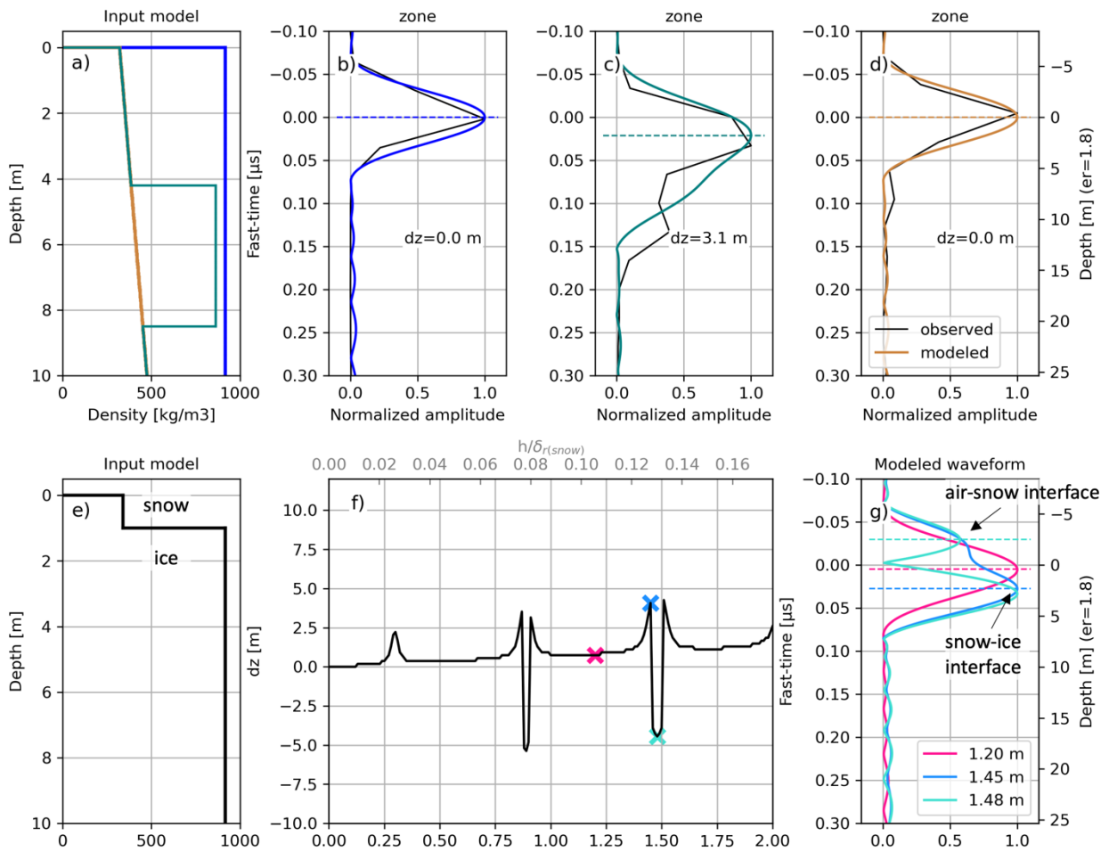
Figure 3: RadSPy model input depth-density profiles, representing the ablation- (blue), percolation- (teal) and dry-snow zones (brown). b-c) RadSPy modelled signals for the different input stratigraphies. The coloured curves represent the modelled signal, while the black curves represent typical MCoRDS traces observed over the different firn facies (Figure 2Figure 2). e) RadSPy model input depth-density profile representing a snow layer on top of the ablation zone. f) Modelled surface peak offset over the ablation zone as function of the snow layer thickness. The x-axis on the top shows the snow layer thickness scaled by the rang resolution \delta_r of the modelled signal in snow (~11 m) g) examples of modelled waveforms for selected snow layer thicknesses (marked with crosses on f).
