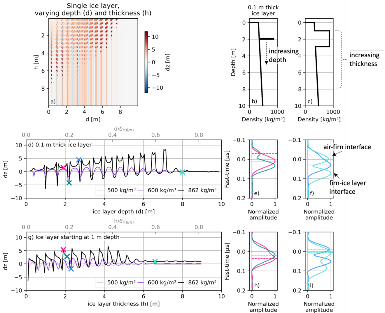
Figure 4: a) Surface peak offset ( dz ) for RadSPy simulated MCoRDS surface returns over firn stratigraphies consisting of a single ice layer placed at various depths and with different thicknesses. b) and c) show example model input profiles. d) dz for a 0.1 m thick ice layer, as well as layers with densities of 500 \text{ kg/m}^3 and 600 \text{ kg/m}^3 at different depths, with waveforms for selected ice layer depths (marked with crosses) shown in e and f. g) dz for an ice layer, as well as layers with densities of 500 \text{ kg/m}^3 and 600 \text{ kg/m}^3 , starting at 1 m depth and with increasing layer thickness, with waveforms for selected ice layer thicknesses (marked with crosses) show in h and i. The dotted lines in the waveform plots show the picked peak identified used to calculate dz . The x-axis on the top of panels d) and g) show the ice layer depth and thickness scaled by the rang resolution \delta_r of the modelled signal in firn ( \sim 11 \text{ m} ).
