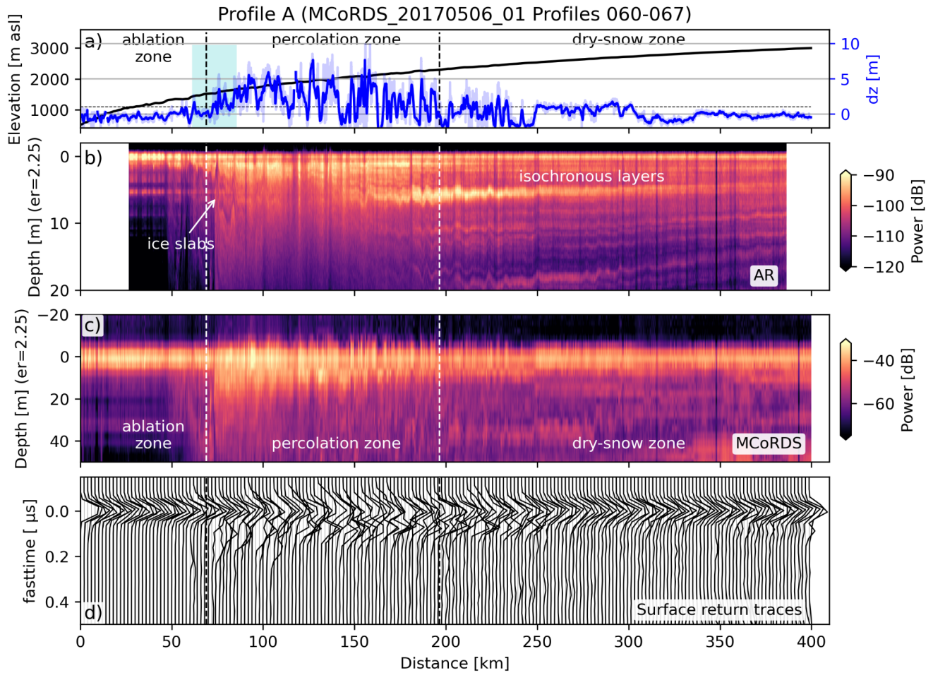
350 Figure 8: Radar surface peak offset ( dz ) over OIB CREsIS MCoRDS and Accumulation Radar (AR) profile A in Central West Greenland (see Figure 7Figure 7e for profile location). a) Ice sheet surface elevation (black) and dz (raw in light blue, and smoothed over a 1 km window in dark blue) along the profile. Vertical dotted black/white lines indicate the firn zone transitions (ablation zone, percolation zone, dry-snow zone) derived from MAR, and the blue shaded area marks the location of previously mapped ice slabs (Jullien et al., 2023). b) AR data showing the firn stratigraphy, including ice slabs and isochronous layers of the uppermost 20 m. c) MCoRDS data of the uppermost 50 m in firn/ice. The radargrams have been flattened with respect to the picked surface reflection. d) MCoRDS traces along the profile showing the shape of the surface reflection along the profile. The traces are aligned with respect to the picked surface reflection, and normalised to the maximum energy.
