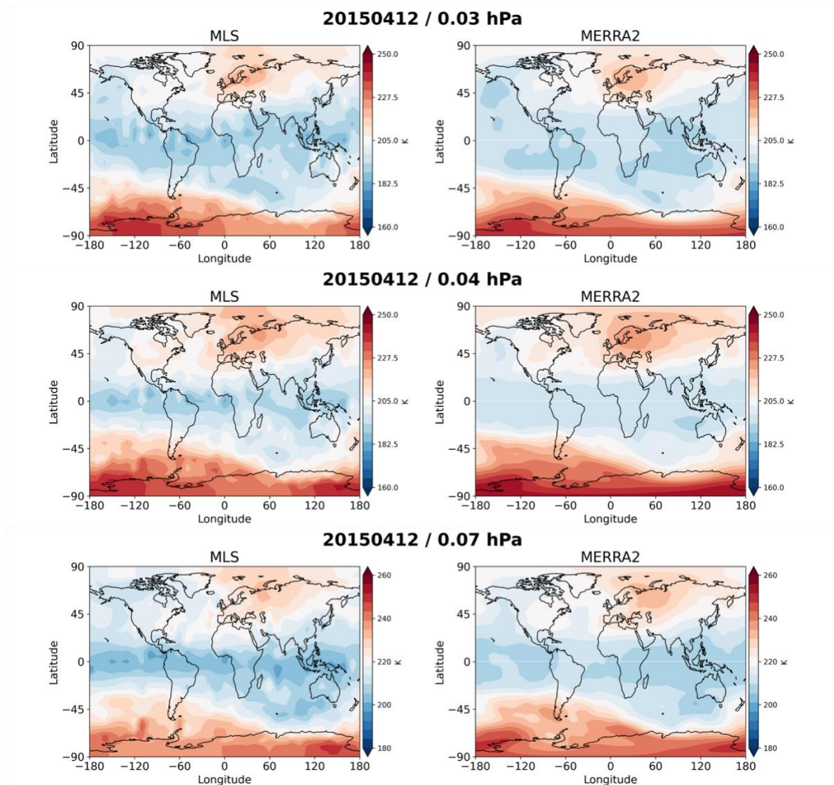
Figure R1 Longitude-Latitude distributions of temperature at three different pressure levels of 0.03 hPa, 0.04 hPa, and 0.07 hPa. For each pressure level, the temperature distributions from (left) MLS and (right) MERRA-2 are presented.
