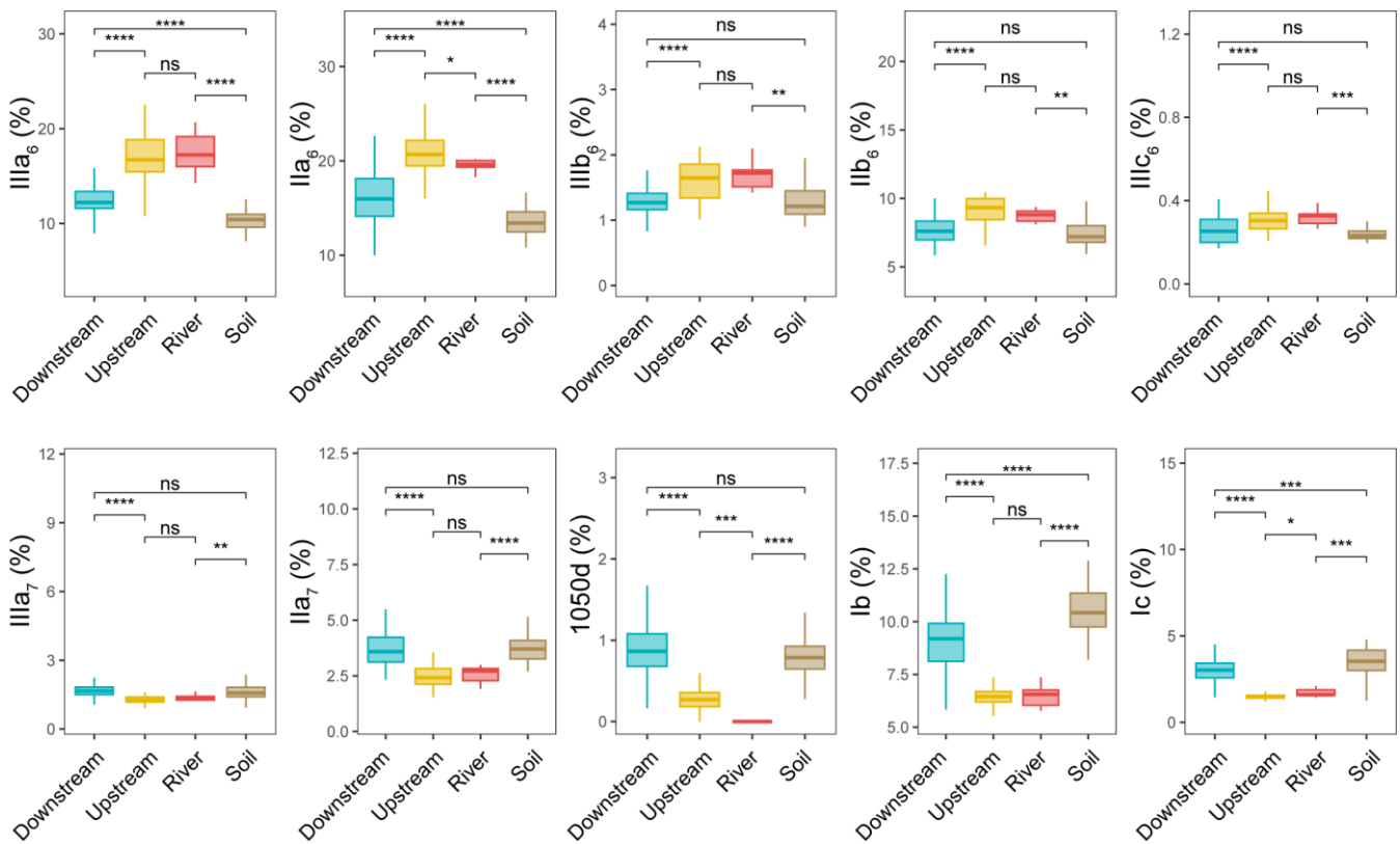
345 Figure 3: Relative abundances of selected individual brGDGTs over 20 brGDGTs (IIIa5, IIIb5, IIIc5, IIa5, IIb5, IIc5, IIIa6, IIIb6, IIIc6, IIa6, IIb6, IIc6, IIIa7, IIIb7, IIa7, Ia, Ib, Ic, 1050d, and 1036d) from soils (surficial soils and mudflat soils/sediments, n=51 ), river ( n=9 ), upstream estuary ( n=56 ), and downstream estuary ( n=121 ) samples across the Seine River basin: cyclopentane-containing tetramethylated brGDGTs (Ib and Ic), 6-methyl brGDGTs (IIa6, IIIa6, IIb6, IIIb6, and IIIc6), 7-methyl brGDGTs (IIa7 and IIIa7) and brGDGT 1050d. Box plots of upstream and downstream estuary samples are based on SPM and sediments, whereas those of river samples are based only on SPM. Boxes show the upper and lower quartiles of the data, and whiskers show the range of the data, which are color-coded based on the sample type (river in red, upstream estuary in yellow, and downstream estuary in blue). The center-line in the boxes indicates the median value of the dataset. Statistical testing was performed by a Wilcoxon test (* P < 0.05 ; ** P < 0.01 ; *** P < 0.001 ; **** P < 0.0001 ; ns, not significant, P > 0.05 ).
