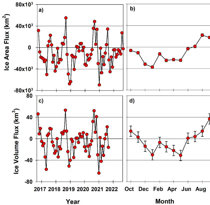
Figure 4: (a) time series of the monthly ice area flux from October 2016 to September 2022, (b) the average monthly ice area flux, 225 (c) time series of the ice volume flux from October 2016 to September 2021, and (d) the average monthly ice volume flux. Positive flux values indicate ice import to the Arctic Ocean or Baffin Bay and negative values indicate ice export from the Arctic Ocean or Baffin Bay. Black vertical bars (b, d) indicate uncertainty.
