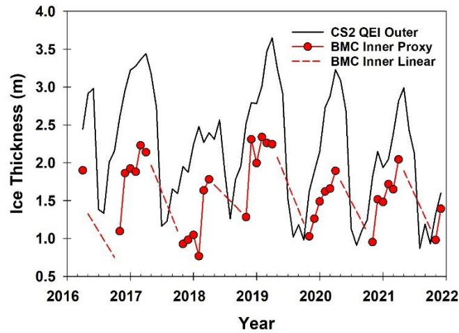
190 Figure 3. Time series of CryoSat-2 ice thickness for the Queen Elizabeth Islands (QEI; black) outer gates, proxy ice thickness for the Byam Martin Channel (BMC, red) inner gate, and linearly interpolated ice thickness for BMC inner gate (dashed red) from 2016-2022.
