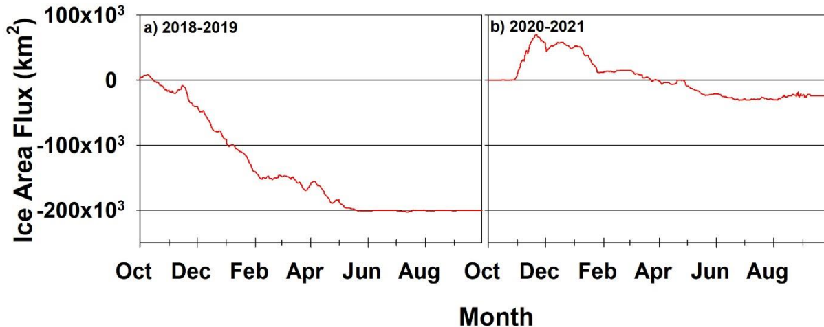
Figure 7: Time series of the Amundsen Gulf cumulative ice area flux for (a) 2018-2019 and (b) 2020-2021. Positive flux values 295 indicate ice import from Arctic Ocean and negative values indicate ice export to the Arctic Ocean.
