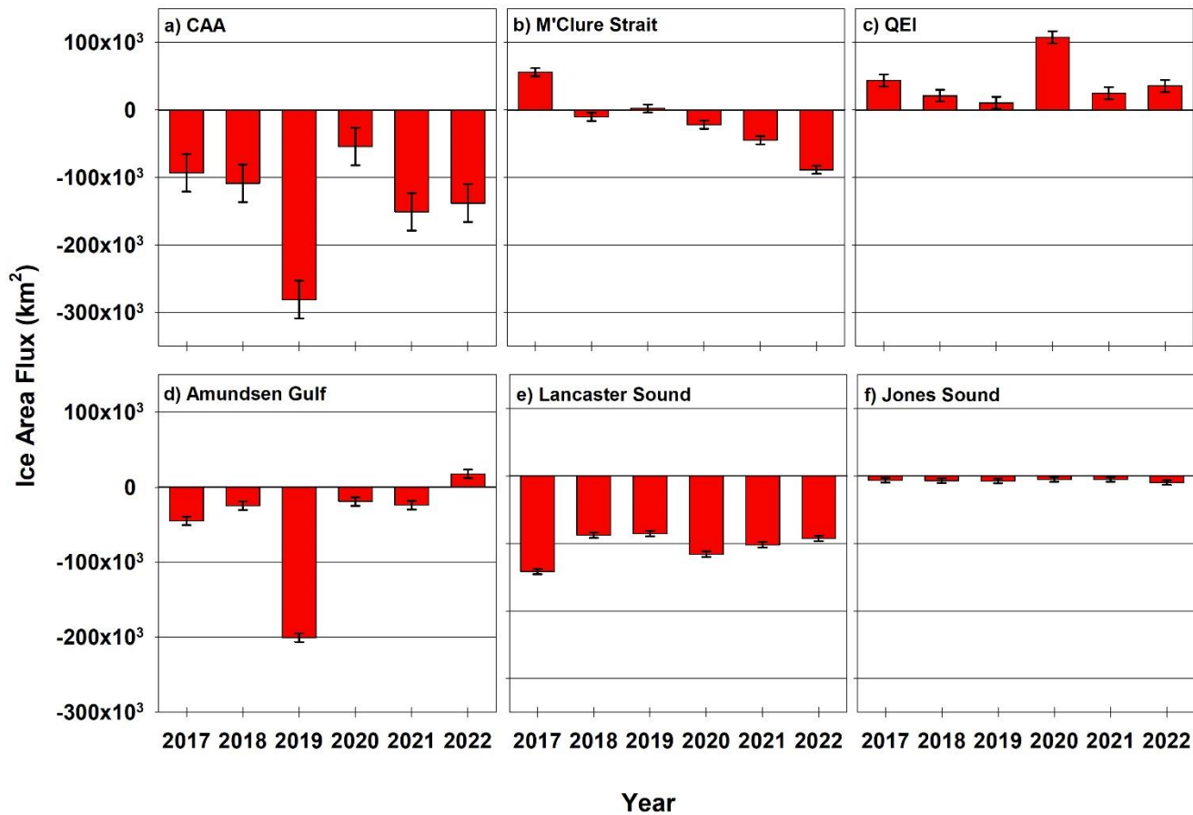
235 Figure 5. Annual (October to September) ice area ice flux (a) the Canadian Arctic Archipelago (CAA), (b) M'Clure Strait, (c) Queen Elizabeth Islands (QEI), (d) Amundsen Gulf, (e) Lancaster Sound, and (f) Jones Sound for 2017 to 2022. Positive flux values indicate ice import from the Arctic Ocean or Baffin Bay and negative values indicate ice export to the Arctic Ocean or Baffin Bay. Black vertical bars indicate uncertainty.
