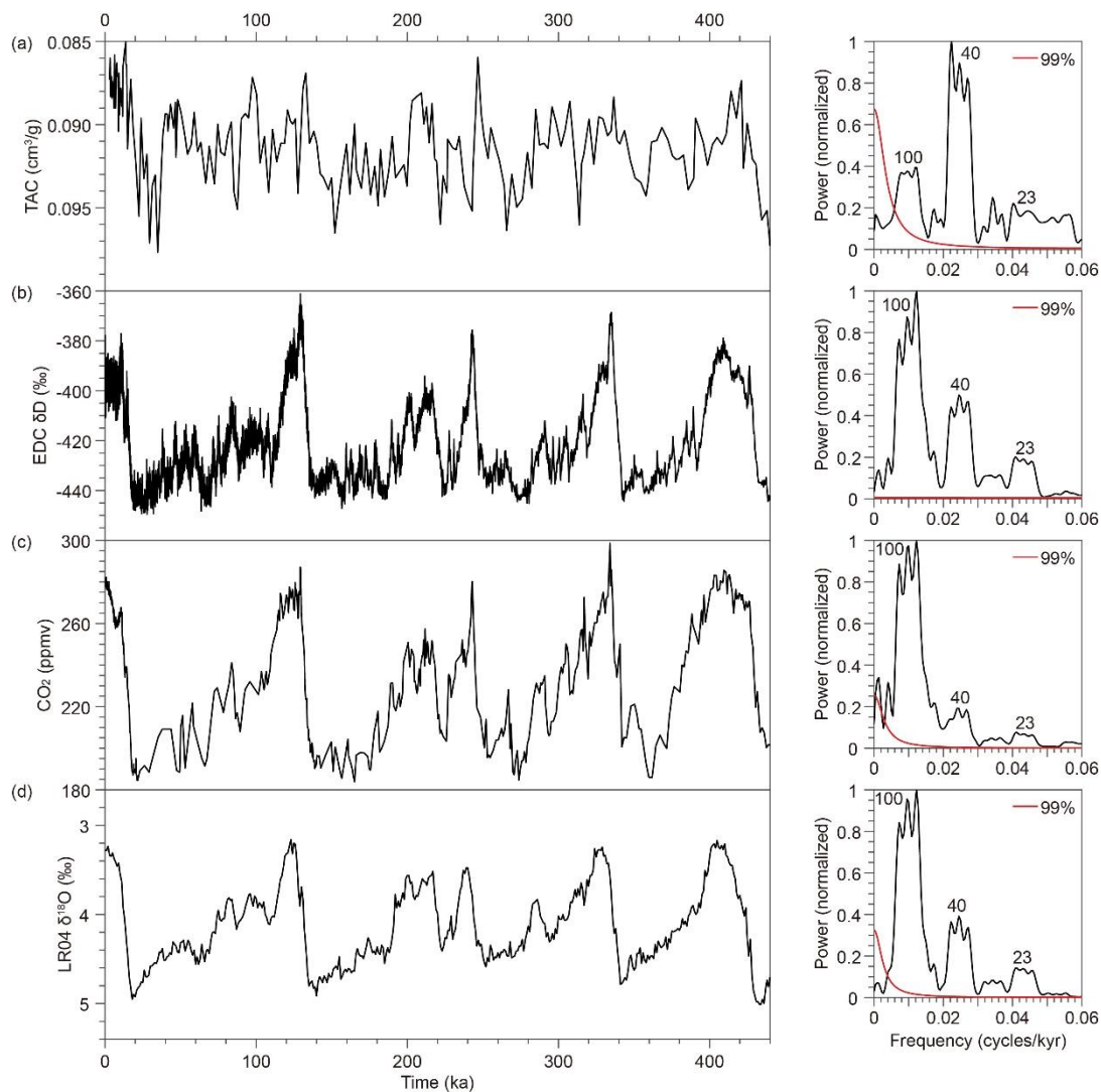
Figure 1. Variations and spectra over the past 440 ka of (a) TAC record (raw data, Raynaud et al. 2007), (b) EDC \delta D record Jouzel et al., 2007, (c) CO 2 concentration Lüthi et al., 2008 and (d) benthic \delta^{18}O Lisiecki and Raymo, 2005. The major periodicities in kyr are indicated. The EDC TAC record, \delta D record and CO 2 concentrations are displayed on the AICC2023 chronology Bouchet et al., 2023. The spectra are calculated using the multi-taper method (MTM), the number of tapers is set to 2 and the zero padding is set to 5, and the 99% confidence limit is shown (red curves).
