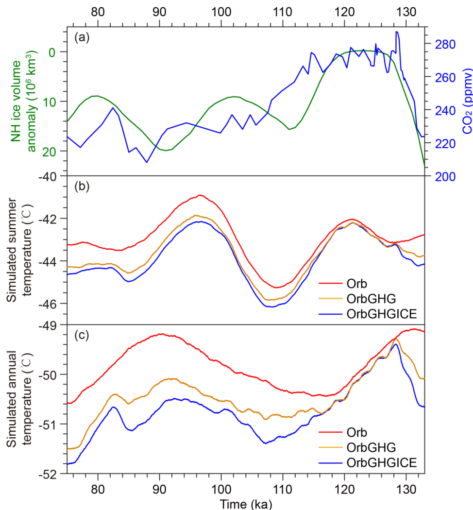
255 Figure 6. LOVECLIM1.3 transient simulation without acceleration for the period 133-75 ka. The effect of insolation, GHG and NH ice sheets on the summer and annual temperature at Dome C. (a) CO 2 concentration (blue, Lüthi et al., 2008) and NH ice volume anomaly as compared to pre-industrial (green, Ganopolski and Calov, 2011), (b) simulated mean half-year summer temperature and (c) simulated annual mean temperature from the Orb, OrbGHG and OrbGHGICE experiments.
