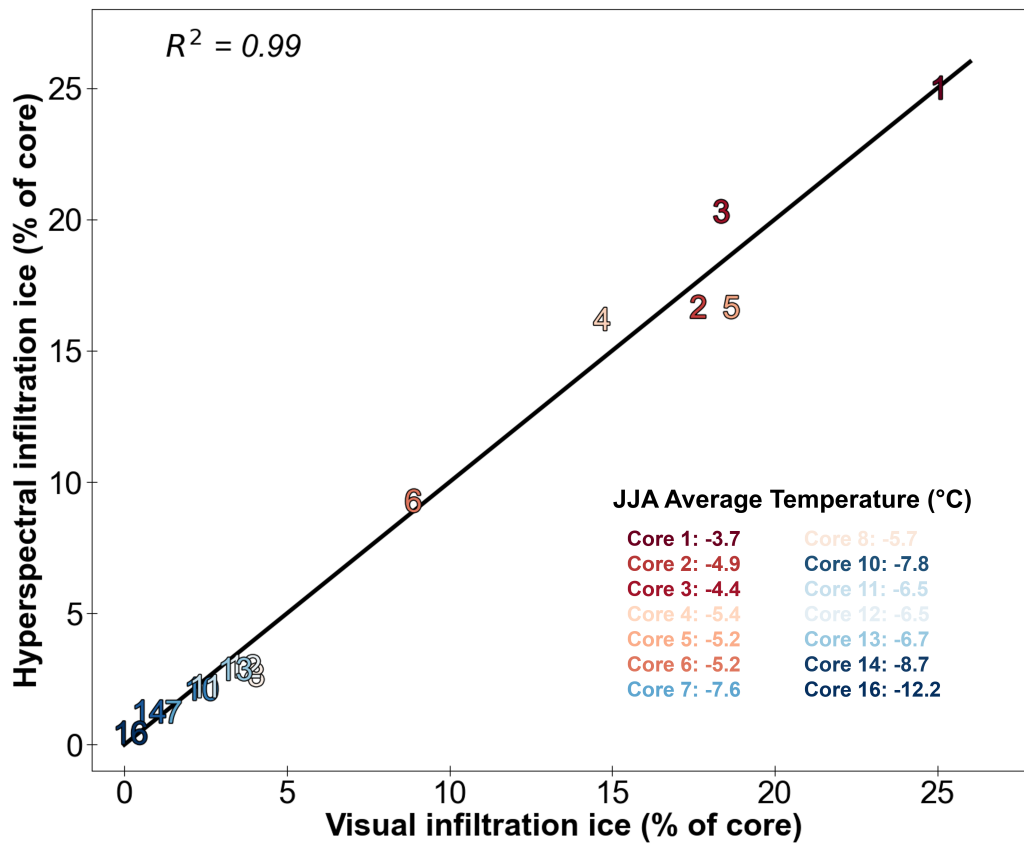
Figure B3. Infiltration ice identified in the NIR-HSI scans compared to visually-identified infiltration ice content in each core. The one-to-one line is shown in black. The core numbers are shaded by summer (JJA) average temperatures estimated by MODIS Land Surface Temperatures.
