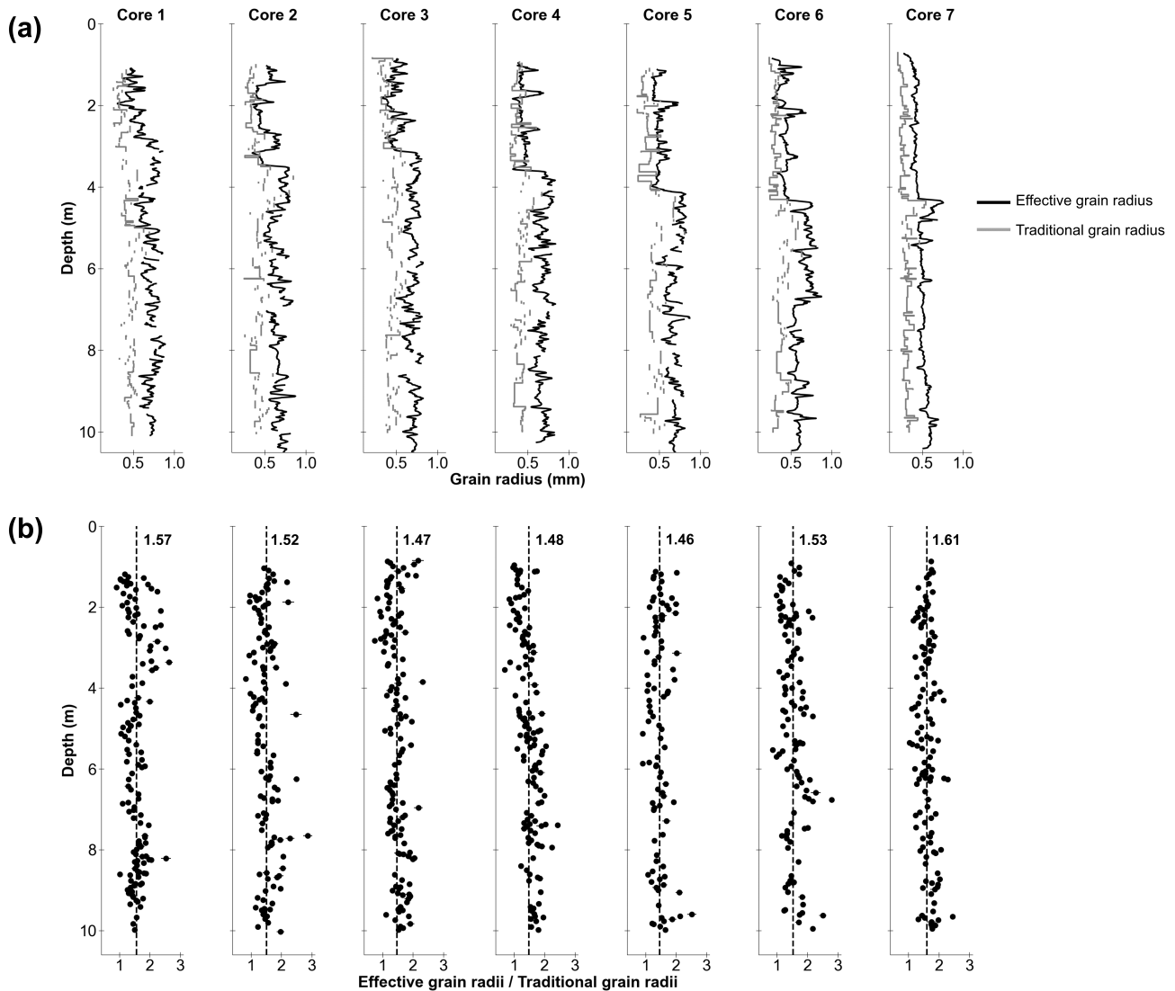
Figure 6. Effective vs. traditional grain sizes. (a) Grain size profiles from digital grain diameter measurements from McDowell et al. (2023) (grey) and from the NIR-HSI (black). (b) Ratios of effective grain sizes to traditional grain sizes. The mean ratios for each core are reported and represented by the dashed black lines.
