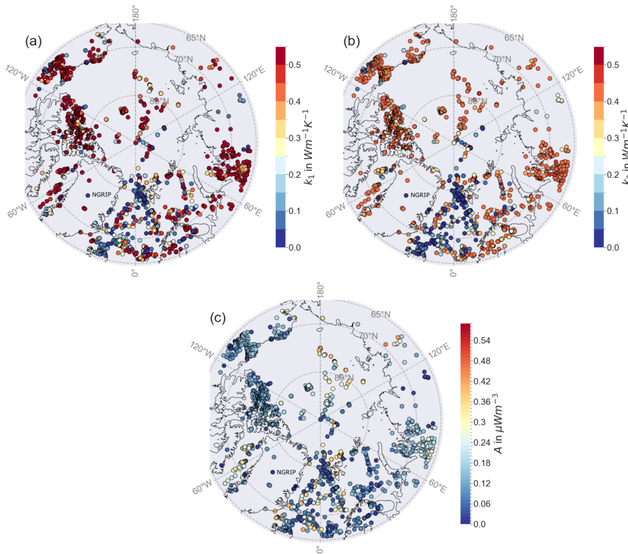
Figure A2. Distribution of the standard deviation of the thermal parameters with q_D calculated with Eq. (3). (a) crustal thermal conductivity k_1 , (b) mantle thermal conductivity k_2 (c) crustal heat production A .
