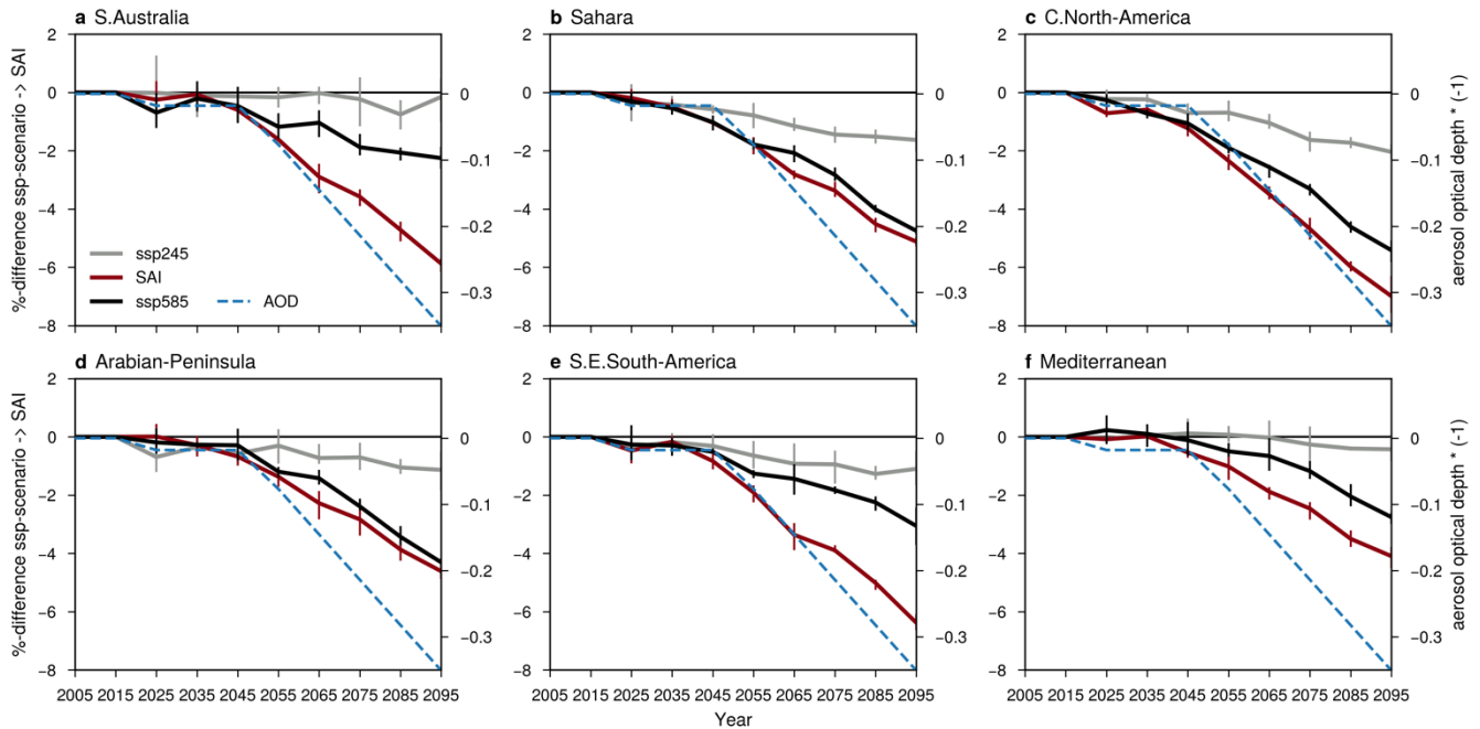
325 Figure 7: Relative difference over time of SAI (red), SSP245 (gray) and SSP585 (black) PV potential compared to 2015-2024 values for selected regions. Lines are the ensemble means with the bars indicating the 20-80 percentile ranges of the single members. X \rightarrow y denotes (y - x)/x .
