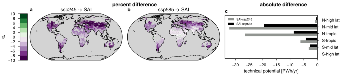
Figure 4: Difference in 2090-2099 PV potential with fixed tilted panels between the ensemble means of SAI and a) SSP245, b) SSP585 and c) absolute difference between latitudinal zonal sums between SAI and SSP245 and SSP585 in PWh/year. White areas have a SNR of < 1 . x \rightarrow y denotes (y - x)/x .
