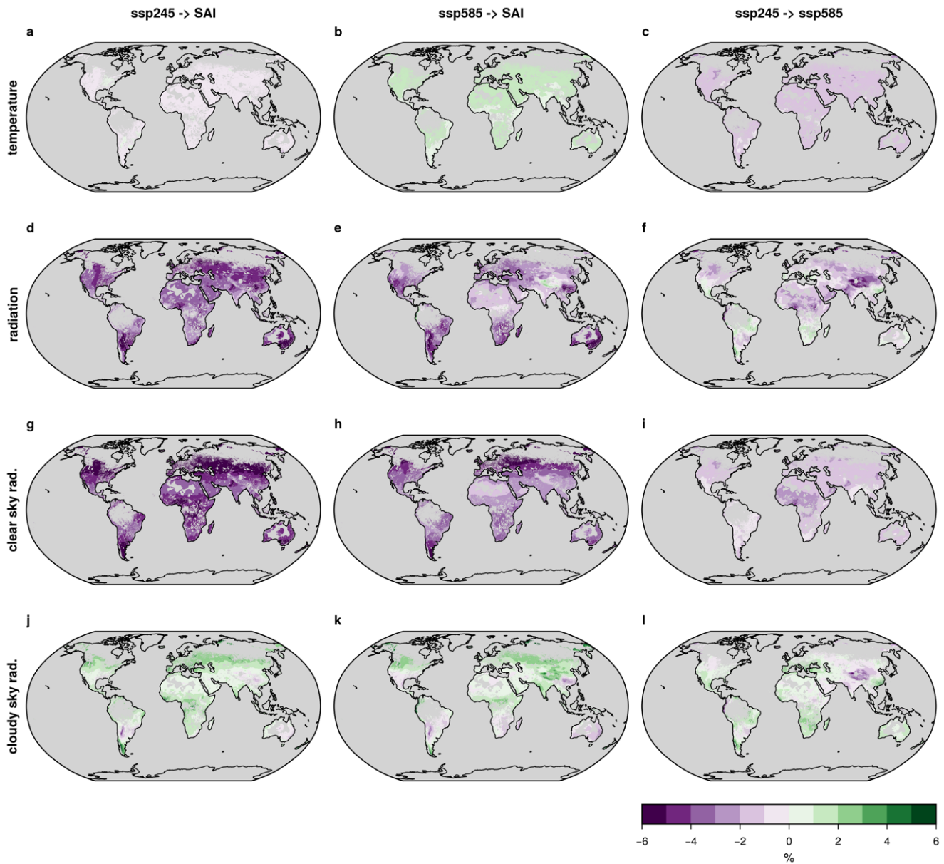
245 Figure 3: Main drivers of change in 2090-2099 PV potential, a-c) surface air temperature, d-f) total downwelling surface radiation, g-i) clear-sky radiation and j-l) cloudy-sky radiation. Areas with SNR < 1 are shown in white. x -> y denotes (y - x)/x . a-c) was calculated by keeping all variables except temperature fixed, d-f) by keeping all variables except radiation fixed, g-i) by using the model output clear sky radiation instead of total radiation (see Methods) and j-l) by subtracting clear sky radiation from total radiation.
