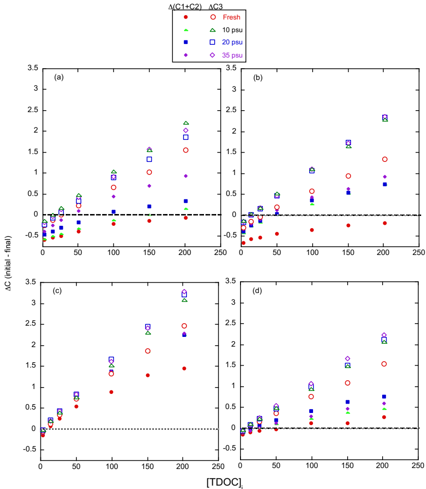
345 Figure 7. Change in EEM components C1-C3 during adsorption-desorption incubations. Plotted is the change in component score, initial – final (i.e. net “adsorption”), for the sum of C1 and C2 (RU, closed symbols) and C3 (RU, open symbols) as a function of initial incubation TDOC ( TDOC_i , mg L -1 ). (a) Kirkpatrick, (b) Taskinas, (c) Jug Bay, and (d) Wachapreague. Red circles, green triangles, blue squares, and purple diamonds reflect 0, 10, 20, and 35 salinity treatments, respectively.
