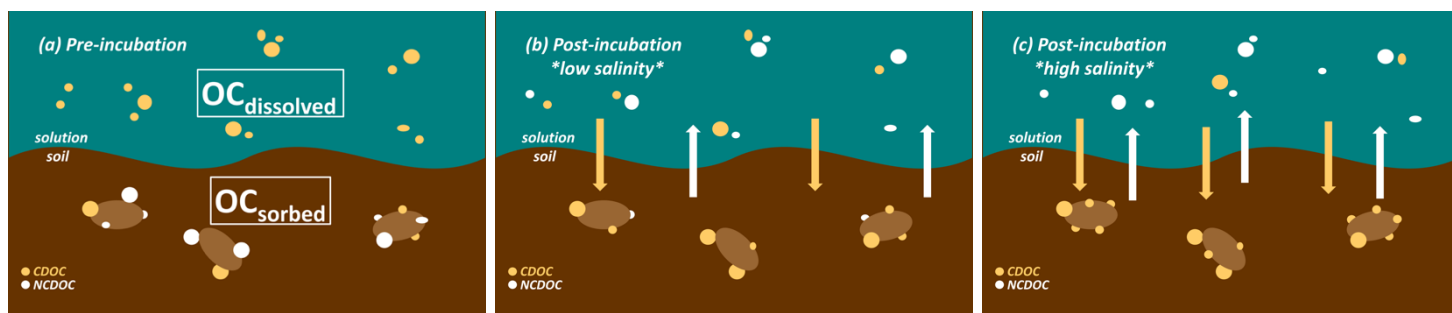
Figure 8. Conceptual diagram of the closed incubation experiments showing (a) pre- vs. (b) & (c) post-incubation exchange of colored (beige dots) vs non-colored (white dots) organic carbon that is either sorbed to soil (bottom brown area) or dissolved (top bluegreen area). The initial composition of the wetland soil sorbed organic carbon ( OC_{\text{sorbed}} ) is a mixture of colored and noncolored OC, whereas the Great Dismal Swamp DOC contains almost exclusively colored OC ( OC_{\text{dissolved}} ). During the incubation at low salinity (b), colored OC is preferentially adsorbed to soil while non-colored OC is desorbed into solution. These net fluxes are intensified at high salinity (c).
