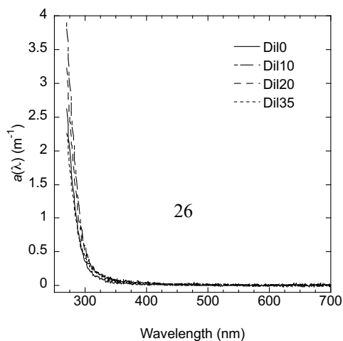
Fig. B1: Average absorbance spectra ( a(\lambda) , m -1 ) of dilutant used to create different standards from the Great Dismal Swamp
