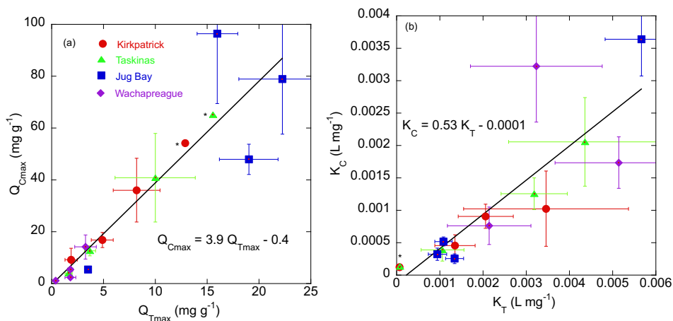
280 Figure 6. Comparison of maximum sorption capacity (a) and binding affinity (b) estimated for CDOC isotherms ( Q_{Cmax} , K_C ) vs those for the TDOC isotherms ( Q_{Tmax} , K_T ) fit with initial mass Langmuir isotherms (the latter in Appendix B Table B2). Error bars indicate standard errors of the parameter estimates from non-linear regression. Red circles, green triangles, blue squares, and purple diamonds denote Kirkpatrick, Taskinas, Jug Bay, Wachapreague, respectively. Points marked with asterisks are the Kirkpatrick and Taskinas 35 incubations, which were estimated by extrapolation and lack error bars.
