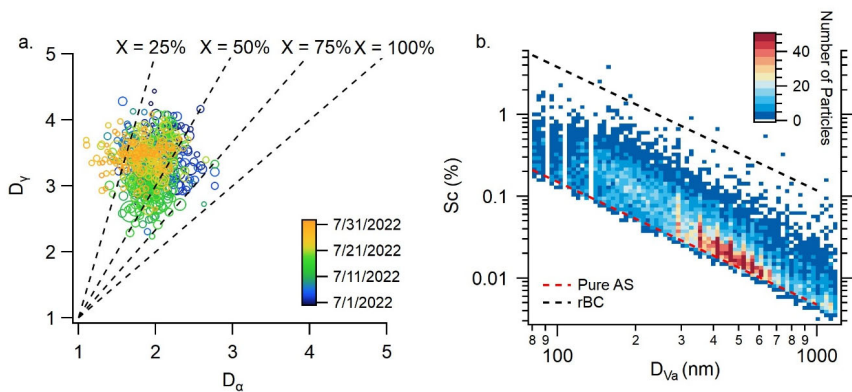
560 Figure 7: (a) Mixing state diagram depicting the relationship between bulk particle diversity ( D_T ), average single particle diversity ( D_a ). The dashed lines indicate the resulting mixing state index ( \chi ). Points are sized by PM_{1,rBC} concentration and colored by sampling date. (b) Bivariate histogram of estimated particle critical supersaturation and particle diameter. Dashed lines represent uncoated rBC ( \kappa = 0.001 ) and pure ammonium sulfate ( \kappa = 0.61 ).
