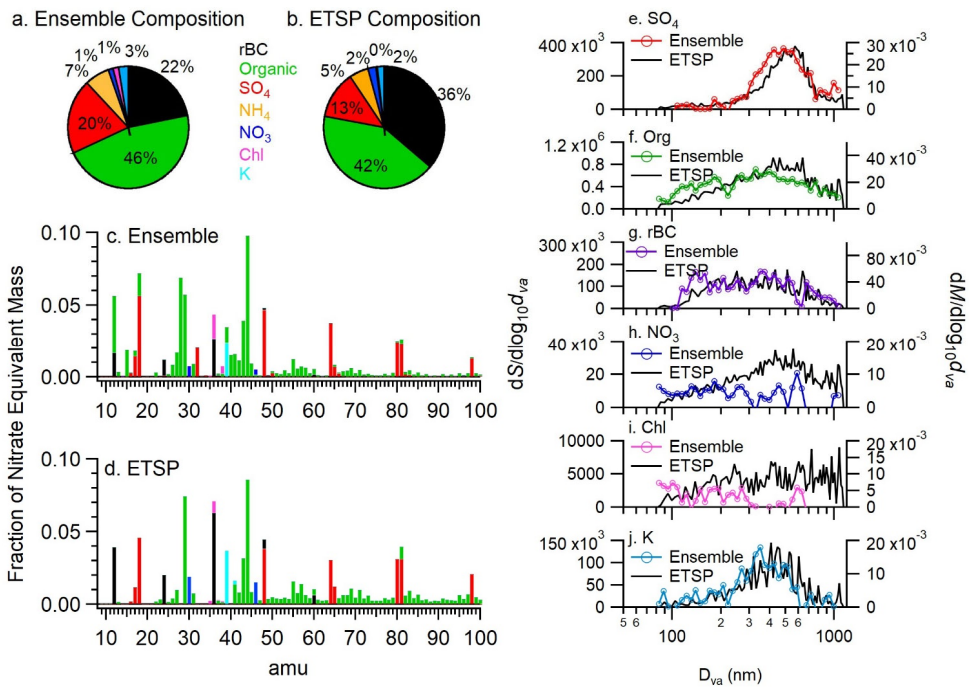
540 Figure 3: Average fractional composition of total PM 1,BC measured by (a) high-resolution ensemble measurements and (b) ETSP measurements. (c) Average mass spectrum of ensemble measurements and (d) average mass spectrum of all single particle events measured by ETSP mode. (e-j) Comparison of species dependent size distributions for ensemble measurements (colored line) and ETSP measurements (black line). Bulk size distributions are mass weighted (against right y axes), while ETSP measurements are signal weighted (against left y axes).
