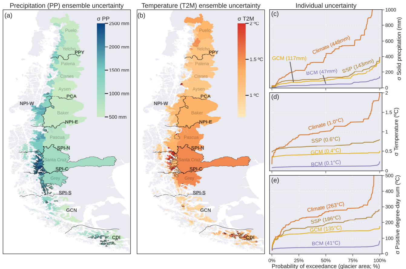
395 Figure 7. Future climate uncertainty (standard deviation; \sigma ) in mean annual precipitation (a) and temperature (b) obtained from the complete ensemble (2070–2099). The catchments with a coefficient of variation greater than 40% have black outlines. Means were calculated using only the glacierized grid cells of each catchment. The grey names in (a) and (b) correspond to the names of the main catchments, while the solid black line indicates the division between the hydrological zones defined in Fig. 1. Individual uncertainty (in terms of glacier area) in solid precipitation (c), temperature (d) and positive degree-day sum (e) across different reference climates, emission scenarios (SSPs), general circulation models (GCMs) and bias correction methods (BCM). The values in parenthesis indicate the glacier area weighted means. 400
