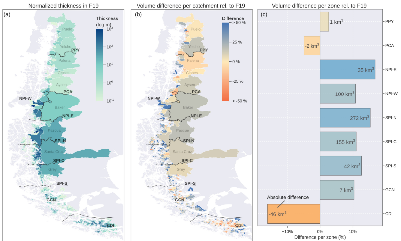
345 Figure 4. Volume comparison between Millan et al. (2022) (M22) and Farinotti et al. (2019) (F19) based on RGI6. a) Thickness normalized by the catchment area from F19 (in log scale). Percentage difference between M22 and F19 per b) catchment and c) hydrological zone considering F19 as reference. The grey names in (a) and (b) correspond to the names of the main catchments, while the solid black line corresponds to the division between the hydrological zones defined in Fig. 1. The text in c) indicates the absolute difference in volume (M22 - F19).
