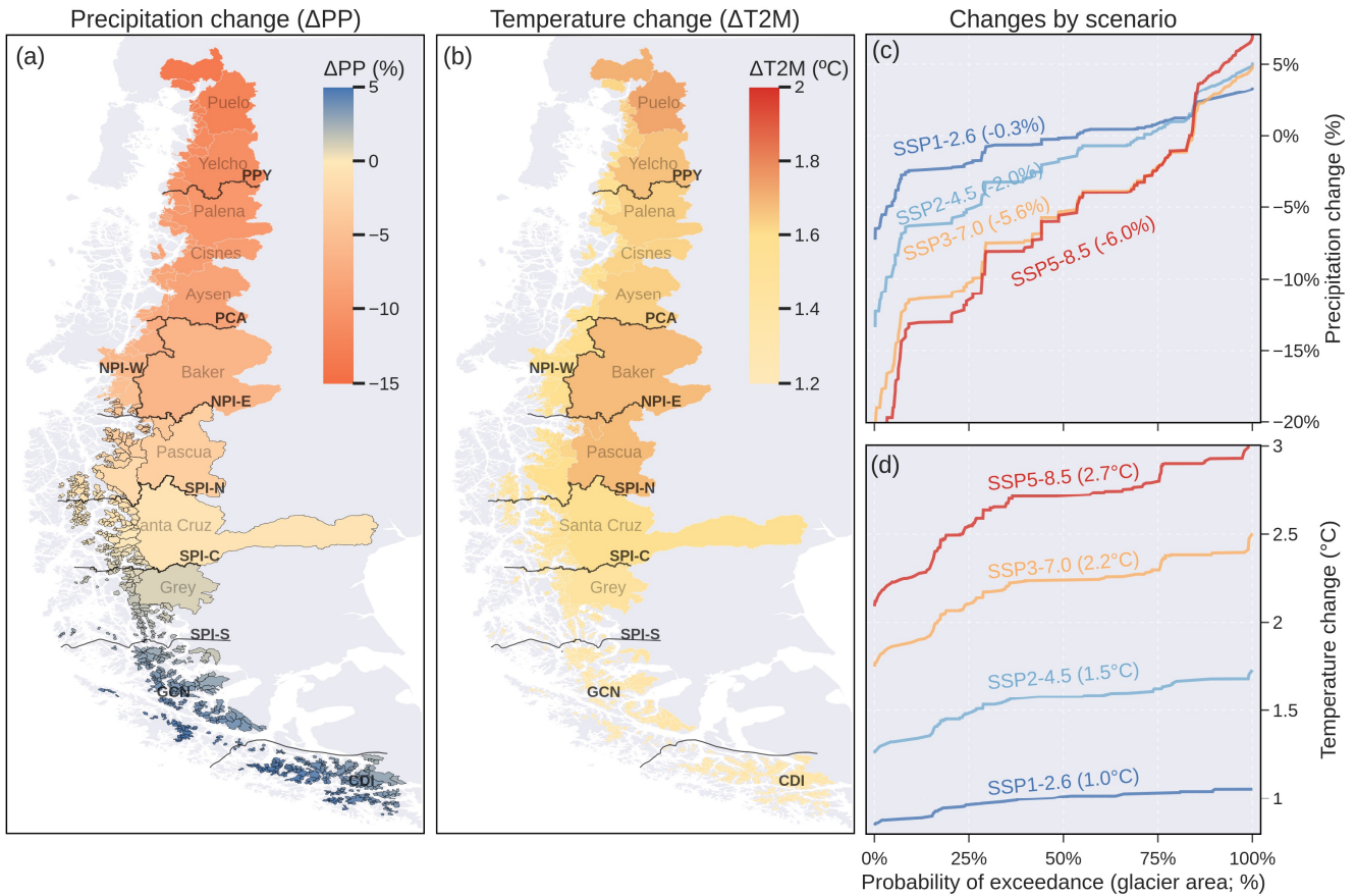
375 Figure 6. Multi-model means ( n = 10 ) of future precipitation (a) and temperature change (b) considering the SSP 2-4.5 scenario (1980–2015 vs. 2070–2099). Means were calculated using only the glacierized grid cells of each catchment. The catchments with black outlines indicate low model agreement, where less than 80% of the models agree on the sign of the change. The grey names in (a) and (b) correspond to the names of the main catchments, while the solid black line indicates the division between the hydrological zones defined in Fig. 1. Differences by scenario for precipitation (c) and temperature (d). The values in parenthesis indicate the glacier area weighted means. 380
