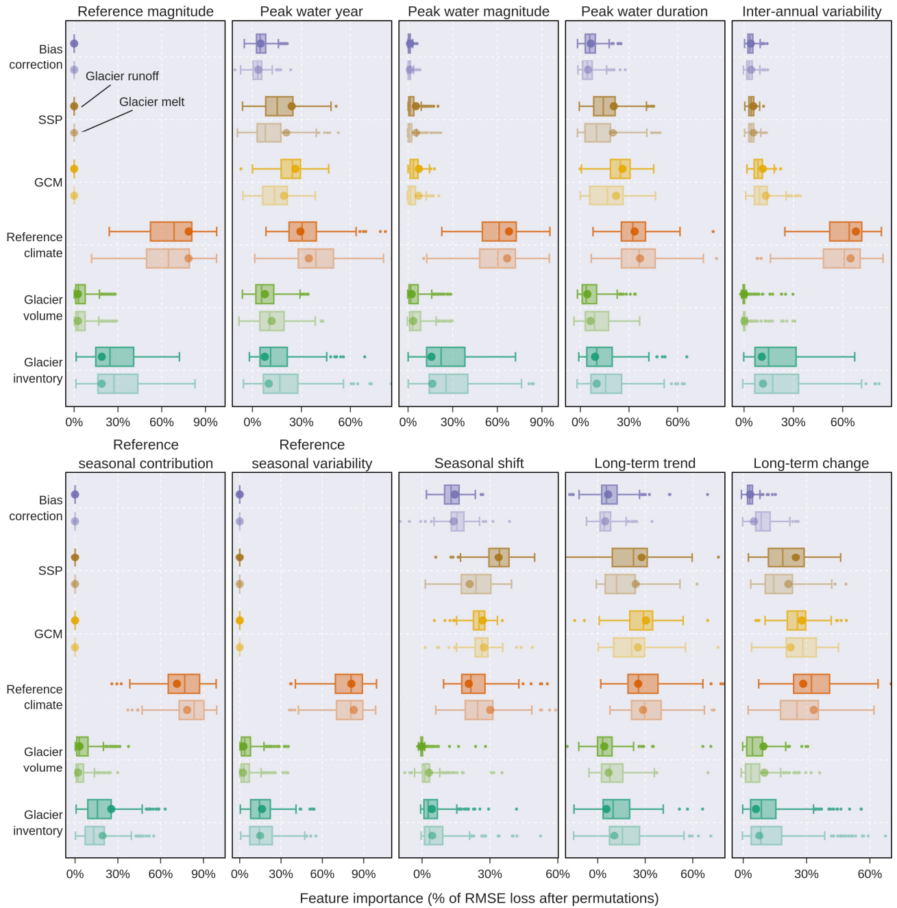
465 Figure 10. Importance of each source of uncertainty for the glacio-hydrological signatures obtained from the glacier runoff (dark colours) and melt (light colours). The importance of each source on the glacio-hydrological signatures (Table 2) is represented as the percentage of the average change in the Root Mean Square Error (RMSE), with high values indicating a greater importance. The circles correspond to the glacier area weighted means. Note that each panel has a different range.
