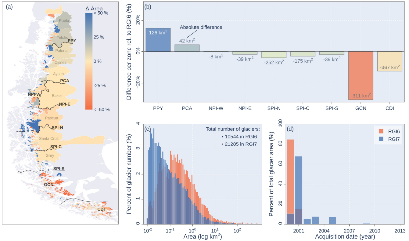
330 Figure 3. Comparison between Randolph Glacier Inventory (RGI) versions 6 and 7. Difference in area a) per catchment and b) per hydrological zone considering RGI6 as reference. The names in grey in (a) correspond to the names of the main catchments, while the solid black line corresponds to the division between the hydrological zones defined in Fig. 1. The text in b) indicates the absolute difference in area (RGI7 – RGI6). c) Distribution of glacier area. d) Percent of glacier area per year of acquisition.
