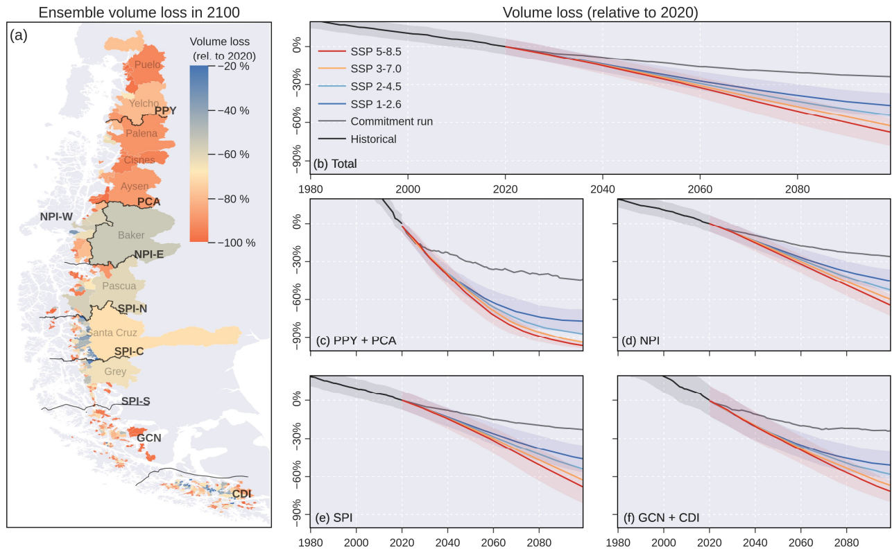
Figure 8. Glacier volume loss relative to 2020. a) Mean volume loss in 2100 derived from the full ensemble ( n = 1920 ). Volume loss for the sum of all catchments (b), the northern area including PPY and PCA (c), the Northern Patagonian Icefield (d), the Southern Patagonian Icefield (e) and the southern area including GCN and CDI (f). The solid line represents the mean for each scenario, while the uncertainty bands represent \pm one standard deviation (shown only for historical, SSP 1-2.6 and SSP 5-8.5 for visualization purposes). Volume, area and specific mass balance by hydrological zone are shown in Fig. S1. The commitment run considers a pseudo-random climate based on the period 1985–2015.
