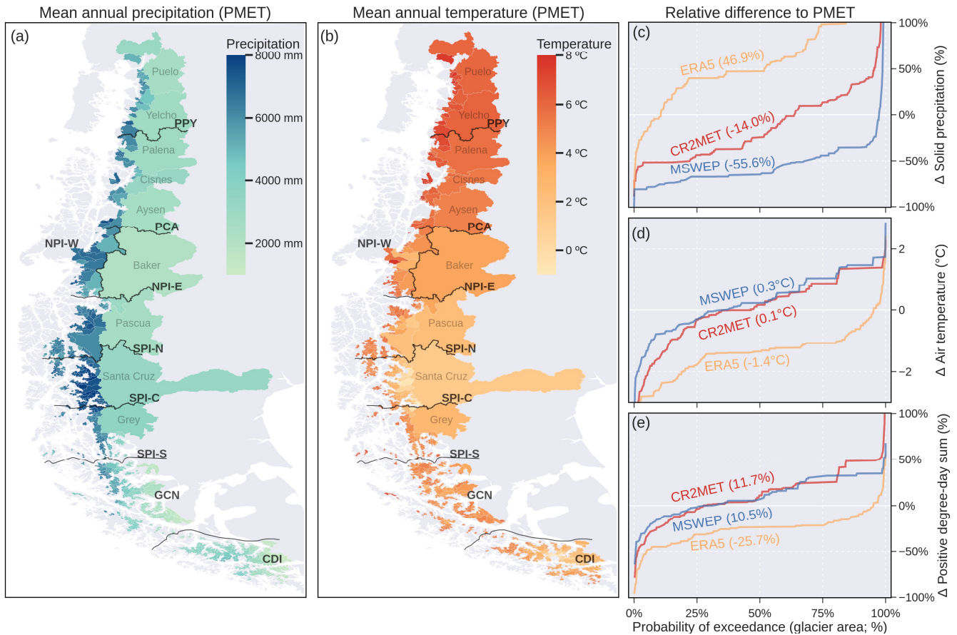
360 Figure 5. Historical reference climate in terms of annual precipitation (a) and temperature (b) according to the PMET dataset. Long- term averages (1980-2015) were calculated using only the glacierized grid cells of each catchment. The grey names in (a) and (b) correspond to the names of the main catchments, while the solid black line corresponds to the division between the hydrological zones defined in Fig. 1. Differences between PMET and CR2MET, ERA5 and MSWEP/MSWX sorted by glacier area for solid 365 precipitation (c), temperature (d), and positive degree-day sum (e). The values in parenthesis indicate the glacier area weighted means.
