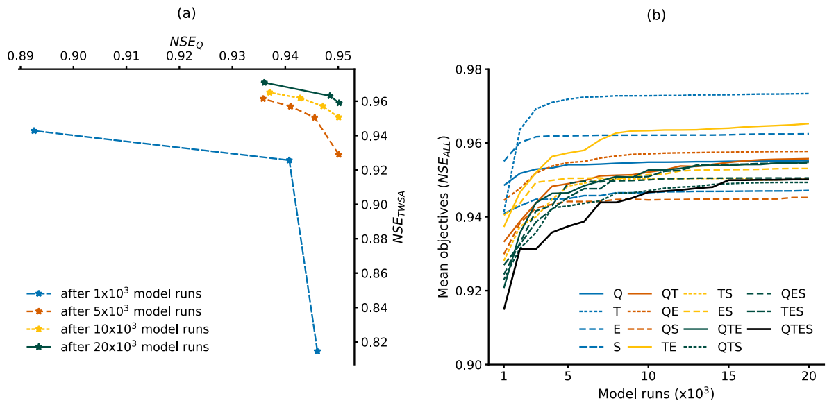
Figure 3. Convergence of single and multi-objective calibrations of the Brahmaputra basin. (a) Pareto fronts of a 2-objective calibration experiment (Experiment-QT with objectives NSE_Q and NSE_{TWSA} ) after one, five, ten, and twenty thousand model evaluations. (b) the mean objective value ( NSE ) of the compromise solution of all calibration experiments as a function of no. of model evaluations. The Pareto fronts and the compromise solutions have been determined after merging all solutions in all replications.
