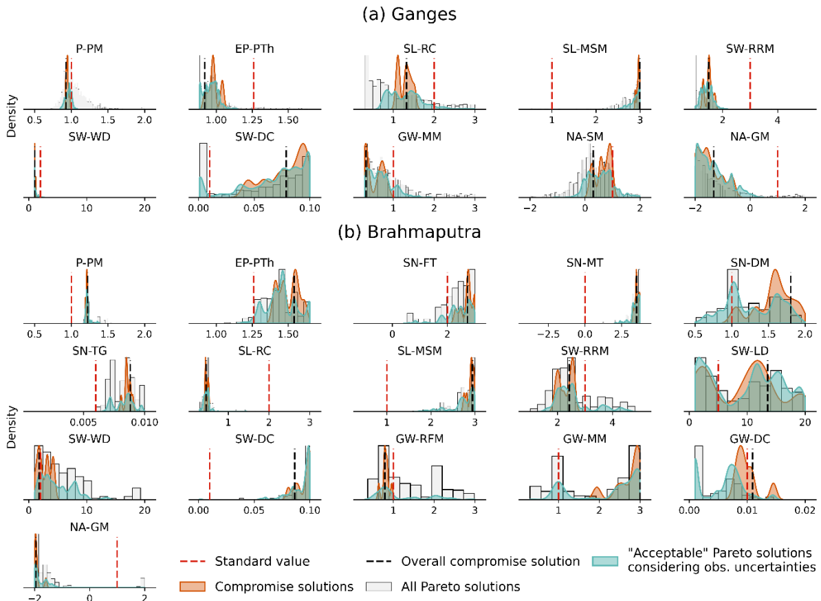
Figure 7: The distribution of parameters of the compromise solutions in the 8 repeated 4-objective calibration experiments (greendarkorange), and the “acceptable” Pareto solutions considering observation uncertainties (orangecyan), and all Pareto solutions in all replications (grey). The overall compromise solution (red-black dashed vertical line) represents the compromise solution among all solutions in all replications. The parameter value of the standard WGHM is shown with the black-red dashed vertical line.
