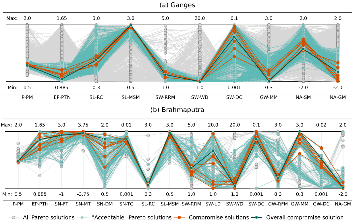
Figure 8: Parallel coordinate plot of all Pareto solutions (grey), the compromise parameter sets (N=8, black-dashed darkorange ), the overall compromise solution ( black solid cyan ), and the set of “acceptable Pareto solutions considering observation uncertainty” ( Greendark green ) of the 4-objective calibration in the Ganges basin (a) and the Brahmaputra (b) basin
