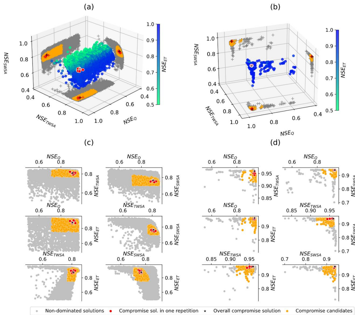
Figure 5: The Pareto front of 4-objective calibration experiments of the Ganges basin and for both the Brahmaputra basin. The 3-D view of the 4-D PF of Ganges (a) and Brahmaputra (b), while the 4 th dimension is colour coded. Only solutions having NSE greater than 0.5 are shown. The 2-D projection is shown with crosses. The bottom row shows the 2-D view of each pair of objectives for the Ganges (c) and the Brahmaputra (d) basin. All non-dominated solutions are shown in grey, the compromise solution of each replication in red, the overall compromise solution in black, and the candidate compromise solutions in orange.
