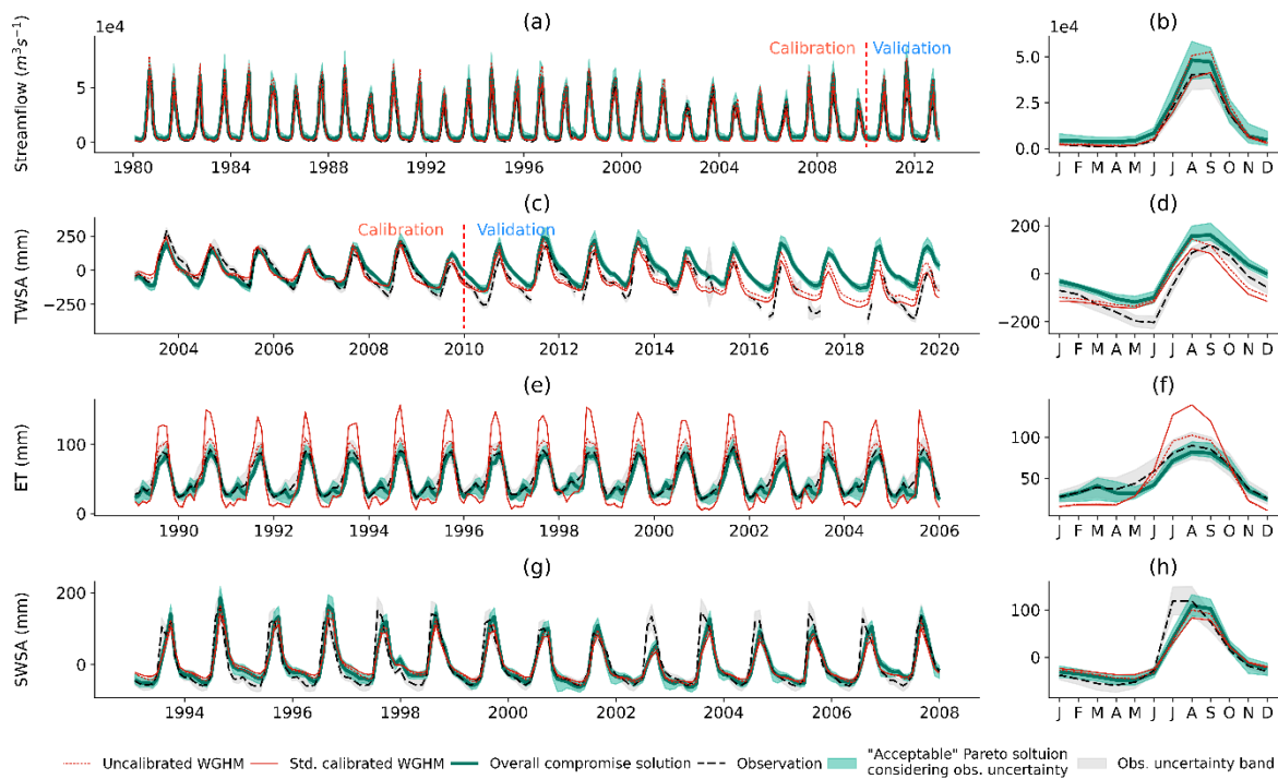
1655 Figure 9: Simulations of streamflow (a, b), TWSA (c, d), ET (e, f), and SWSA (g, h) in the 1660 Ganges basin with the overall compromise solution of the 4-objective calibration. The simulation results with the acceptable Pareto solutions considering observation uncertainties (green dark green), with uncalibrated WGHM (red dotted line), and with the calibrated model with standard approach (dashed grey red solid) are also shown; monthly time series (a, c, e, g) and monthly mean values (b, d, f, h). The mean was computed over the entire period with available observations.
