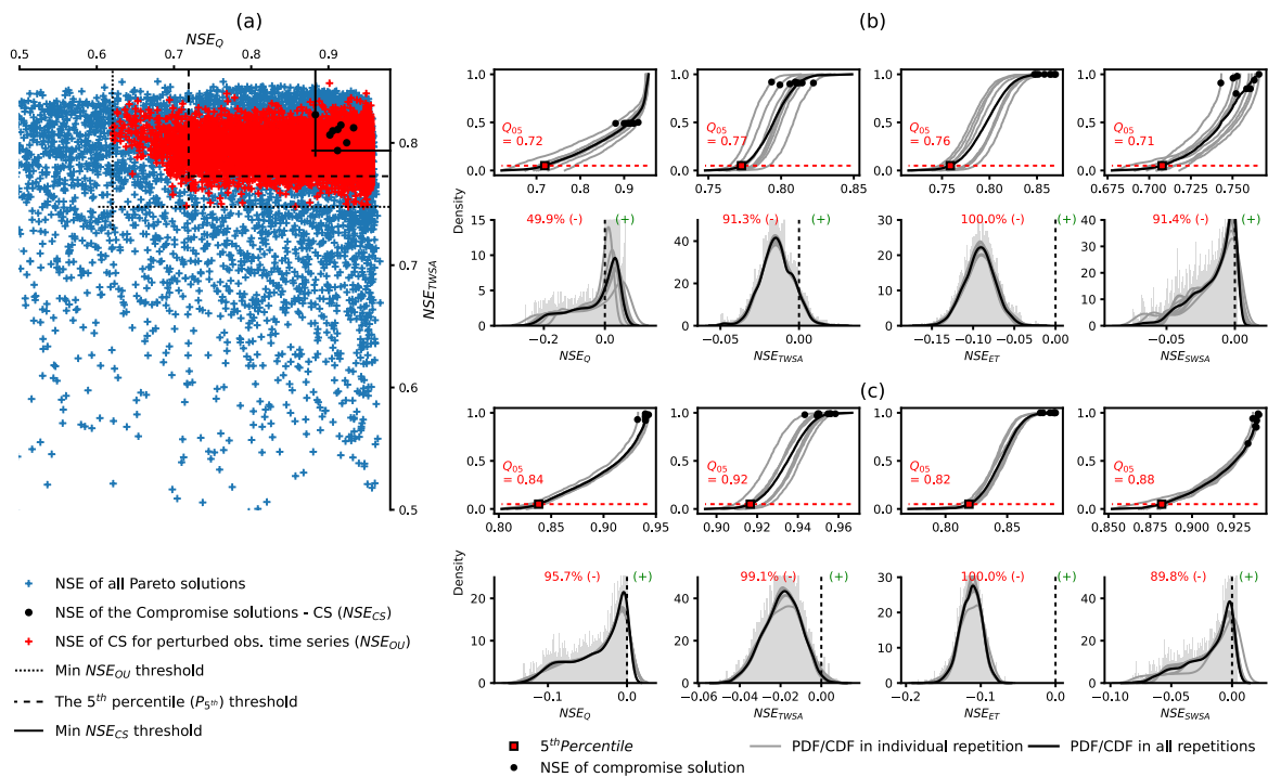
Figure 6: Uncertainty in NSE of the compromise solutions (CS) in the repeated experiments of 4-objective calibration, obtained by propagation of observational uncertainties into objectives. (a) Scatter plot of objective values (NSE) of (i) all Pareto solutions, (ii) the compromise solutions ( NSE_{CS} ) and (iii) the compromise solutions computed for 1000 perturbed observation time series ( NSE_{OU} ) for the Ganges basin. Three thresholds (M2, M3, M4) are visualized as options to delineate the space of compromise solutions under consideration of observational uncertainties (see text for details). Density functions (CDFs and PDFs) of NSE_{OU} in the Ganges basin (b) and in the Brahmaputra basin (c). PDFs represent the deviations NSE_{OU} - NSE_{CS} . The black dashed vertical lines in the density plots delineate the zones of NSE decrease and NSE increase. Densities of NSE_{OU} for each compromise solution of a single repetition are plotted in grey and the density function of NSE_{OU} of all compromise solutions are in black. The black dots show the objective values of the compromise solutions.
