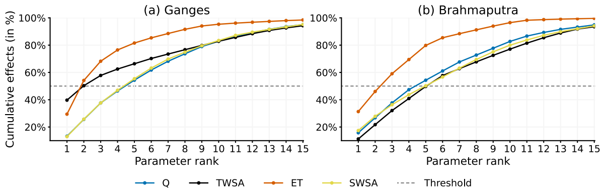
625 Figure 2. Cumulative effect in percent of the “total effect” (sum of all effects of all parameters) of top-ranked parameters up to different cut-off ranks. The function of the cumulative effect and the cut-off level differ among the four response variables Q, TWSA, ET, and SWSA in the two basins – Ganges (a) and Brahmaputra (b). Sensitivity to parameters in this example was for the monthly time-series (MTS) of the four target response variables. The grey line indicates the cut-off threshold at 50% of the “total effect” that must be surpassed by the top-ranked parameters for each variable and for each signature. For example, the cumulative effect of the three highest-ranked parameters on TWSA in the Ganges basin accounts for 58% of the total combined effects of all parameters on this variable, while the cumulative effect of the top three parameters on Q is only 38% of the total combined effects of all parameters in the basin. 630 635
