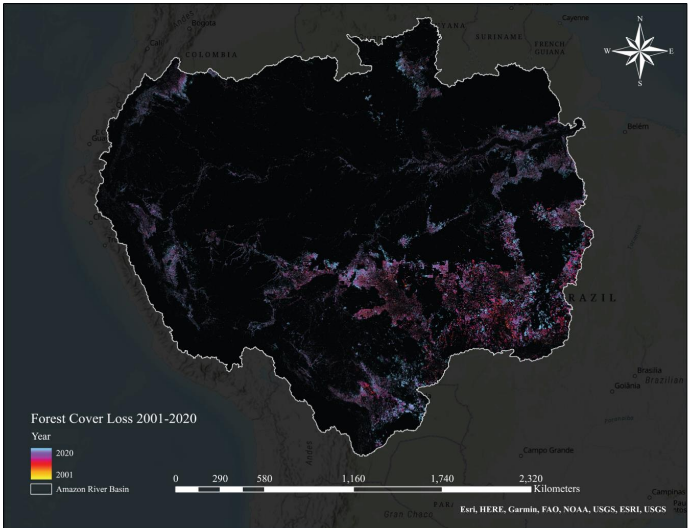
Figure 2. Forest Cover Loss in the Amazon River Basin 2001-2020. Forest loss data was acquired from the Global Forest Change Dataset (Hansen et al., 2013).
