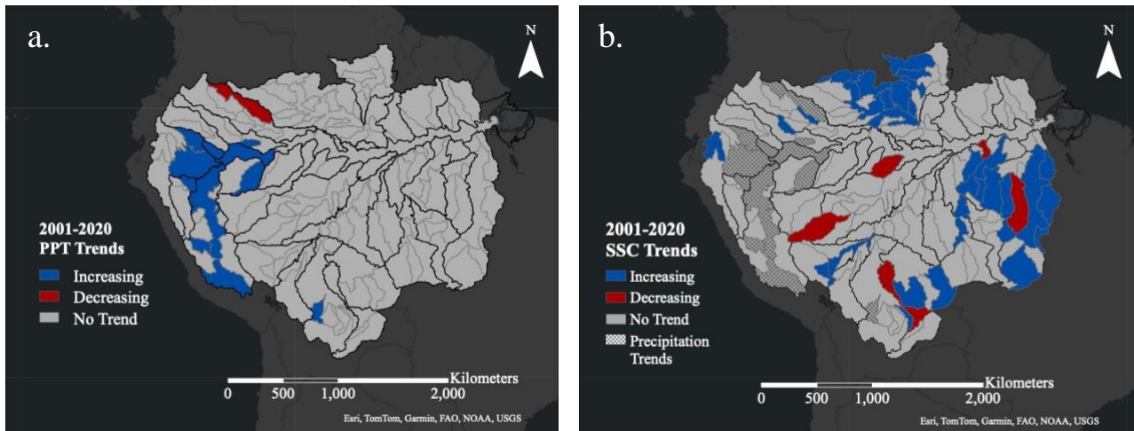
325 Figure 5. Precipitation (a) and Sediment (b) Trends across the Amazon River Basin, 2001-2020.
