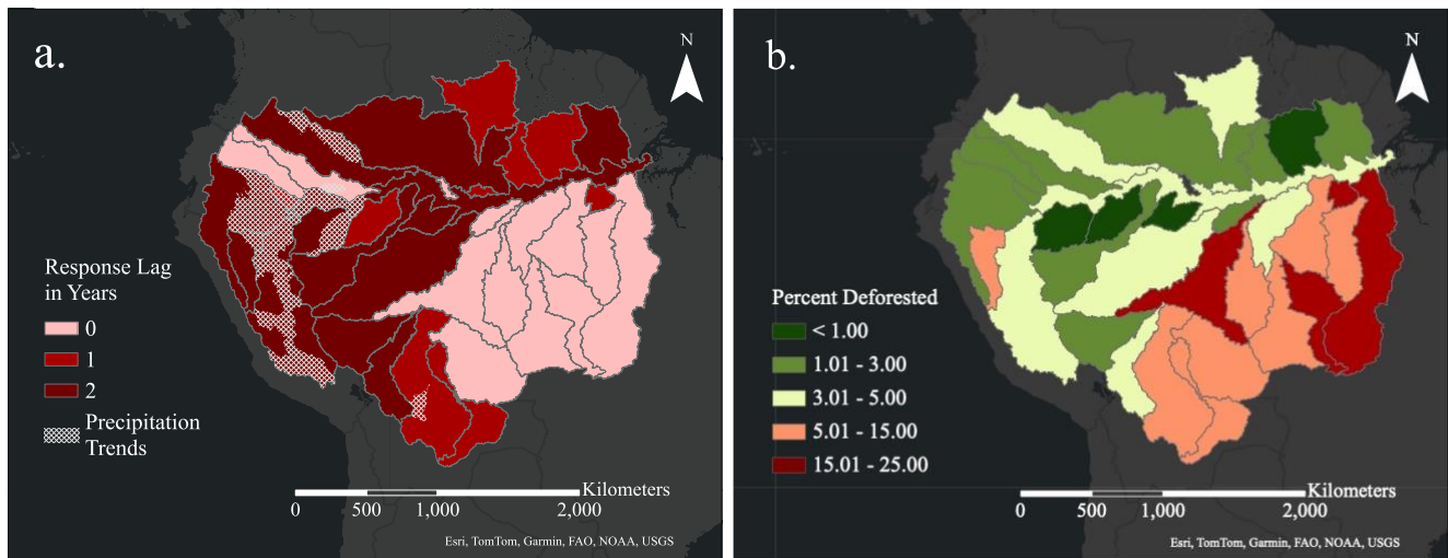
350 Figure 7. Identified lag response (in years) present in each major tributary basin (a) and total percentage of each major tributary basin deforested in the Amazon from 2001-2020 (b). River reaches falling within the precipitation zone (sig. precipitation trends) were excluded from the basin lag analysis.
