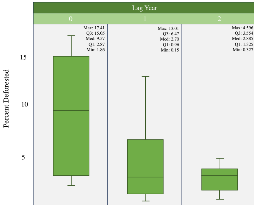
390 Figure 8. Percent of each basin deforested by lag year. Two outlier basins, the Curuá-una and the Huallaga basins, were removed from L1 (Curuá-una, 23%) and L2 (Huallaga, 10%).
