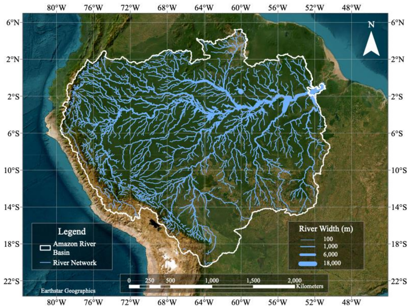
Figure 1: The Amazon River Basin with major streams and rivers. Line width symbolizes river's width. Data used to produce river reach delineations are from the Surface Water Ocean Topography (SWOT) River Database (SWORD) centerlines (Altenau et al., 2021)
