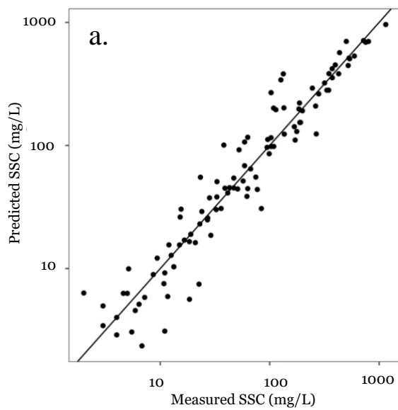
205 Figure 4. (a) Validation plot of remote sensing derived (predicted) suspended sediment concentration (SSC; mg/L) vs. in situ SSC measurements (MAE = 32 mg/L; Relative Error = 0.21; Percent Bias = 11%; RMSE = 58.7 mg/L) and (b) Number of annually averaged SSC observations during the 2001-2020 period.
