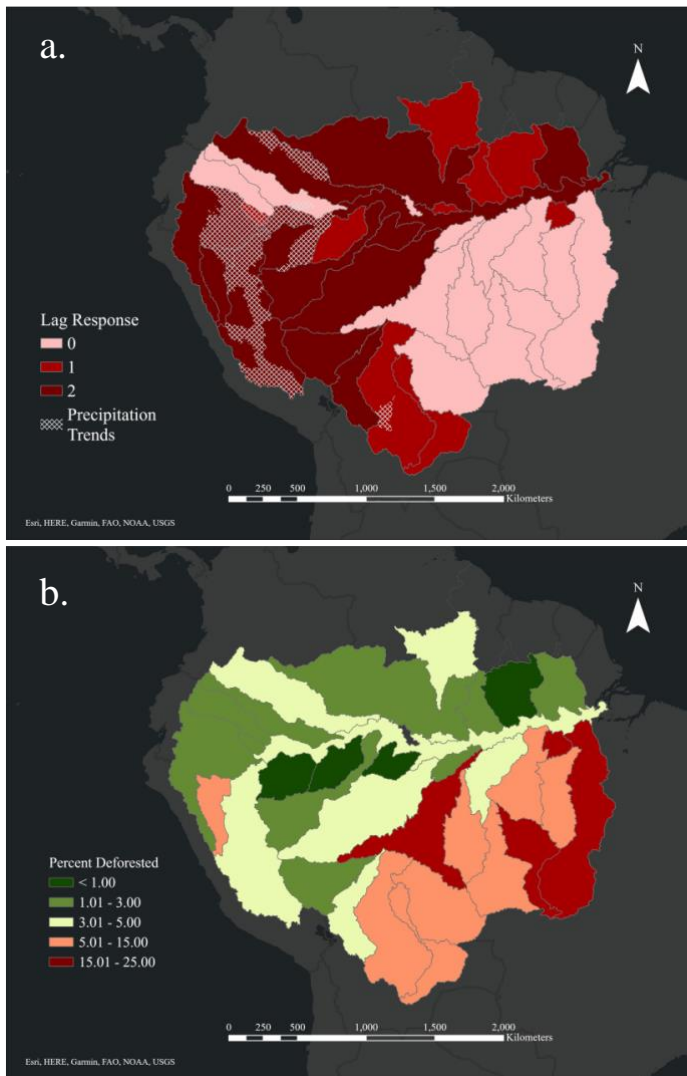
Figure 7. Identified lag response (in years) present in each major tributary basin (a) and total percentage of each major tributary basin deforested in the Amazon from 2001-2020 (b). River reaches falling within the precipitation zone (sig. precipitation trends) were excluded from the basin lag analysis.
