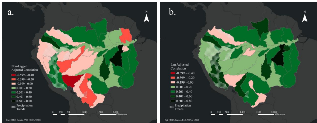
335 Figure 6. Correlation Coefficients prior to applying lags (a) and Correlation Coefficients after applying lags (b)
