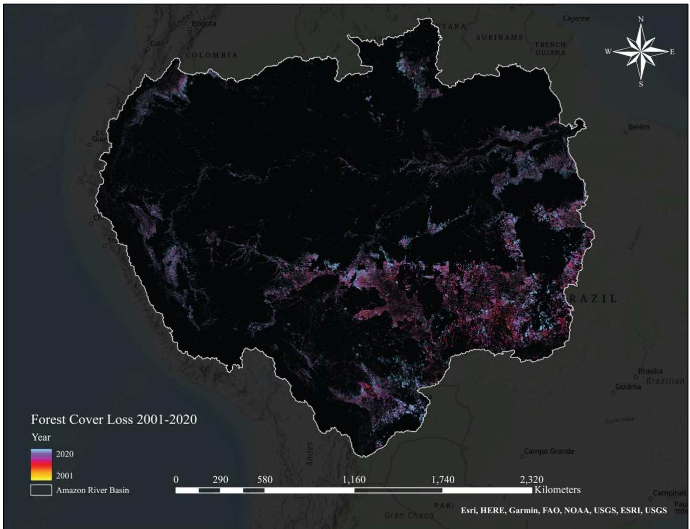
155 Figure 2. Forest Cover Loss in the Amazon River Basin 2001-2020. Forest loss data was acquired from the Global Forest Change Dataset (Hansen et al., 2013).
