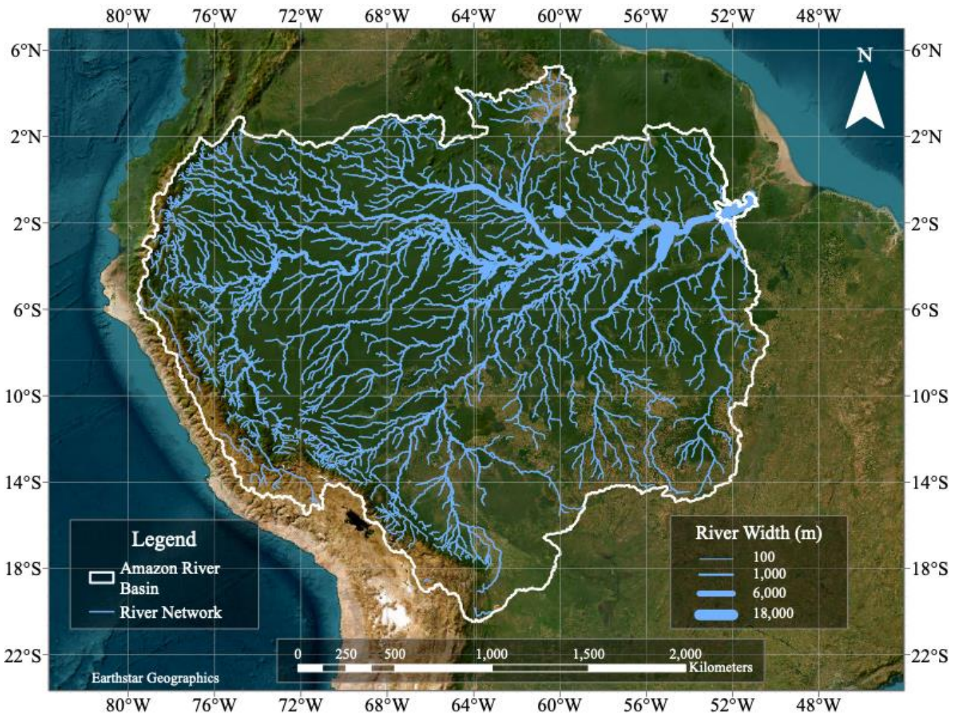
125 Figure 1: The Amazon River Basin with major streams and rivers. Line width symbolizes river's width. Data used to produce river reach delineations are from the Surface Water Ocean Topography (SWOT) River Database (SWORD) centerlines (Altenau et al., 2021)
